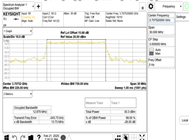
Band77-Part27_15MHz_DFT_s_OFDM_SCS30kHz_BPSK_RB36_0_CH647168
