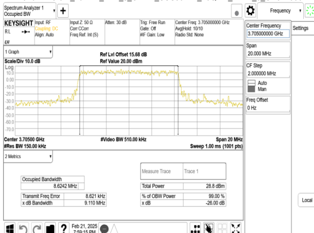
Band77-Part27_10MHz_DFT_s_OFDM_SCS30kHz_16QAM_RB24_0_CH647000
