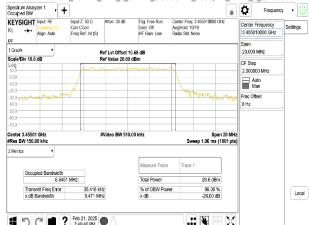
Band77-Part27_10MHz_DFT_s_OFDM_SCS30kHz_256QAM_RB24_0_CH630334
