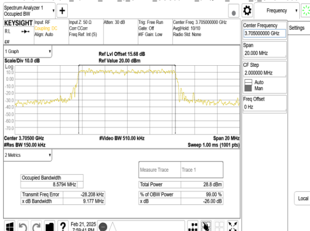
Band77-Part27_10MHz_DFT_s_OFDM_SCS30kHz_64QAM_RB24_0_CH647000
