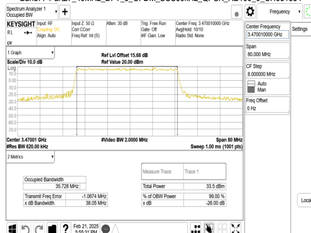
Band77-Part27_40MHz_DFT_s_OFDM_SCS30kHz_QPSK_RB100_0_CH631334
