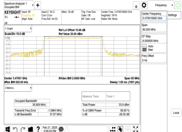
Band77-Part27_40MHz_DFT_s_OFDM_SCS30kHz_BPSK_RB100_0_CH631334
