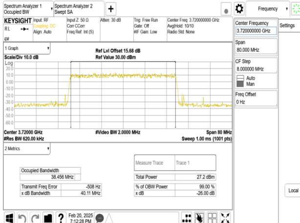
Band77-Part27_40MHz_DFT_s_OFDM_SCS15kHz_256QAM_RB216_0_CH648000
