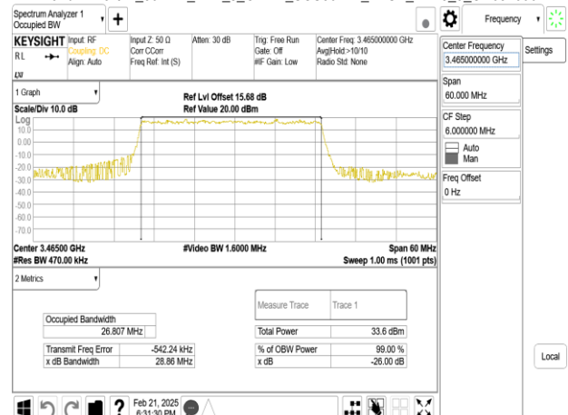
Band77-Part27_30MHz_DFT_s_OFDM_SCS30kHz_BPSK_RB75_0_CH631000
