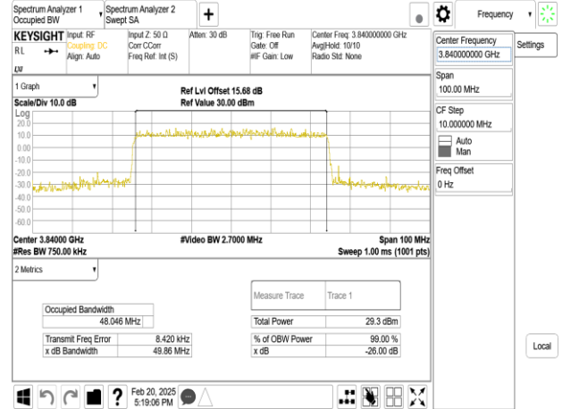
Band77-Part27_50MHz_DFT_s_OFDM_SCS15kHz_QPSK_RB270_0_CH663666
