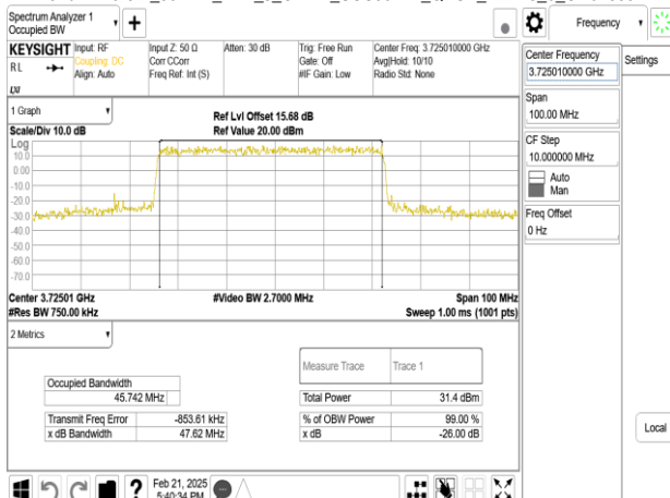
Band77-Part27_50MHz_DFT_s_OFDM_SCS30kHz_QPSK_RB128_0_CH648334
