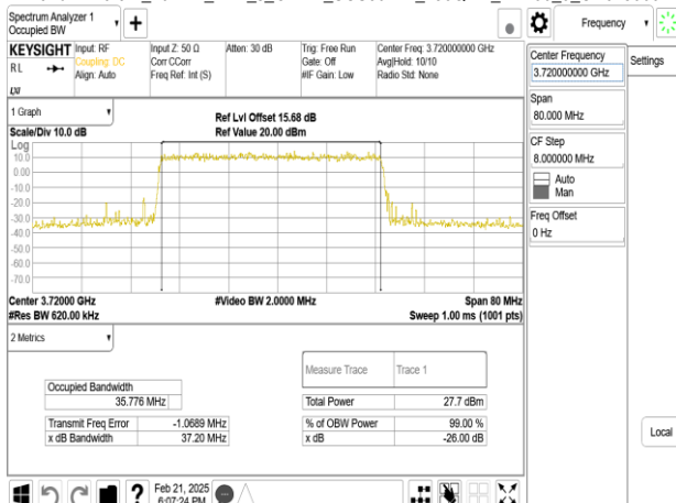
Band77-Part27_40MHz_DFT_s_OFDM_SCS30kHz_256QAM_RB100_0_CH648000
