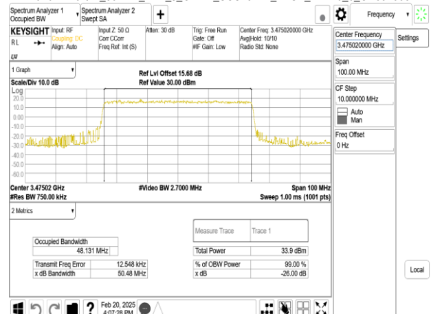
Band77-Part27_50MHz_DFT_s_OFDM_SCS15kHz_BPSK_RB270_0_CH631668
