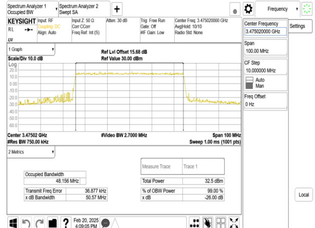
Band77-Part27_50MHz_DFT_s_OFDM_SCS15kHz_16QAM_RB270_0_CH631668
