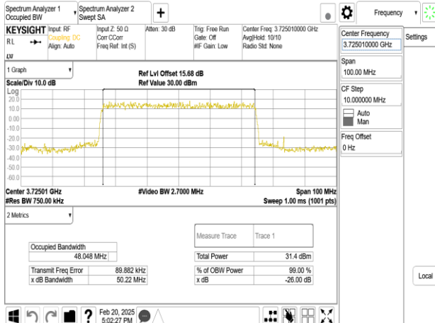
Band77-Part27_50MHz_DFT_s_OFDM_SCS15kHz_BPSK_RB270_0_CH648334
