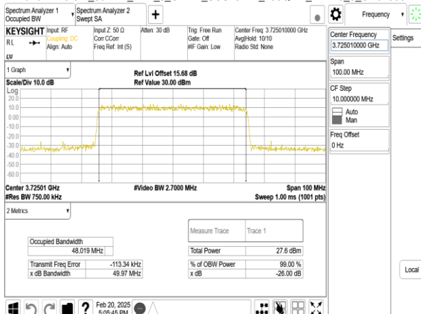
Band77-Part27_50MHz_DFT_s_OFDM_SCS15kHz_256QAM_RB270_0_CH648334
