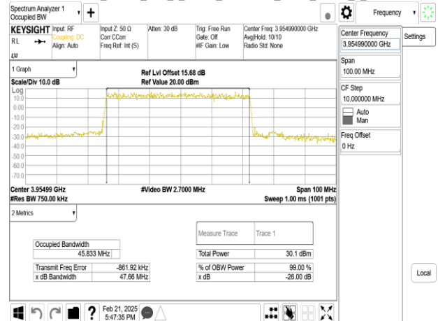
Band77-Part27_50MHz_DFT_s_OFDM_SCS30kHz_16QAM_RB128_0_CH631668
