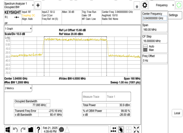
Band77-Part27_80MHz_DFT_s_OFDM_SCS30kHz_QPSK_RB216_0_CH662666
