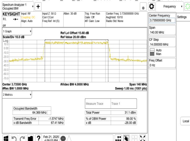
Band77-Part27_70MHz_DFT_s_OFDM_SCS30kHz_QPSK_RB180_0_CH649000
