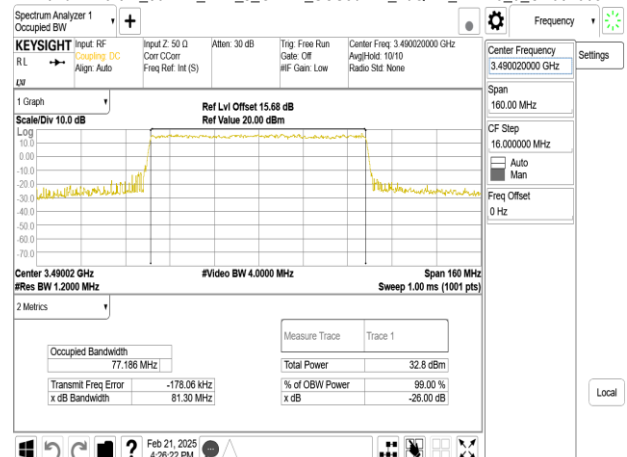
Band77-Part27_80MHz_DFT_s_OFDM_SCS30kHz_16QAM_RB216_0_CH632668
