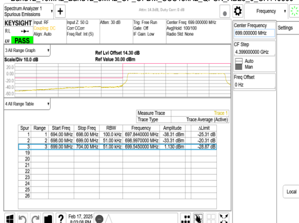
Band12_10MHz_Band12_5MHz_CP_OFDM_SCS15kHz_QPSK_RB25_0_CH140300
