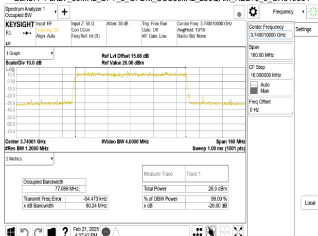
Band77-Part27_80MHz_DFT_s_OFDM_SCS30kHz_256QAM_RB216_0_CH649334
