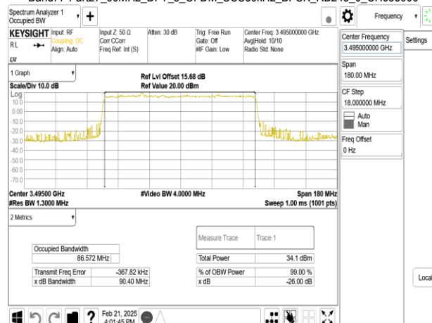
Band77-Part27_90MHz_DFT_s_OFDM_SCS30kHz_BPSK_RB243_0_CH633000
