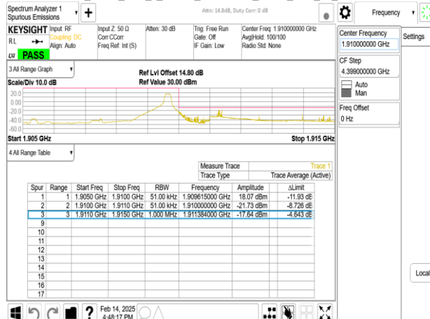
Band2_5MHz_DFT_s_OFDM_SCS15kHz_BPSK_RB25_0_CH381500
