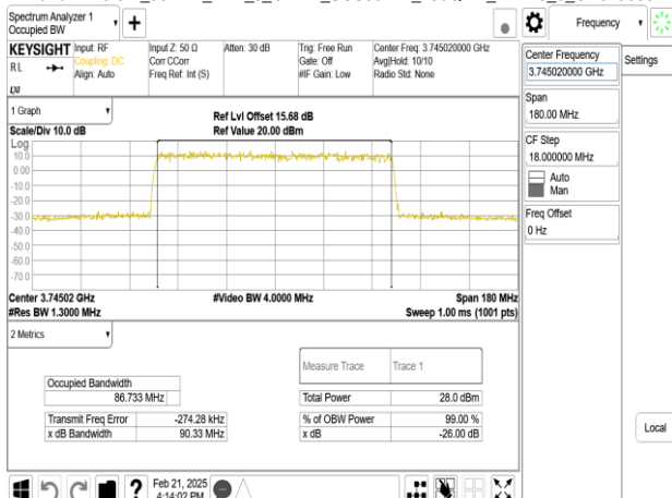
Band77-Part27_90MHz_DFT_s_OFDM_SCS30kHz_256QAM_RB243_0_CH649668
