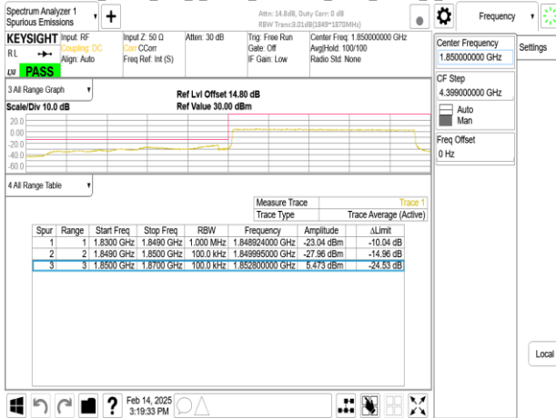
Band2_20MHz_DFT_s_OFDM_SCS15kHz_BPSK_RB1_0_CH372000
