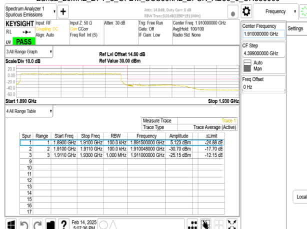
Band2_20MHz_DFT_s_OFDM_SCS30kHz_BPSK_RB50_0_CH380000
