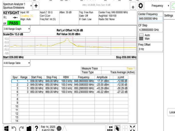
Band5_10MHz_DFT_s_OFDM_SCS30kHz_BPSK_RB24_0_CH168800
