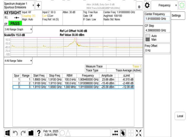
Band2_20MHz_CP_OFDM_SCS15kHz_QPSK_RB106_0_CH372000
