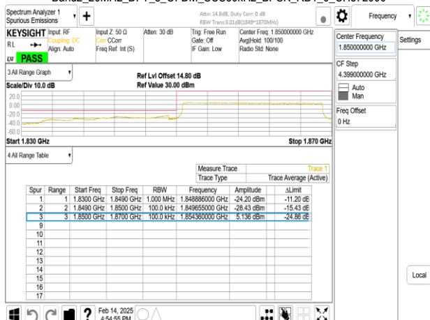
Band2_20MHz_DFT_s_OFDM_SCS30kHz_BPSK_RB1_0_CH372000
