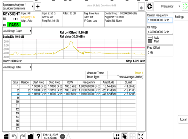
Band2_10MHz_DFT_s_OFDM_SCS30kHz_BPSK_RB1_23_CH381000
