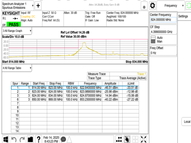
Band5_10MHz_CP_OFDM_SCS30kHz_QPSK_RB24_0_CH165800
