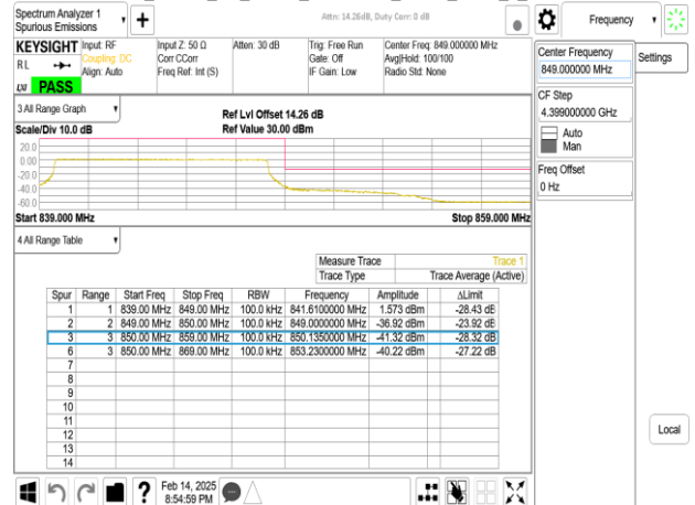
Band5_15MHz_DFT_s_OFDM_SCS15kHz_BPSK_RB1_0_CH166300
