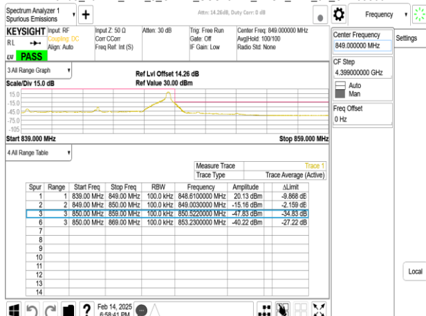
Band5_10MHz_DFT_s_OFDM_SCS15kHz_BPSK_RB1_51_CH168800
