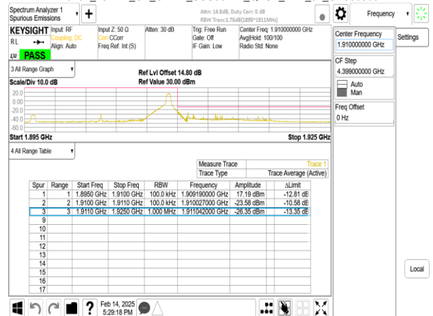
Band2_15MHz_CP_OFDM_SCS30kHz_QPSK_RB38_0_CH380500
