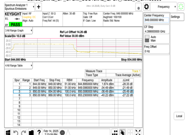
Band5_5MHz_CP_OFDM_SCS15kHz_QPSK_RB25_0_CH169300
