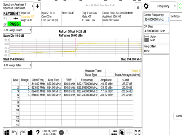
Band5_10MHz_CP_OFDM_SCS15kHz_QPSK_RB50_0_CH165800
