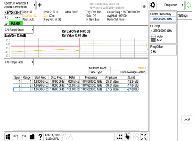
Band2_20MHz_CP_OFDM_SCS15kHz_QPSK_RB1_0_CH372000
