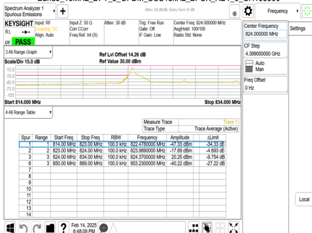
Band5_10MHz_DFT_s_OFDM_SCS15kHz_BPSK_RB50_0_CH165800
