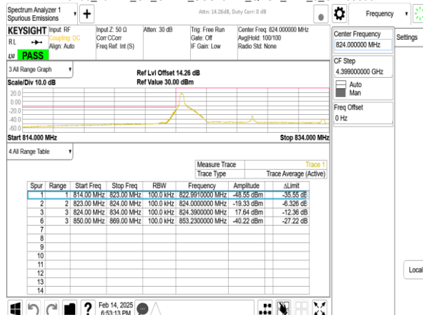
Band5_10MHz_CP_OFDM_SCS15kHz_QPSK_RB50_0_CH165800
