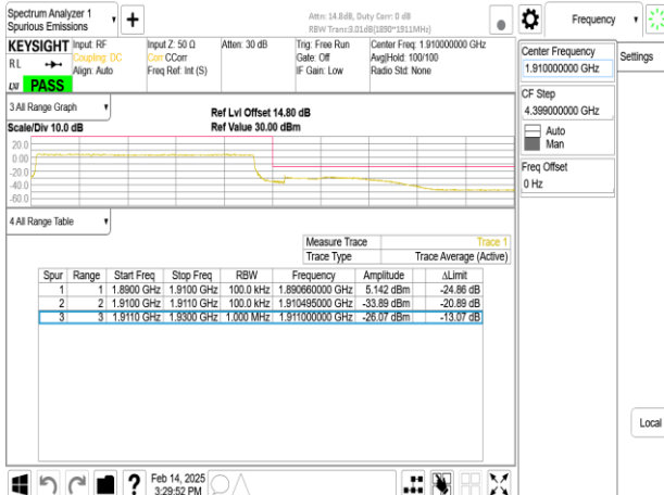
Band2_20MHz_DFT_s_OFDM_SCS15kHz_BPSK_RB100_0_CH380000
