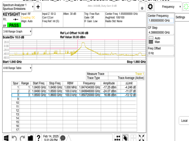
Band2_10MHz_DFT_s_OFDM_SCS30kHz_BPSK_RB24_0_CH371000
