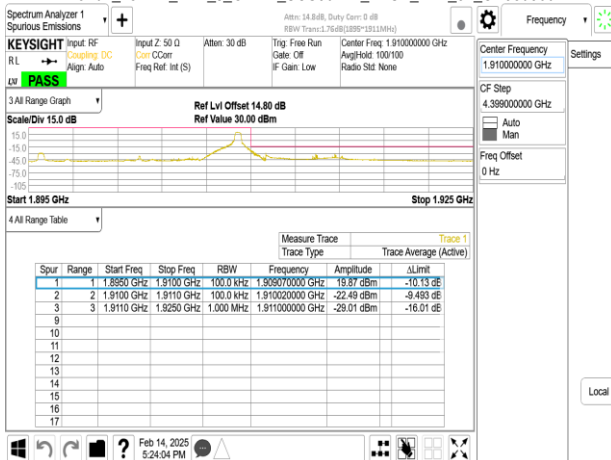
Band2_15MHz_DFT_s_OFDM_SCS30kHz_BPSK_RB36_0_CH380500
