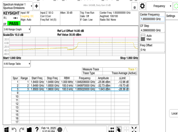
Band2_10MHz_CP_OFDM_SCS30kHz_QPSK_RB24_0_CH371000
