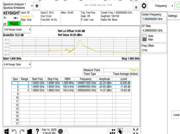
Band2_10MHz_CP_OFDM_SCS30kHz_QPSK_RB24_0_CH371000
