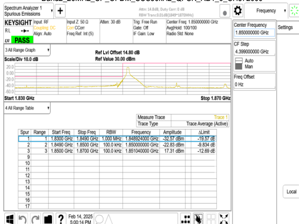
Band2_20MHz_CP_OFDM_SCS30kHz_QPSK_RB51_0_CH372000
