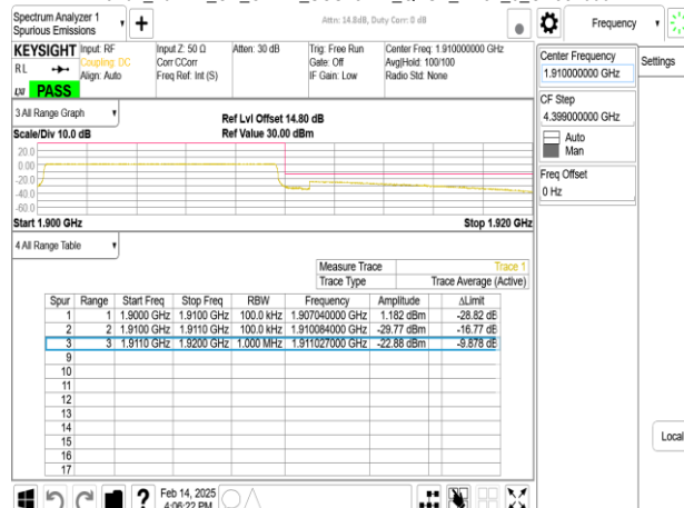
Band2_10MHz_CP_OFDM_SCS15kHz_QPSK_RB52_0_CH381000
