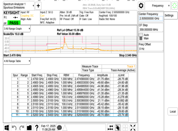
Band7_10MHz_CP_OFDM_SCS15kHz_QPSK_RB1_51_CH501000
