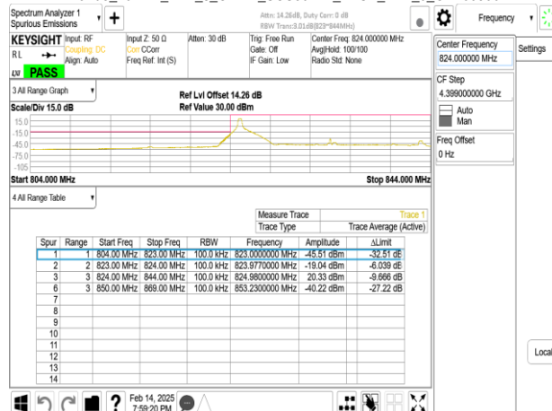
Band5_20MHz_DFT_s_OFDM_SCS30kHz_BPSK_RB50_0_CH166800
