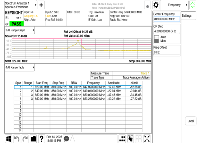
Band5_20MHz_CP_OFDM_SCS30kHz_QPSK_RB51_0_CH167800
