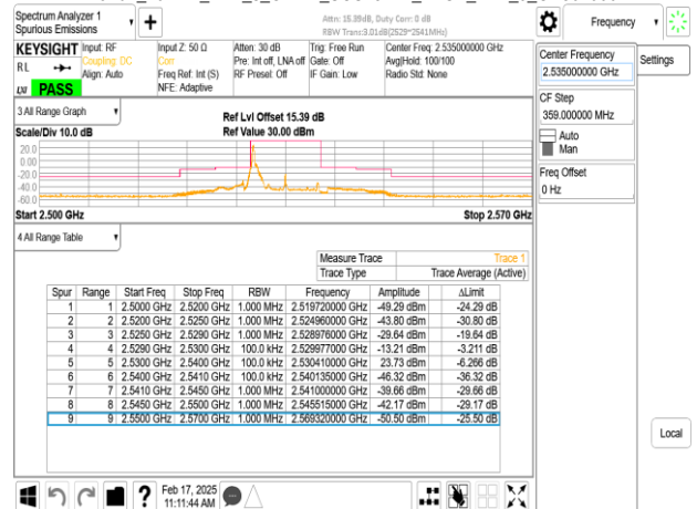
Band7_10MHz_DFT_s_OFDM_SCS15kHz_BPSK_RB1_51_CH507000
