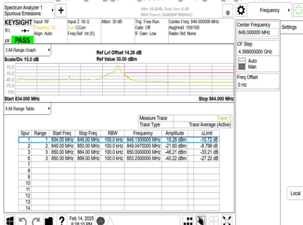
Band5_15MHz_DFT_s_OFDM_SCS30kHz_BPSK_RB1_37_CH168300
