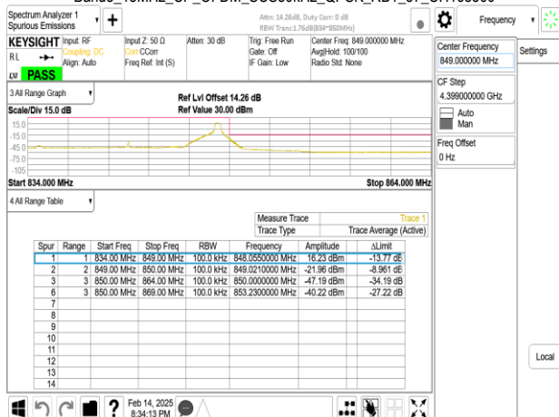
Band5_15MHz_CP_OFDM_SCS30kHz_QPSK_RB38_0_CH168300
