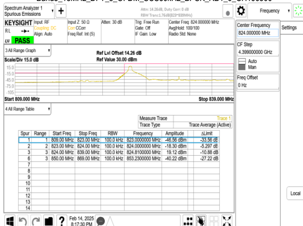
Band5_15MHz_DFT_s_OFDM_SCS30kHz_BPSK_RB36_0_CH166300
