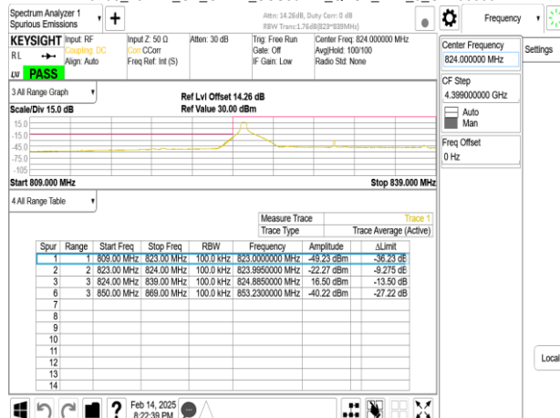
Band5_15MHz_CP_OFDM_SCS30kHz_QPSK_RB38_0_CH166300
