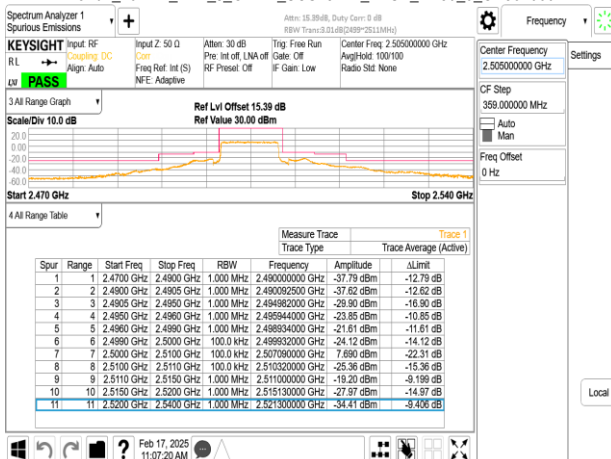
Band7_10MHz_DFT_s_OFDM_SCS15kHz_BPSK_RB50_0_CH501000
