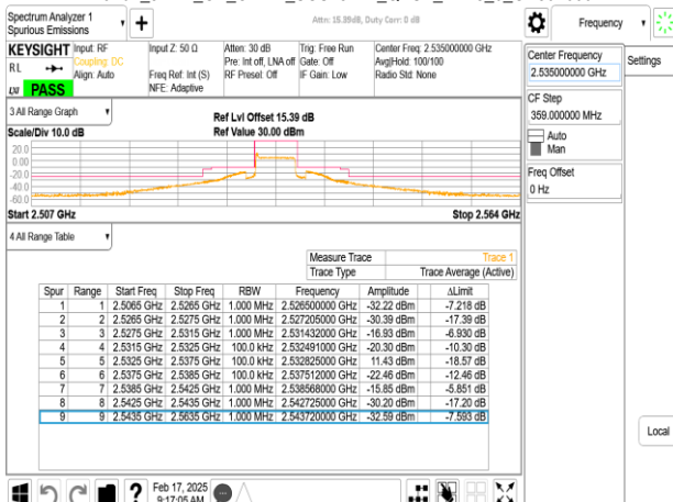
Band7_5MHz_CP_OFDM_SCS15kHz_QPSK_RB25_0_CH507000
