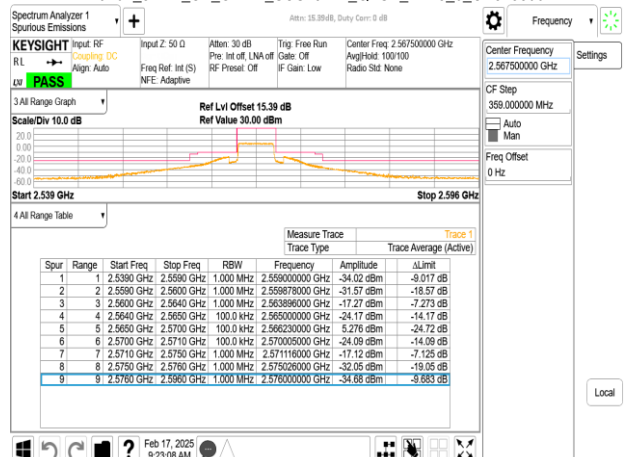
Band7_5MHz_CP_OFDM_SCS15kHz_QPSK_RB25_0_CH513500
