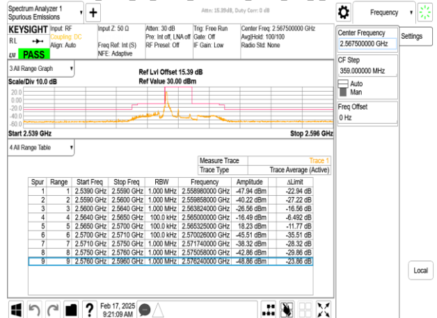
Band7_5MHz_CP_OFDM_SCS15kHz_QPSK_RB1_24_CH513500
