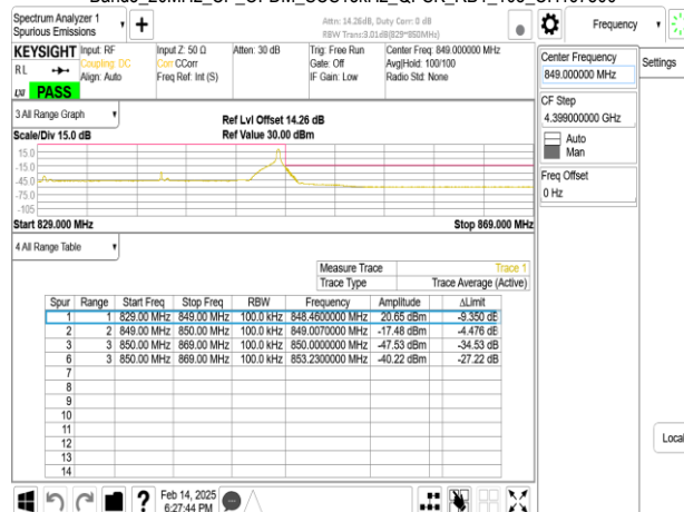
Band5_20MHz_DFT_s_OFDM_SCS30kHz_BPSK_RB1_0_CH166800
