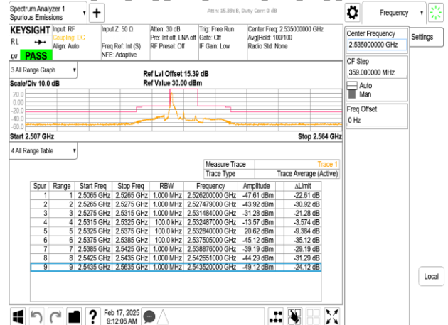
Band7_5MHz_DFT_s_OFDM_SCS15kHz_BPSK_RB1_24_CH507000
