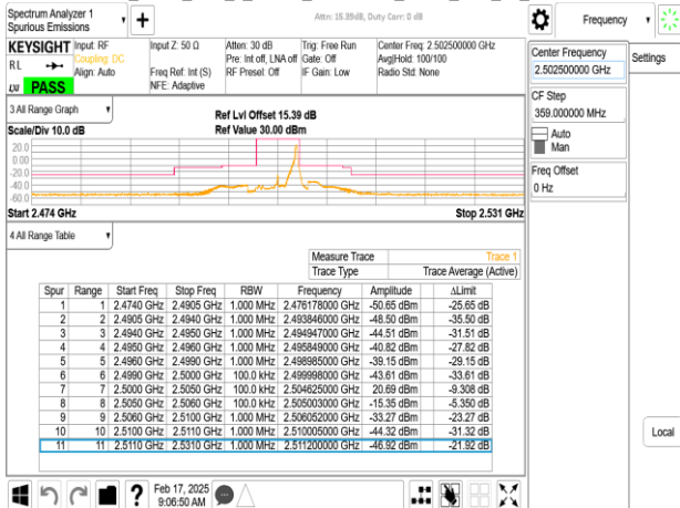
Band7_5MHz_DFT_s_OFDM_SCS15kHz_BPSK_RB25_0_CH500500
