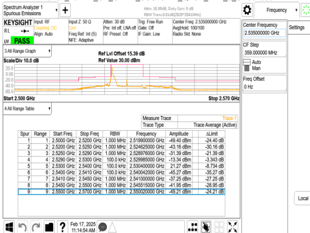
Band7_10MHz_CP_OFDM_SCS15kHz_QPSK_RB1_51_CH507000
