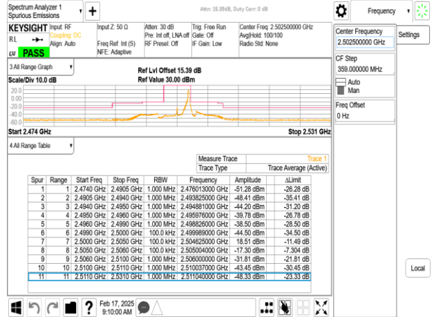
Band7_5MHz_CP_OFDM_SCS15kHz_QPSK_RB25_0_CH500500
