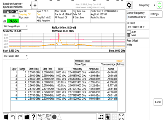
Band7_10MHz_CP_OFDM_SCS15kHz_QPSK_RB1_51_CH513000
