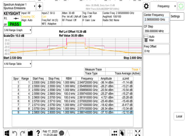
Band7_10MHz_CP_OFDM_SCS15kHz_QPSK_RB52_0_CH513000
