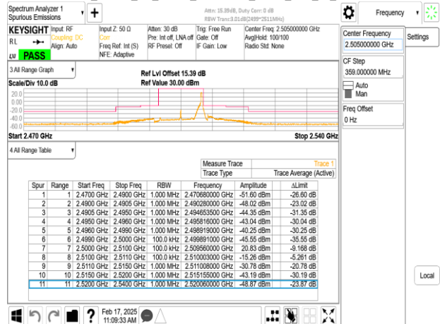
Band7_10MHz_CP_OFDM_SCS15kHz_QPSK_RB52_0_CH501000
