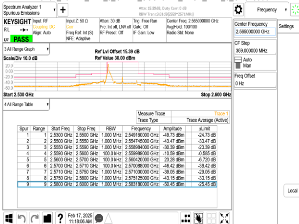
Band7_10MHz_DFT_s_OFDM_SCS15kHz_BPSK_RB1_51_CH513000
