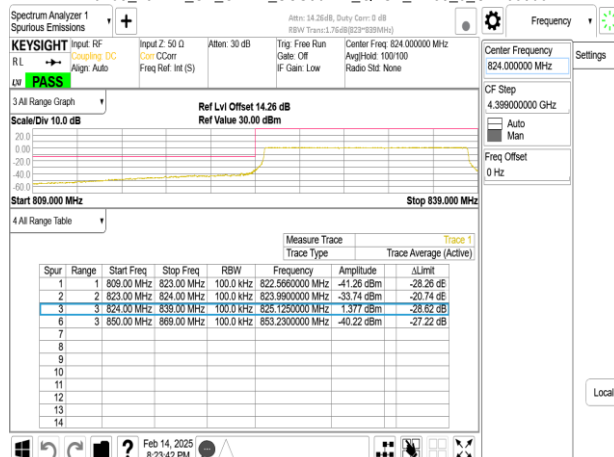
Band5_15MHz_CP_OFDM_SCS30kHz_QPSK_RB38_0_CH166300
