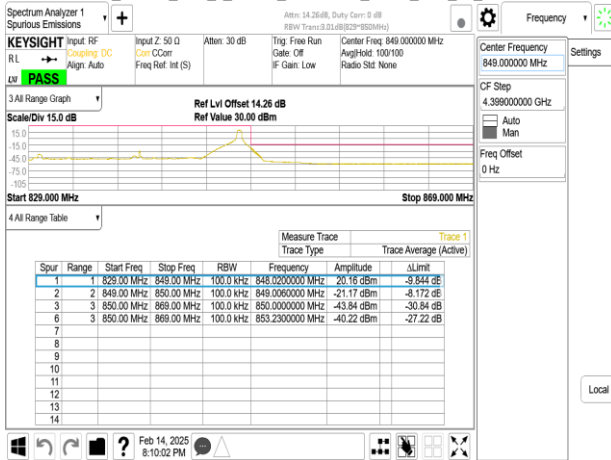
Band5_20MHz_DFT_s_OFDM_SCS30kHz_BPSK_RB50_0_CH167800
