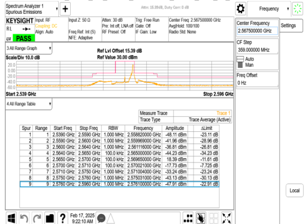
Band7_5MHz_CP_OFDM_SCS15kHz_QPSK_RB25_0_CH513500
