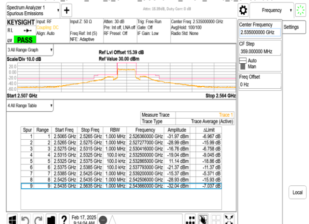
Band7_5MHz_DFT_s_OFDM_SCS15kHz_BPSK_RB25_0_CH507000
