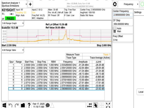
Band7_10MHz_DFT_s_OFDM_SCS15kHz_BPSK_RB50_0_CH513000
