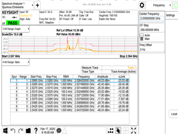
Band7_5MHz_CP_OFDM_SCS15kHz_QPSK_RB25_0_CH507000
