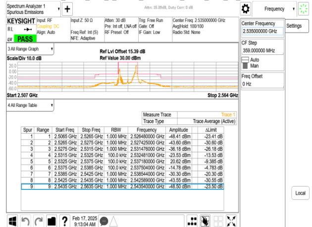
Band7_5MHz_DFT_s_OFDM_SCS15kHz_BPSK_RB25_0_CH507000
