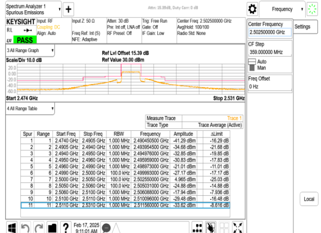
Band7_5MHz_CP_OFDM_SCS15kHz_QPSK_RB25_0_CH500500
