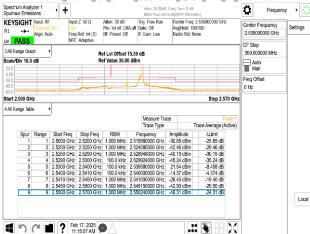
Band7_10MHz_CP_OFDM_SCS15kHz_QPSK_RB52_0_CH507000
