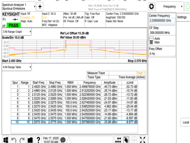
Band7_15MHz_CP_OFDM_SCS15kHz_QPSK_RB79_0_CH507000
