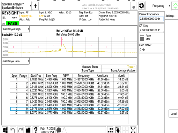
Band7_15MHz_CP_OFDM_SCS30kHz_QPSK_RB1_37_CH507000
