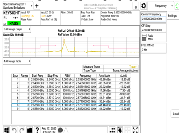
Band7_15MHz_CP_OFDM_SCS30kHz_QPSK_RB1_37_CH512500
