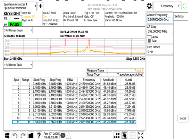
Band7_15MHz_CP_OFDM_SCS15kHz_QPSK_RB79_0_CH501500
