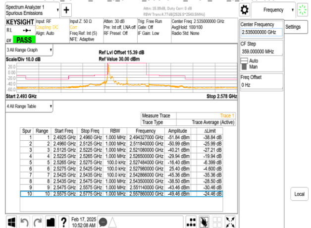
Band7_15MHz_DFT_s_OFDM_SCS15kHz_BPSK_RB1_78_CH507000
