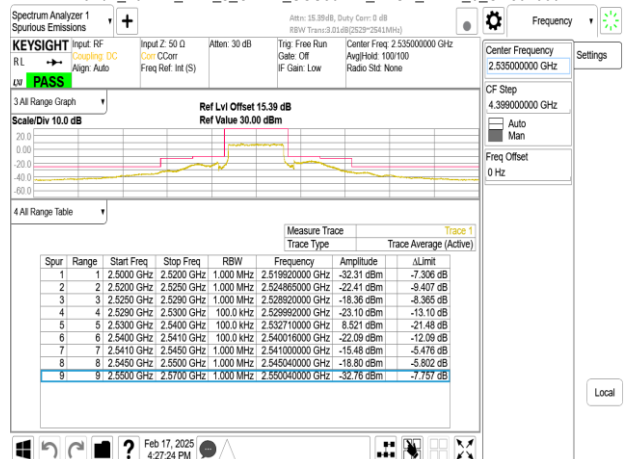
Band7_10MHz_DFT_s_OFDM_SCS30kHz_BPSK_RB24_0_CH507000
