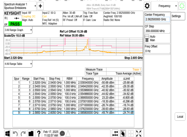
Band7_15MHz_CP_OFDM_SCS15kHz_QPSK_RB79_0_CH512500
