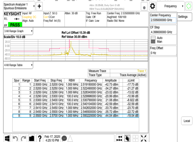
Band7_10MHz_DFT_s_OFDM_SCS30kHz_BPSK_RB1_23_CH507000
