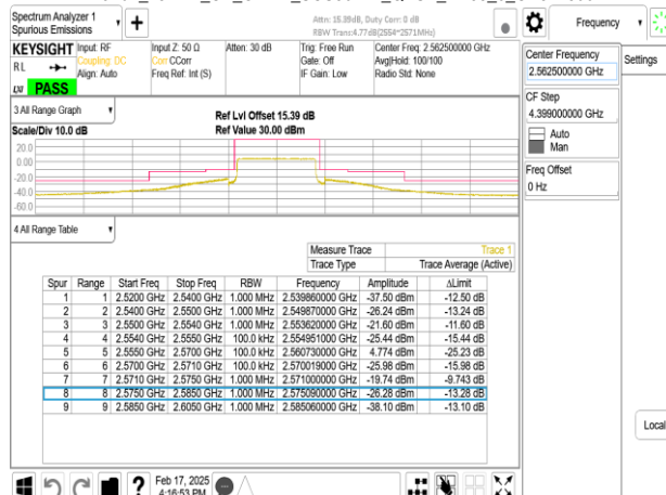
Band7_15MHz_CP_OFDM_SCS30kHz_QPSK_RB38_0_CH512500
