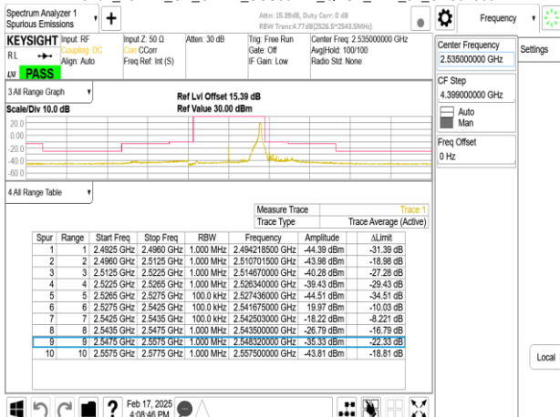
Band7_15MHz_CP_OFDM_SCS30kHz_QPSK_RB38_0_CH507000
