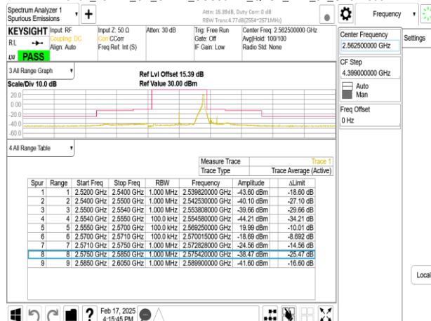
Band7_15MHz_CP_OFDM_SCS30kHz_QPSK_RB38_0_CH512500
