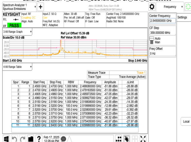
Band7_50MHz_DFT_s_OFDM_SCS15kHz_BPSK_RB1_269_CH509000
