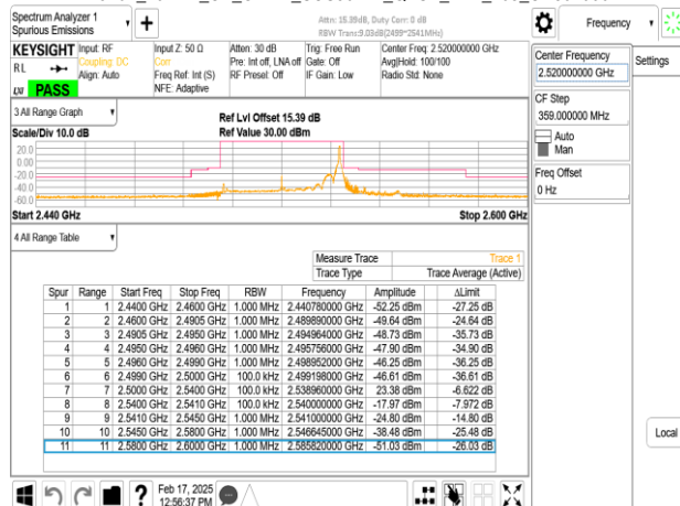
Band7 40MHz_CP_OFDM_SCS30kHz_QPSK_RB1_105_CH504000
