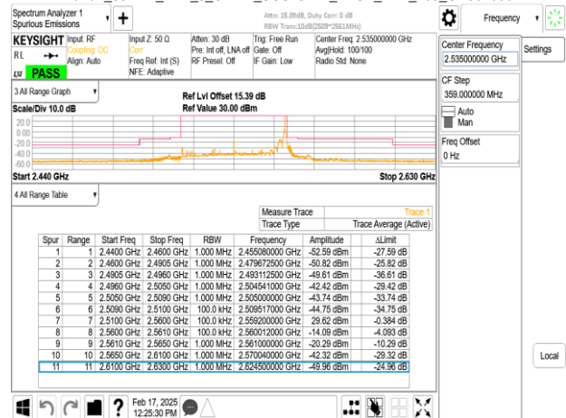
Band7_50MHz_DFT_s_OFDM_SCS15kHz_BPSK_RB270_0_CH507000
