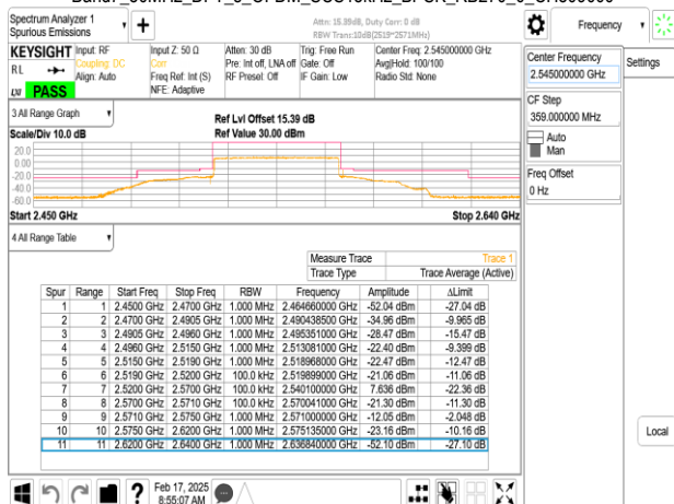
Band7_50MHz_DFT_s_OFDM_SCS15kHz_BPSK_RB270_0_CH509000
