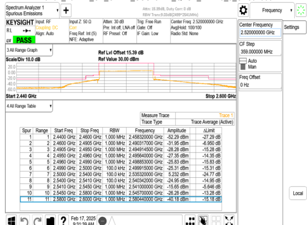
Band7_40MHz_CP_OFDM_SCS15kHz_QPSK_RB216_0_CH504000
