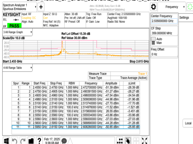
Band7_40MHz_CP_OFDM_SCS15kHz_QPSK_RB1_215_CH507000
