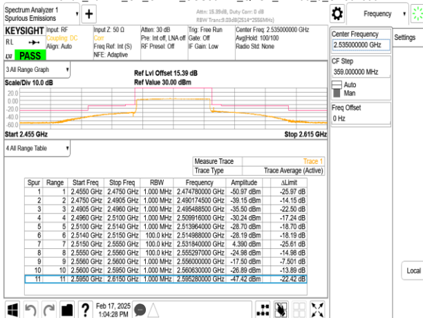
Band7_40MHz_CP_OFDM_SCS30kHz_QPSK_RB1_0_CH507000
