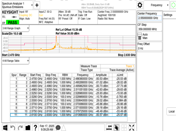
Band7_40MHz_DFT_s_OFDM_SCS15kHz_BPSK_RB1_215_CH510000
