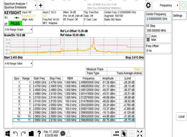
Band7_40MHz_DFT_s_OFDM_SCS15kHz_BPSK_RB216_0_CH507000
