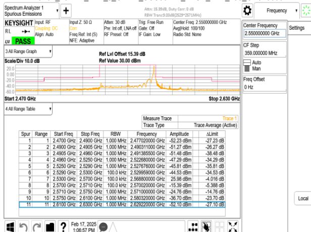
Band7 40MHz_DFT_s_OFDM_SCS30kHz_BPSK_RB1_105_CH510000
