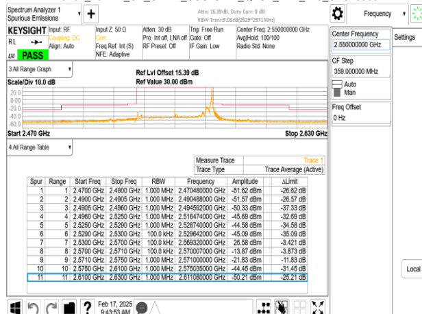
Band7_40MHz_CP_OFDM_SCS15kHz_QPSK_RB216_0_CH510000
