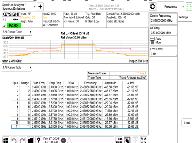
Band7_40MHz_DFT_s_OFDM_SCS15kHz_BPSK_RB216_0_CH510000
