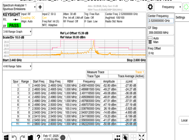
Band7_40MHz_DFT_s_OFDM_SCS30kHz_BPSK_RB1_105_CH504000
