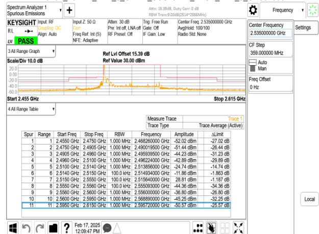
Band7_40MHz_DFT_s_OFDM_SCS15kHz_BPSK_RB1_215_CH507000
