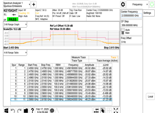
Band7_40MHz_DFT_s_OFDM_SCS15kHz_BPSK_RB216_0_CH507000
