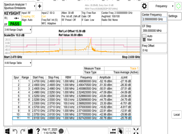
Band7_40MHz_CP_OFDM_SCS30kHz_QPSK_RB1_105_CH510000
