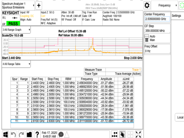
Band7_50MHz_CP_OFDM_SCS15kHz_QPSK_RB270_0_CH507000
