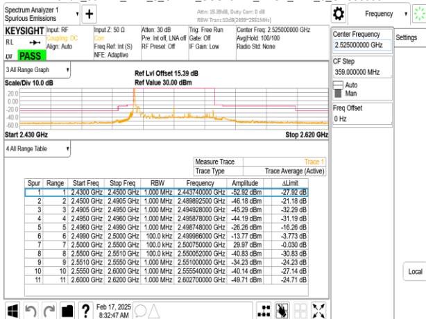
Band7_50MHz_DFT_s_OFDM_SCS15kHz_BPSK_RB1_269_CH505000
