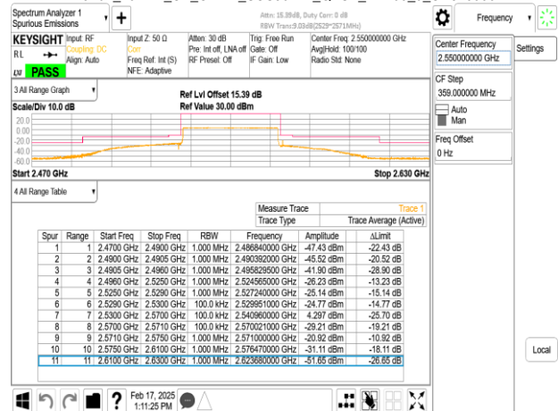
Band7_40MHz_CP_OFDM_SCS30kHz_QPSK_RB1_0_CH510000
