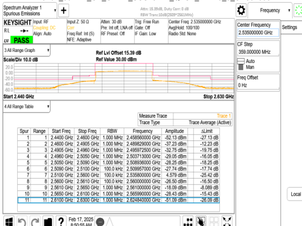
Band7_50MHz_CP_OFDM_SCS15kHz_QPSK_RB270_0_CH507000
