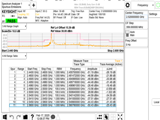
Band7_40MHz_DFT_s_OFDM_SCS15kHz_BPSK_RB1_215_CH504000
