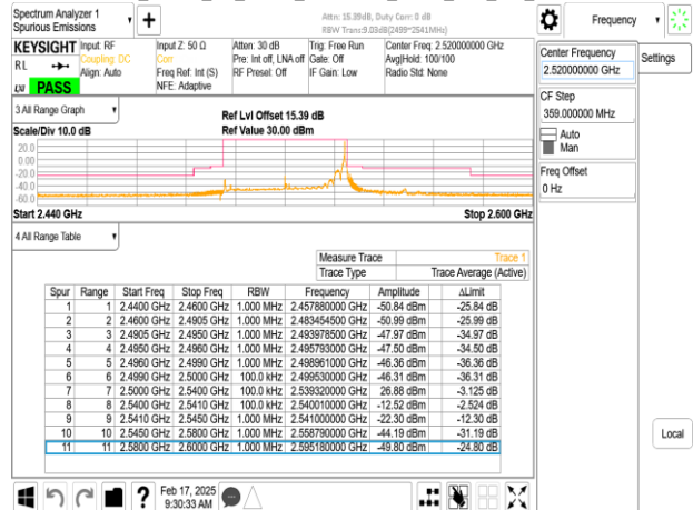
Band7_40MHz_CP_OFDM_SCS15kHz_QPSK_RB216_0_CH504000
