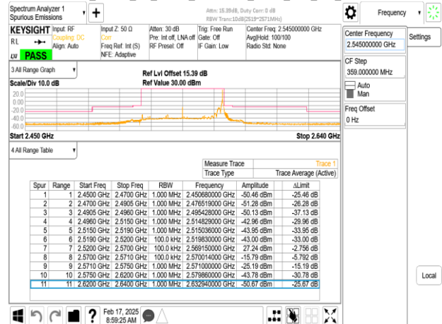
Band7_50MHz_CP_OFDM_SCS15kHz_QPSK_RB270_0_CH509000
