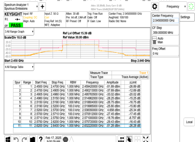
Band7_50MHz_CP_OFDM_SCS15kHz_QPSK_RB270_0_CH509000
