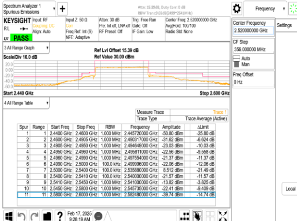
Band7_40MHz_DFT_s_OFDM_SCS15kHz_BPSK_RB216_0_CH504000
