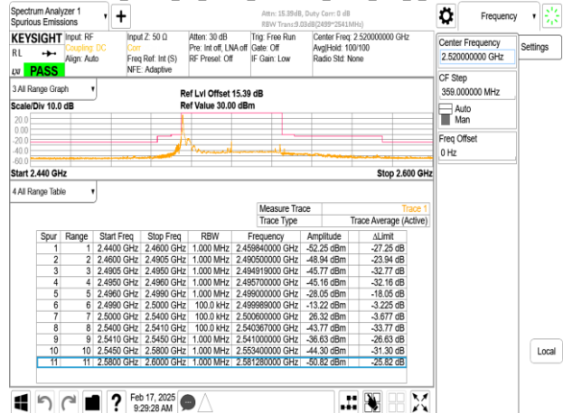
Band7_40MHz_CP_OFDM_SCS15kHz_QPSK_RB1_215_CH504000
