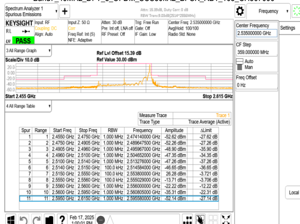
Band7_40MHz_DFT_s_OFDM_SCS30kHz_BPSK_RB1_105_CH507000
