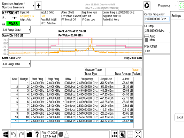
Band7_40MHz_DFT_s_OFDM_SCS15kHz_BPSK_RB216_0_CH504000
