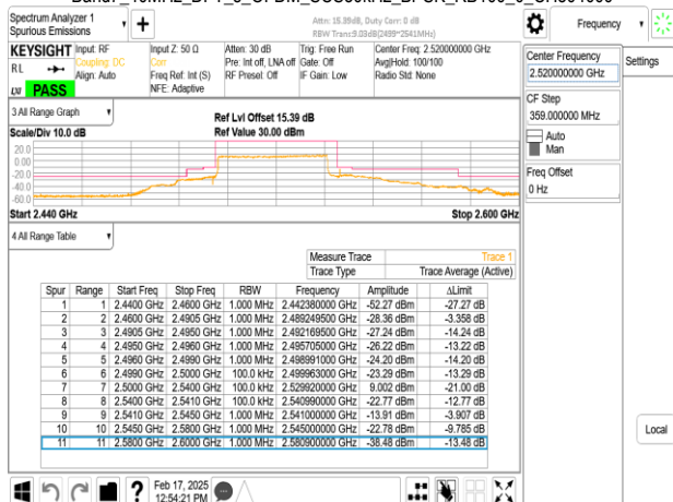
Band7_40MHz_DFT_s_OFDM_SCS30kHz_BPSK_RB1_0_CH504000
