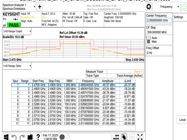
Band7 40MHz_DFT_s_OFDM_SCS30kHz_BPSK_RB1_0_CH510000
