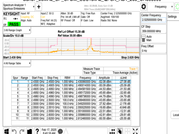
Band7_50MHz_CP_OFDM_SCS15kHz_QPSK_RB270_0_CH505000
