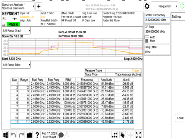
Band7_50MHz_DFT_s_OFDM_SCS15kHz_BPSK_RB270_0_CH505000
