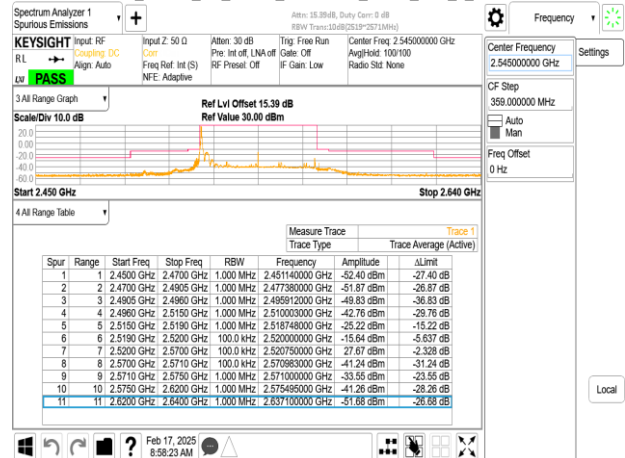
Band7_50MHz_CP_OFDM_SCS15kHz_QPSK_RB1_269_CH509000
