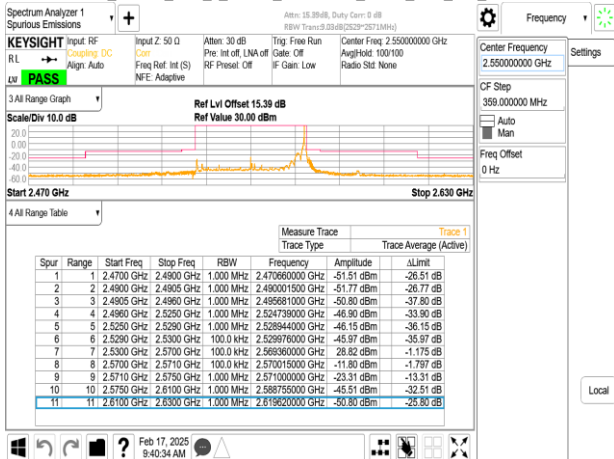
Band7_40MHz_DFT_s_OFDM_SCS15kHz_BPSK_RB216_0_CH510000
