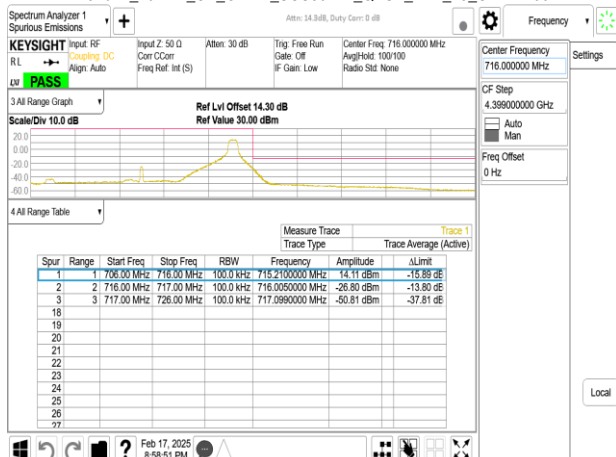
Band12_10MHz_CP_OFDM_SCS30kHz_QPSK_RB1_23_CH142200
