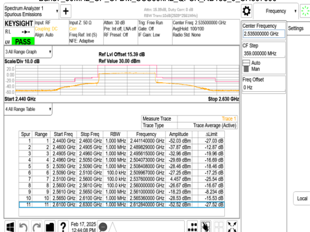
Band7_50MHz_CP_OFDM_SCS30kHz_QPSK_RB1_0_CH507000
