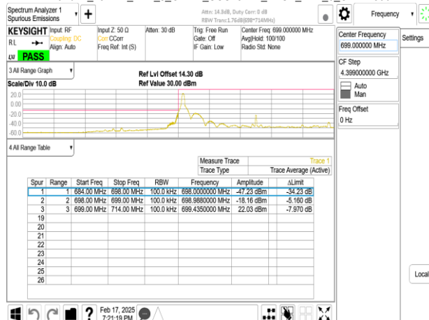
Band12_15MHz_DFT_s_OFDM_SCS15kHz_BPSK_RB75_0_CH141300
