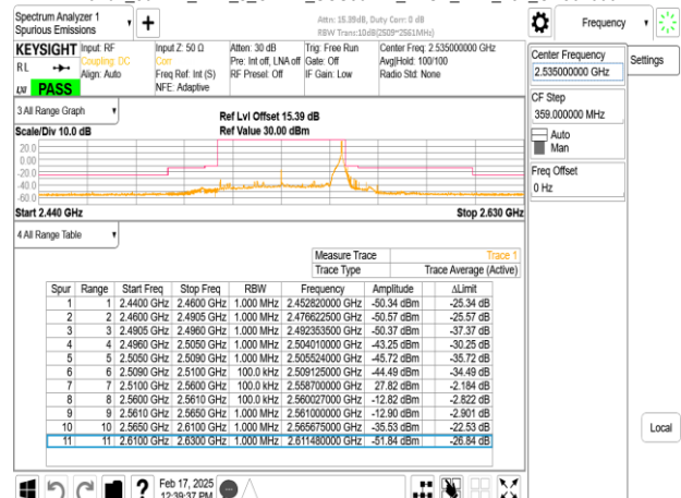
Band7_50MHz_DFT_s_OFDM_SCS30kHz_BPSK_RB1_132_CH507000
