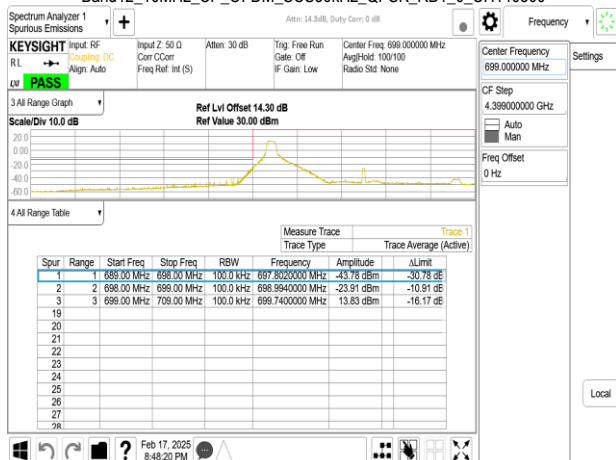
Band12_10MHz_CP_OFDM_SCS30kHz_QPSK_RB24_0_CH140800
