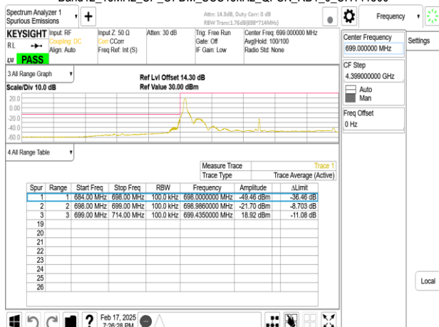
Band12_15MHz_CP_OFDM_SCS15kHz_QPSK_RB1_0_CH141300
