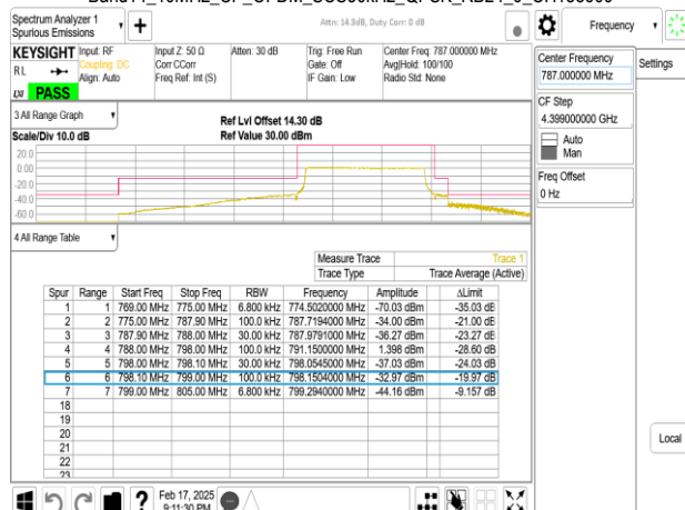
Band14_10MHz_CP_OFDM_SCS30kHz_QPSK_RB24_0_CH158600
