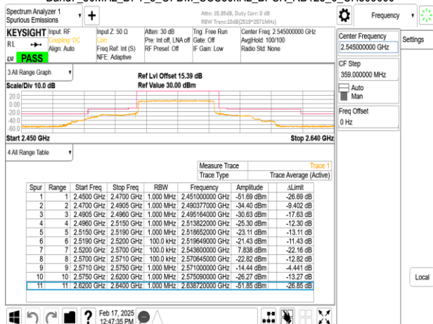
Band7_50MHz_DFT_s_OFDM_SCS30kHz_BPSK_RB1_0_CH509000
