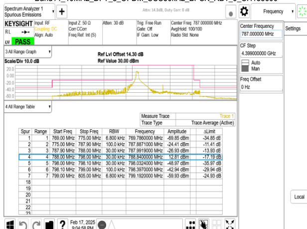
Band14_10MHz_DFT_s_OFDM_SCS30kHz_BPSK_RB1_0_CH158600
