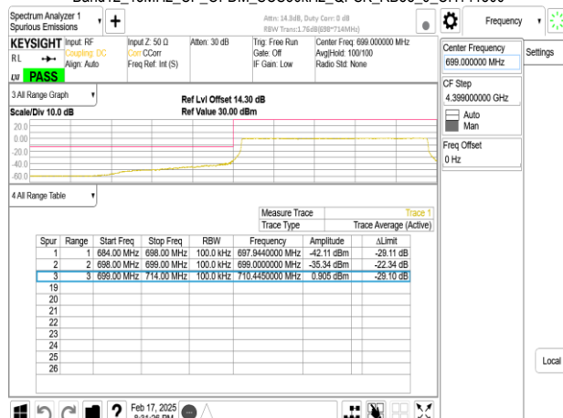
Band12_15MHz_CP_OFDM_SCS30kHz_QPSK_RB38_0_CH141300
