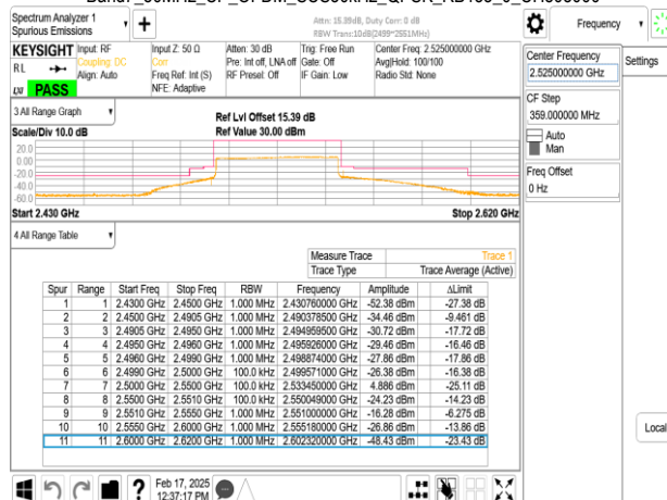
Band7_50MHz_CP_OFDM_SCS30kHz_QPSK_RB1_0_CH505000
