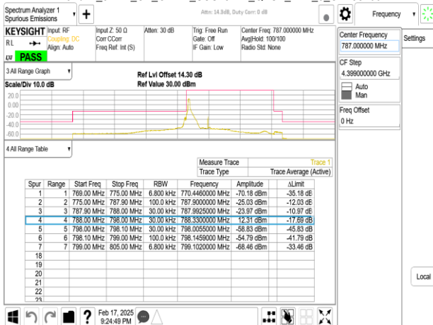
Band14_5MHz_CP_OFDM_SCS15kHz_QPSK_RB25_0_CH158100
