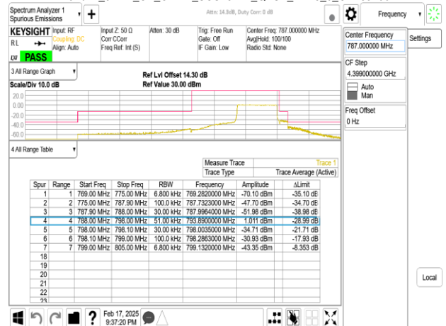
Band14_10MHz_DFT_s_OFDM_SCS15kHz_BPSK_RB1_0_CH158600
