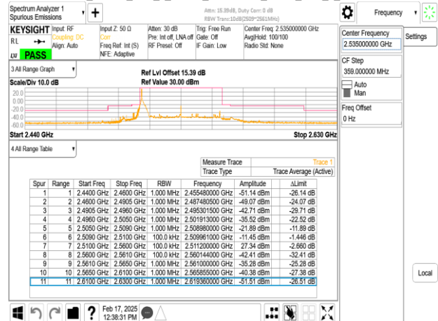
Band7_50MHz_DFT_s_OFDM_SCS30kHz_BPSK_RB1_132_CH507000
