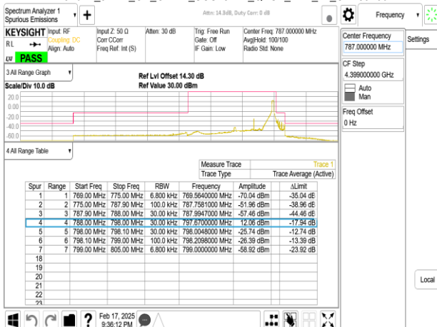
Band14_5MHz_CP_OFDM_SCS15kHz_QPSK_RB1_24_CH159100
