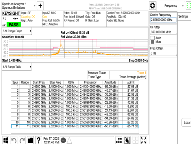
Band7_50MHz_DFT_s_OFDM_SCS30kHz_BPSK_RB1_132_CH505000
