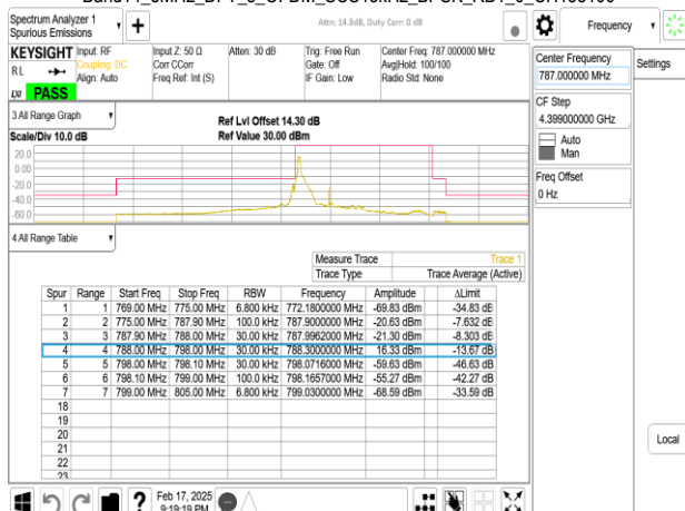
Band14_5MHz_DFT_s_OFDM_SCS15kHz_BPSK_RB1_0_CH158100
