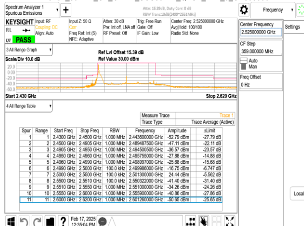
Band7_50MHz_CP_OFDM_SCS30kHz_QPSK_RB1_132_CH505000
