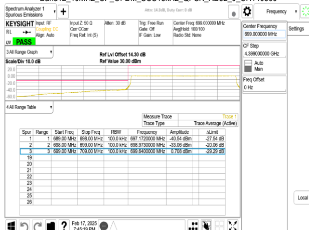
Band12_10MHz_CP_OFDM_SCS15kHz_QPSK_RB52_0_CH140800
