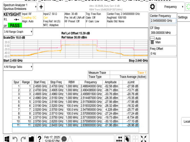
Band7_50MHz_CP_OFDM_SCS30kHz_QPSK_RB1_0_CH509000
