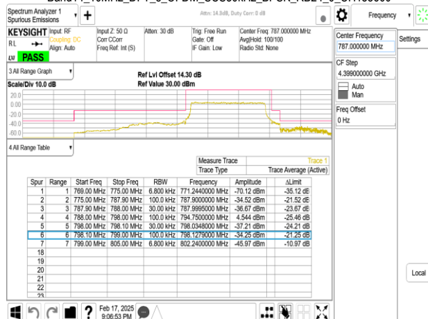
Band14_10MHz_CP_OFDM_SCS30kHz_QPSK_RB1_0_CH158600
