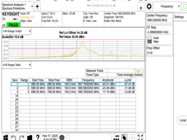
Band12_10MHz_DFT_s_OFDM_SCS30kHz_BPSK_RB1_0_CH140800
