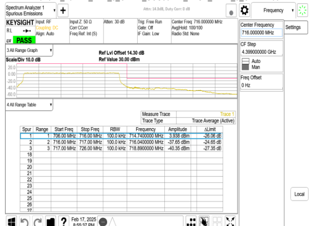
Band12_10MHz_DFT_s_OFDM_SCS30kHz_BPSK_RB24_0_CH142200
