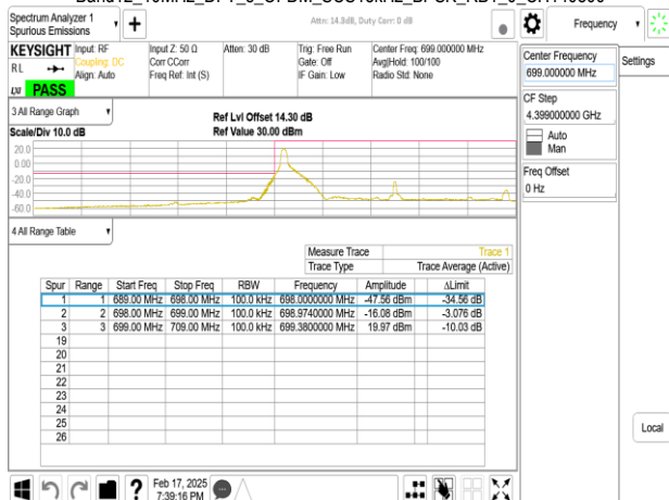
Band12_10MHz_DFT_s_OFDM_SCS15kHz_BPSK_RB50_0_CH140800
