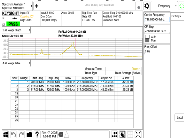
Band12_10MHz_CP_OFDM_SCS15kHz_QPSK_RB52_0_CH142200
