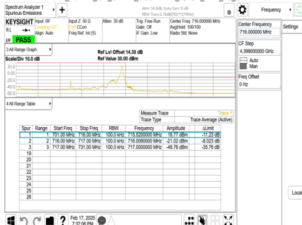
Band12_15MHz_CP_OFDM_SCS15kHz_QPSK_RB79_0_CH141700
