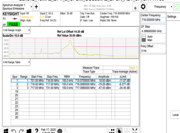
Band12_15MHz_DFT_s_OFDM_SCS30kHz_BPSK_RB1_37_CH141700
