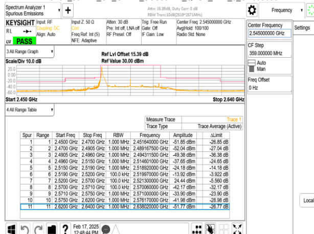
Band7_50MHz_CP_OFDM_SCS30kHz_QPSK_RB1_132_CH509000
