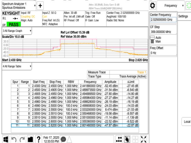
Band7_50MHz_DFT_s_OFDM_SCS30kHz_BPSK_RB1_0_CH505000
