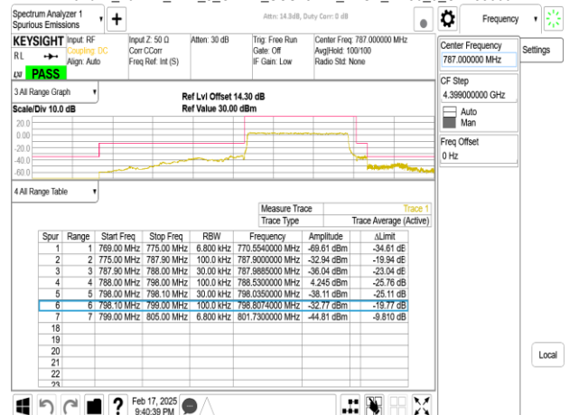
Band14_10MHz_DFT_s_OFDM_SCS15kHz_BPSK_RB50_0_CH158600
