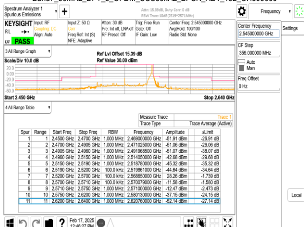
Band7_50MHz_DFT_s_OFDM_SCS30kHz_BPSK_RB1_132_CH509000
