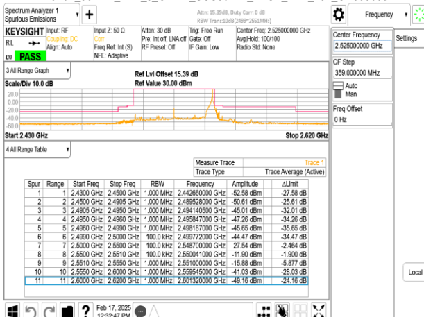
Band7_50MHz_DFT_s_OFDM_SCS30kHz_BPSK_RB1_132_CH505000
