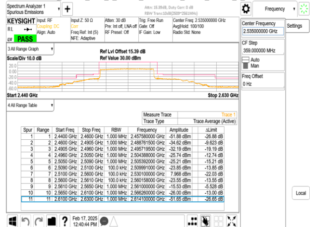
Band7_50MHz_DFT_s_OFDM_SCS30kHz_BPSK_RB1_0_CH507000
