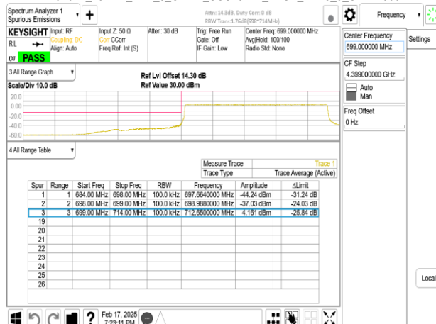
Band12_15MHz_DFT_s_OFDM_SCS15kHz_BPSK_RB75_0_CH141300
