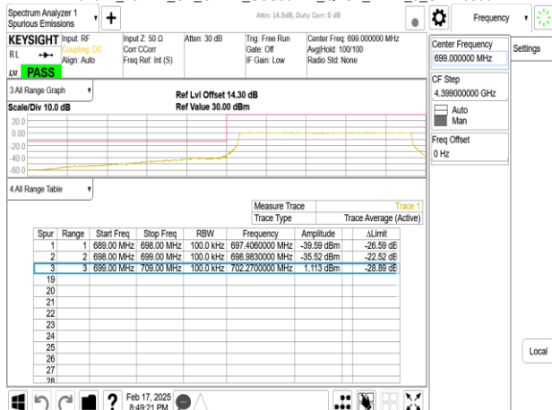
Band12_10MHz_CP_OFDM_SCS30kHz_QPSK_RB1_23_CH142200
