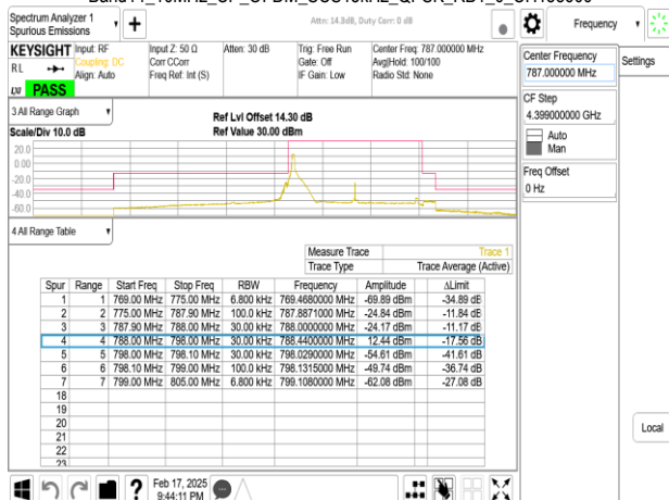
Band14_10MHz_CP_OFDM_SCS15kHz_QPSK_RB25_0_CH158600
