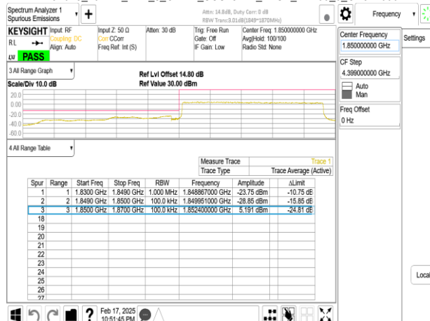
Band25_20MHz_DFT_s_OFDM_SCS15kHz_BPSK_RB1_0_CH372000
