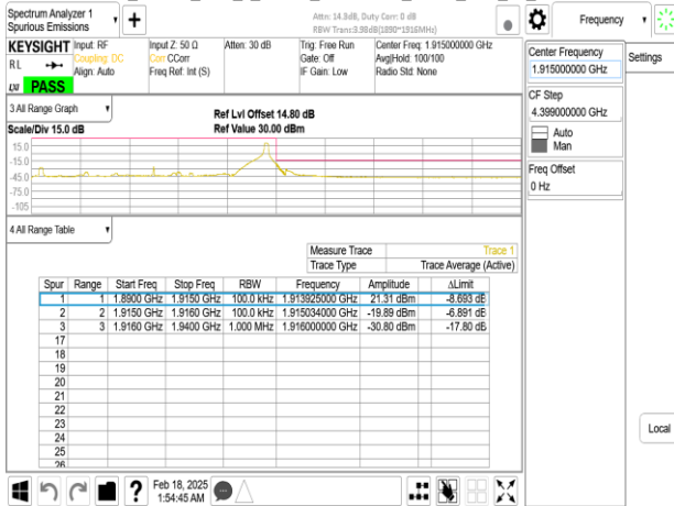
Band25_25MHz_DFT_s_OFDM_SCS30kHz_BPSK_RB64_0_CH380500
