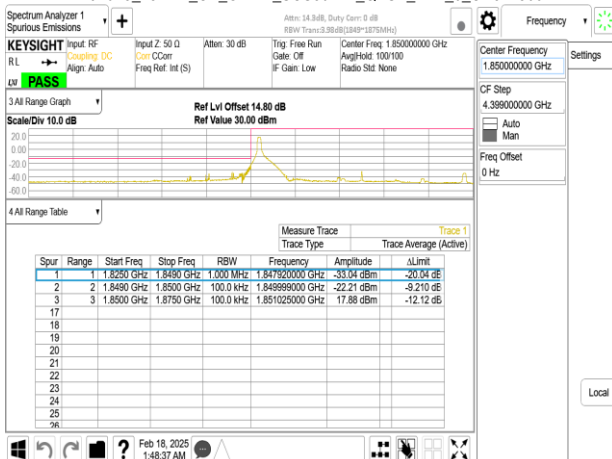
Band25_25MHz_CP_OFDM_SCS30kHz_QPSK_RB1_0_CH372500
