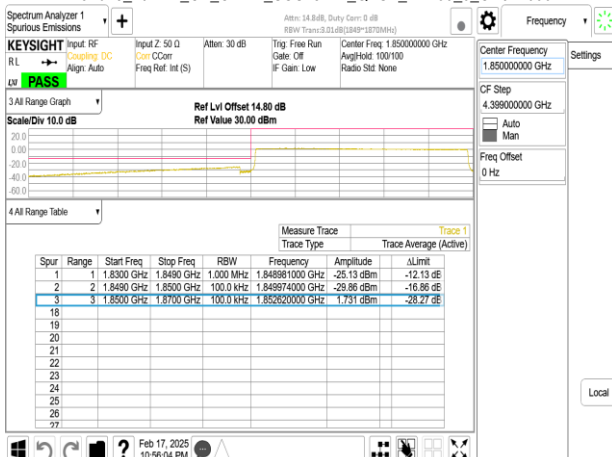
Band25_20MHz_CP_OFDM_SCS15kHz_QPSK_RB106_0_CH372000
