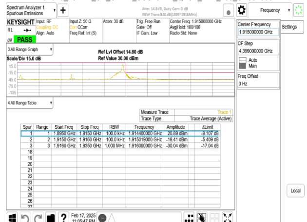
Band25_20MHz_CP_OFDM_SCS15kHz_QPSK_RB1_105_CH381000
