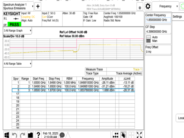
Band25_20MHz_CP_OFDM_SCS30kHz_QPSK_RB51_0_CH372000
