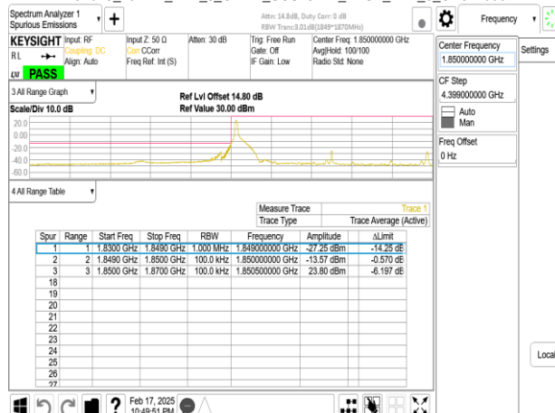
Band25_20MHz_DFT_s_OFDM_SCS15kHz_BPSK_RB1_0_CH372000
