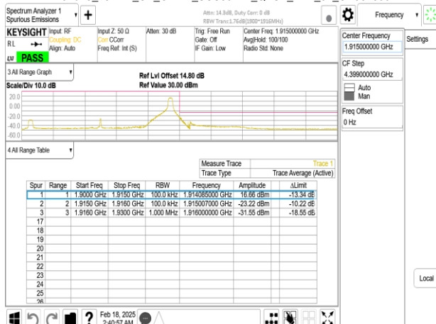
Band25_15MHz_CP_OFDM_SCS30kHz_QPSK_RB1_37_CH381500
