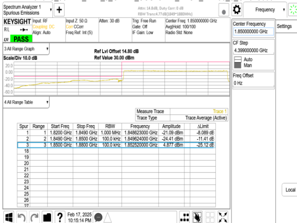
Band25_30MHz_DFT_s_OFDM_SCS15kHz_BPSK_RB1_0_CH373000
