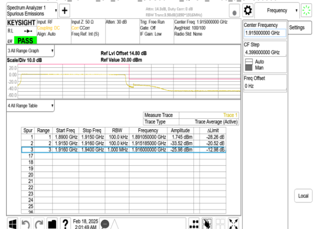
Band25_25MHz_CP_OFDM_SCS30kHz_QPSK_RB65_0_CH380500
