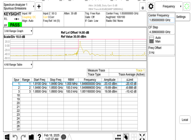
Band25_40MHz_CP_OFDM_SCS30kHz_QPSK_RB1_0_CH374000
