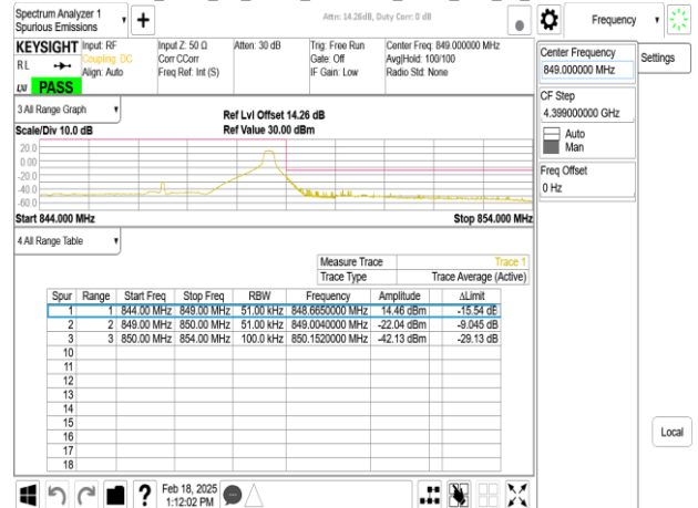
Band26_5MHz_CP_OFDM_SCS15kHz_QPSK_RB25_0_CH169300
