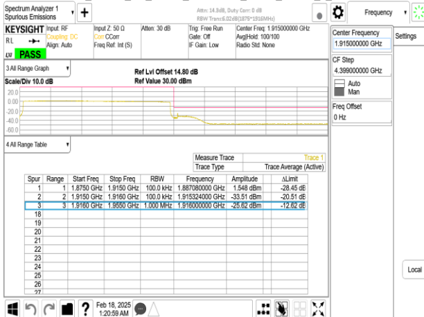
Band25_40MHz_CP_OFDM_SCS30kHz_QPSK_RB1_105_CH379000
