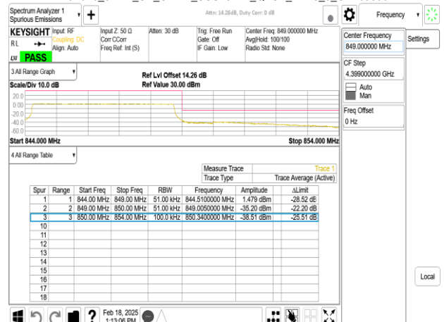
Band26_5MHz_CP_OFDM_SCS15kHz_QPSK_RB25_0_CH169300
