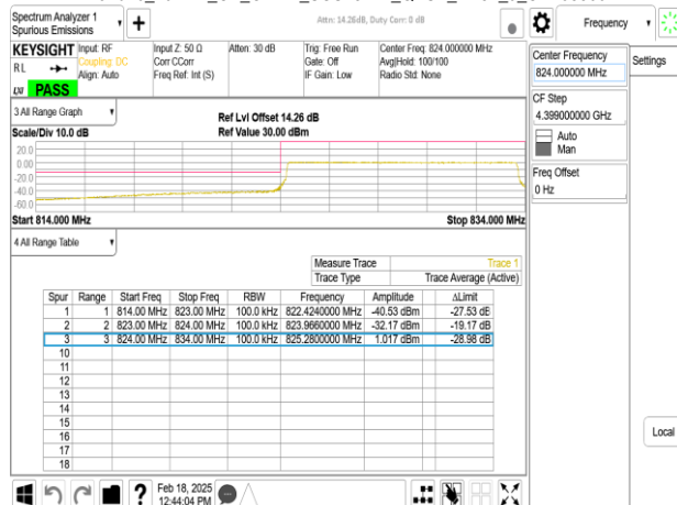
Band26_10MHz_CP_OFDM_SCS15kHz_QPSK_RB52_0_CH165800
