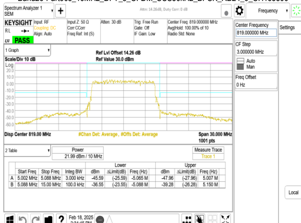
Band26-Part90s_10MHz_CP_OFDM_SCS30kHz_QPSK_RB1_0_CH163800
