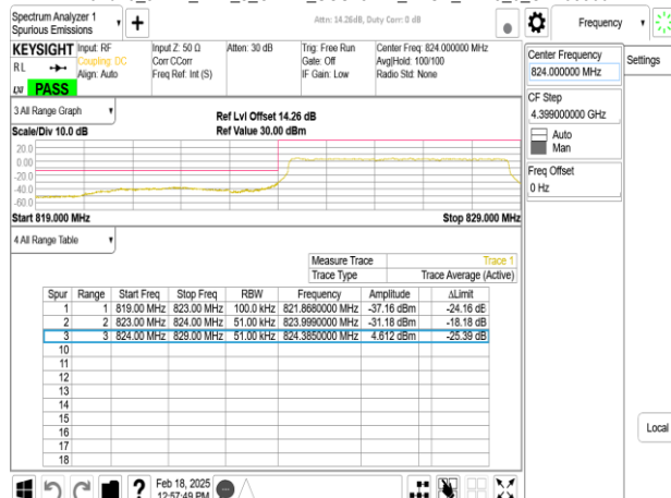
Band26_5MHz_DFT_s_OFDM_SCS15kHz_BPSK_RB25_0_CH165300
