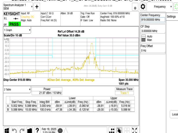
Band26-Part90s_10MHz_DFT_s_OFDM_SCS30kHz_BPSK_RB1_23_CH163800
