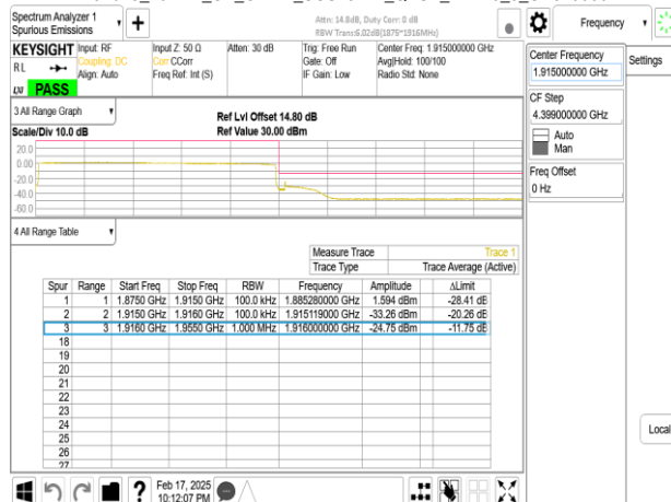
Band25_40MHz_CP_OFDM_SCS15kHz_QPSK_RB216_0_CH379000
