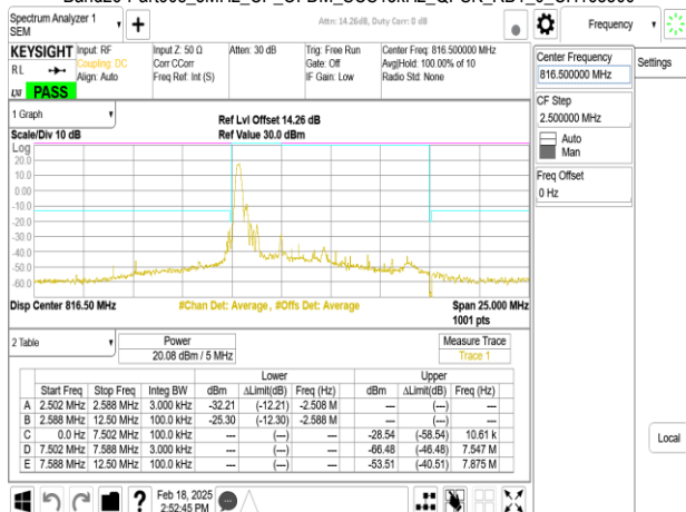
Band26-Part90s_5MHz_CP_OFDM_SCS15kHz_QPSK_RB25_0_CH163300
