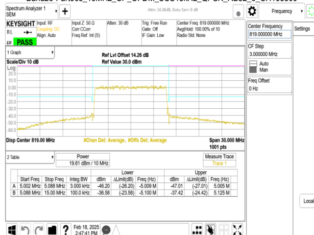
Band26-Part90s_10MHz_DFT_s_OFDM_SCS30kHz_BPSK_RB1_0_CH163800
