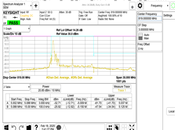
Band26-Part90s_10MHz_DFT_s_OFDM_SCS15kHz_BPSK_RB1_51_CH163800
