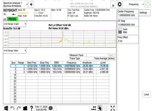
Band25_40MHz_DFT_s_OFDM_SCS15kHz_BPSK_RB216_0_CH374000
