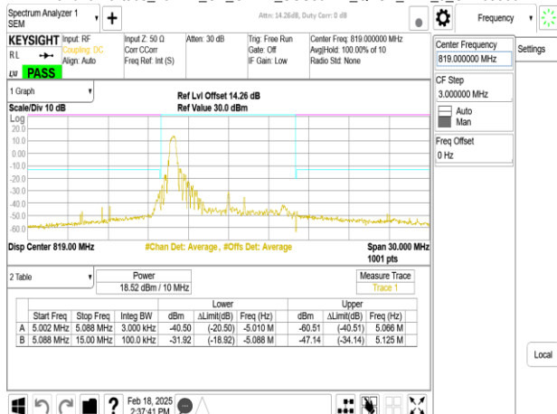
Band26-Part90s_10MHz_CP_OFDM_SCS30kHz_QPSK_RB1_23_CH163800
