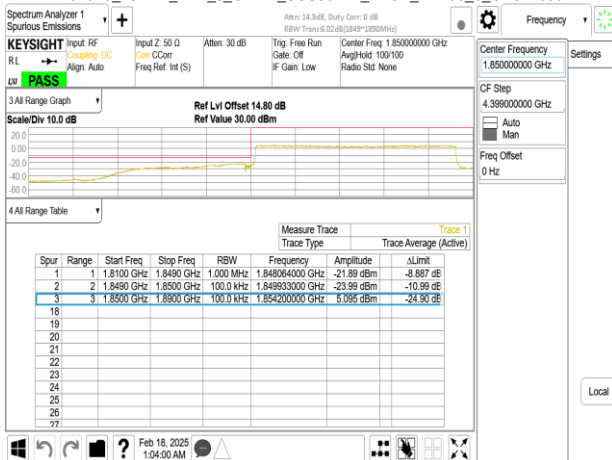
Band25_40MHz_DFT_s_OFDM_SCS30kHz_BPSK_RB1_0_CH374000
