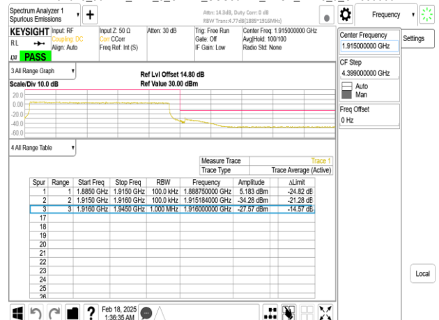
Band25_30MHz_DFT_s_OFDM_SCS30kHz_BPSK_RB75_0_CH380000
