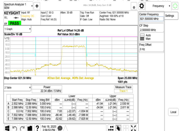
Band26-Part90s_5MHz_DFT_s_OFDM_SCS15kHz_BPSK_RB25_0_CH164300
