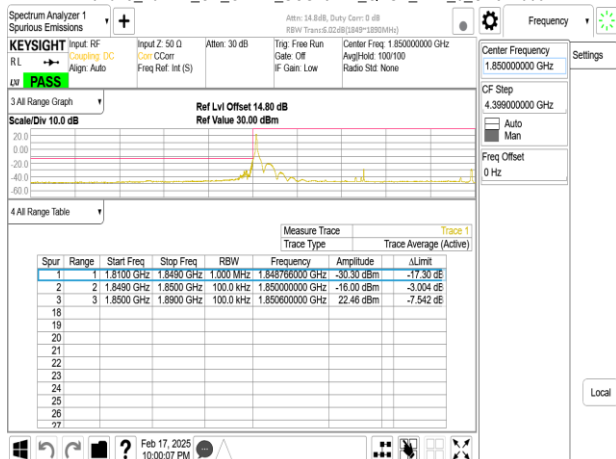
Band25_40MHz_CP_OFDM_SCS15kHz_QPSK_RB1_0_CH374000
