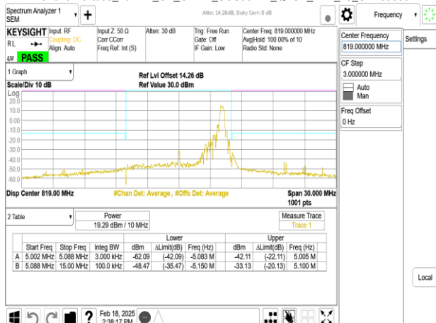
Band26-Part90s_10MHz_CP_OFDM_SCS30kHz_QPSK_RB1_23_CH163800
