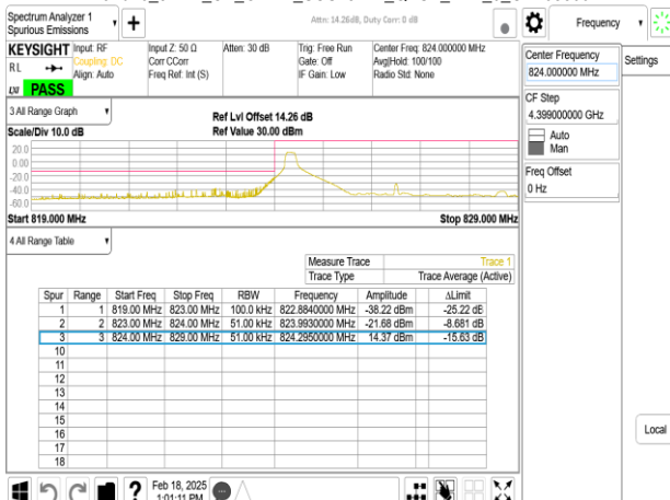
Band26_5MHz_CP_OFDM_SCS15kHz_QPSK_RB1_0_CH165300
