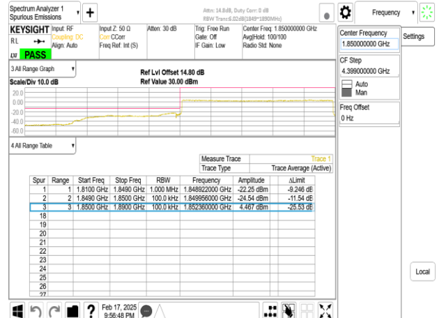
Band25_40MHz_DFT_s_OFDM_SCS15kHz_BPSK_RB216_0_CH374000
