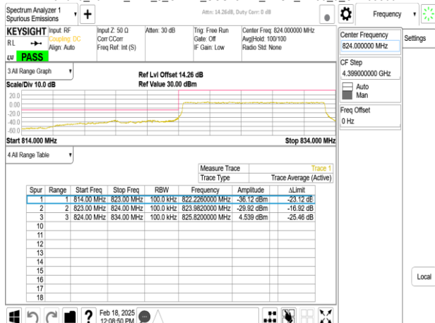
Band26_10MHz_DFT_s_OFDM_SCS15kHz_BPSK_RB1_51_CH168800
