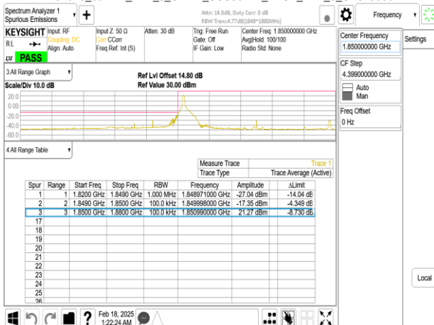
Band25_30MHz_DFT_s_OFDM_SCS30kHz_BPSK_RB1_0_CH373000
