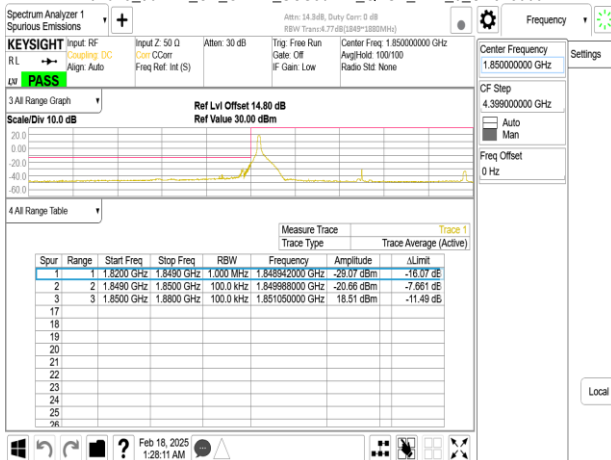
Band25_30MHz_CP_OFDM_SCS30kHz_QPSK_RB78_0_CH373000
