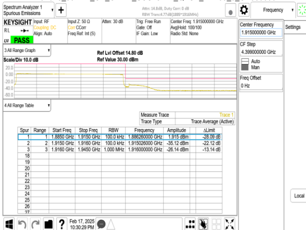
Band25_30MHz_CP_OFDM_SCS15kHz_QPSK_RB1_159_CH380000
