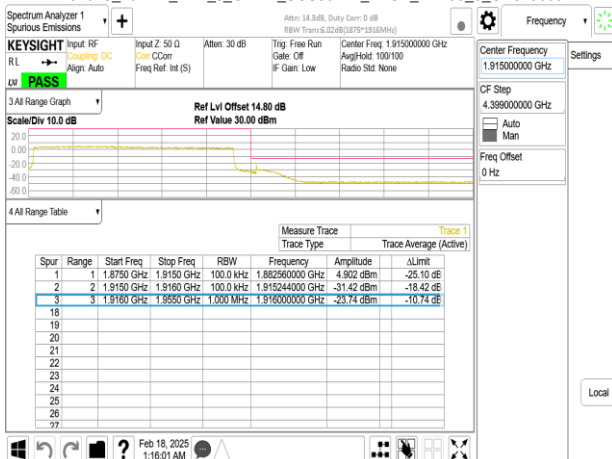
Band25_40MHz_DFT_s_OFDM_SCS30kHz_BPSK_RB100_0_CH379000
