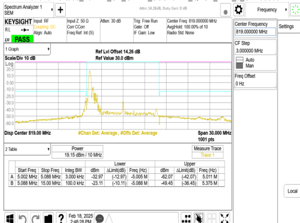
Band26-Part90s_10MHz_CP_OFDM_SCS15kHz_QPSK_RB1_51_CH163800
