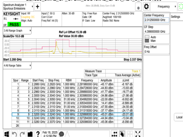
Band30_5MHz_CP_OFDM_SCS15kHz_QPSK_RB1_24_CH461500
