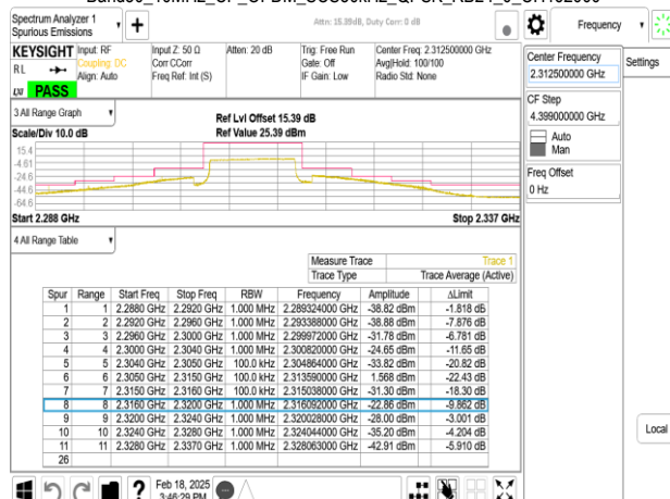
Band30_10MHz_CP_OFDM_SCS30kHz_QPSK_RB24_0_CH462000
