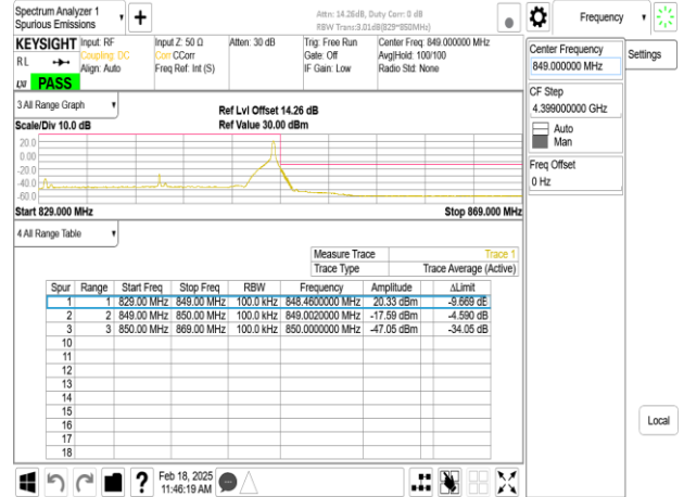
Band26_20MHz_DFT_s_OFDM_SCS30kHz_BPSK_RB1_0_CH166800
