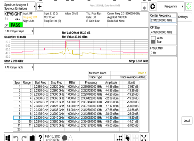
Band30_5MHz_DFT_s_OFDM_SCS15kHz_BPSK_RB25_0_CH462000
