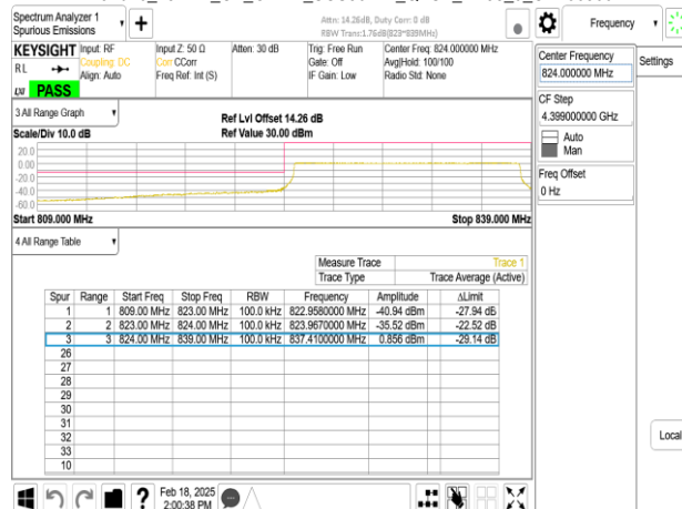
Band26_15MHz_CP_OFDM_SCS30kHz_QPSK_RB38_0_CH166300
