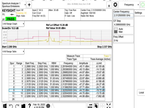
Band30_5MHz_CP_OFDM_SCS15kHz_QPSK_RB25_0_CH462000
