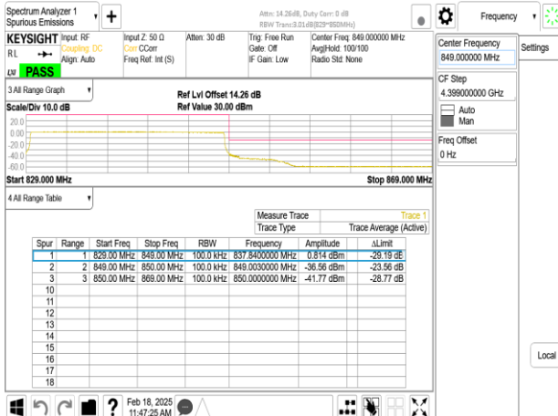
Band26_20MHz_CP_OFDM_SCS15kHz_QPSK_RB106_0_CH167800
