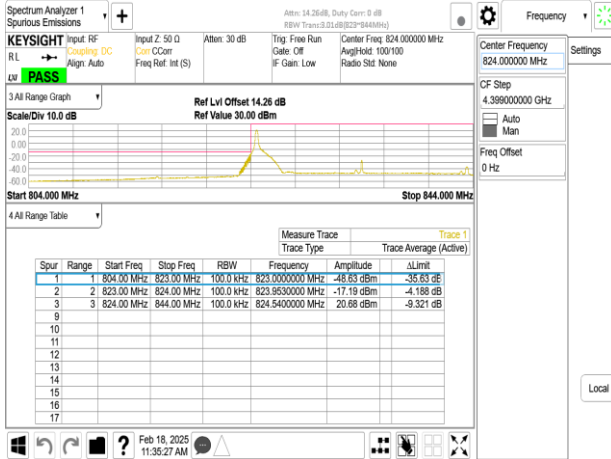
Band26_20MHz_CP_OFDM_SCS15kHz_QPSK_RB106_0_CH167800
