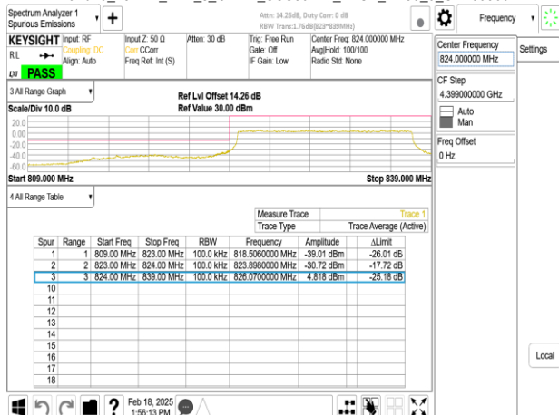
Band26_15MHz_DFT_s_OFDM_SCS30kHz_BPSK_RB1_37_CH168300
