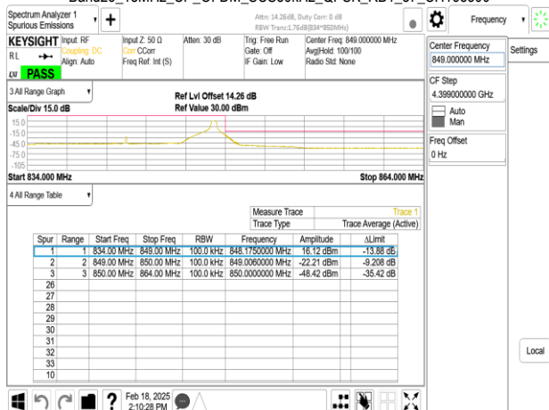
Band26_15MHz_CP_OFDM_SCS30kHz_QPSK_RB38_0_CH168300
