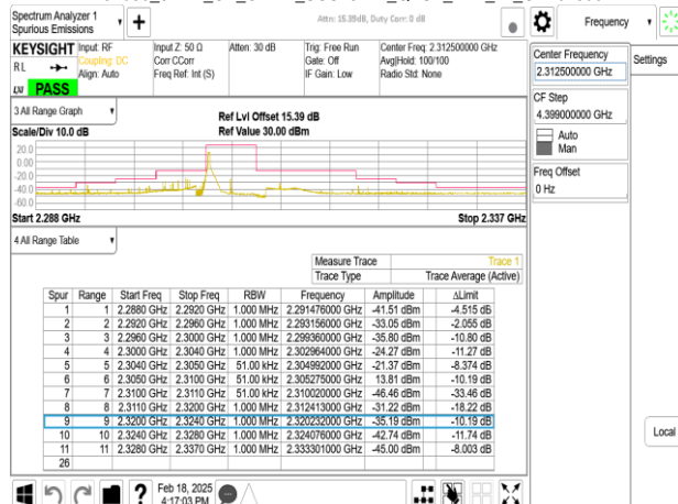
Band30_5MHz_CP_OFDM_SCS15kHz_QPSK_RB25_0_CH461500
