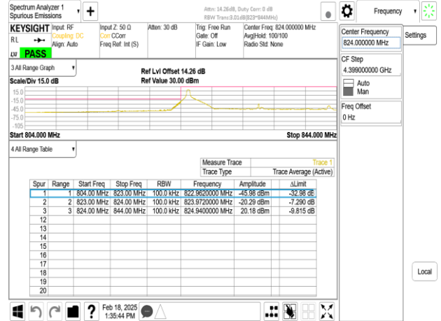
Band26_20MHz_DFT_s_OFDM_SCS30kHz_BPSK_RB50_0_CH166800
