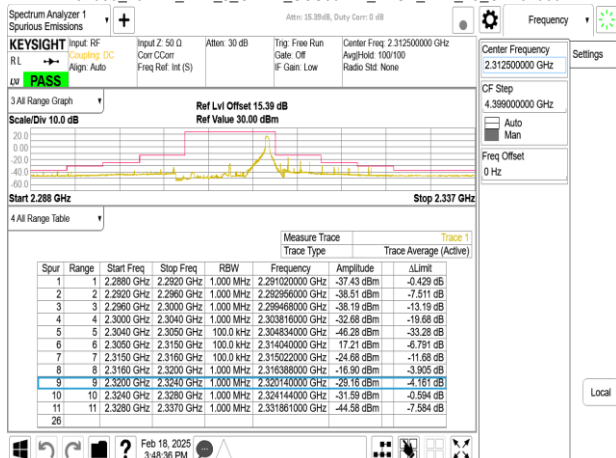
Band30_10MHz_DFT_s_OFDM_SCS30kHz_BPSK_RB24_0_CH462000
