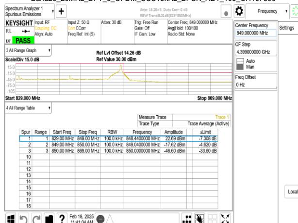
Band26_20MHz_DFT_s_OFDM_SCS15kHz_BPSK_RB1_105_CH167800
