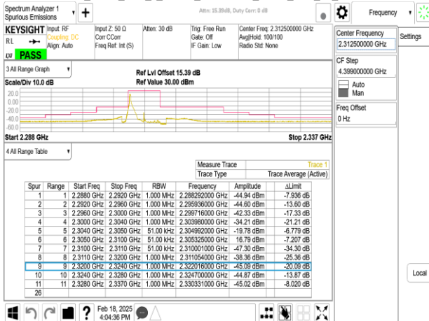
Band30_5MHz_DFT_s_OFDM_SCS15kHz_BPSK_RB25_0_CH461500
