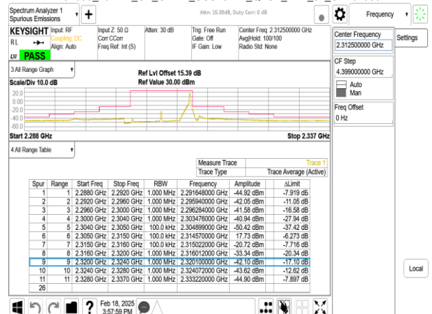
Band30_10MHz_CP_OFDM_SCS15kHz_QPSK_RB1_51_CH462000
