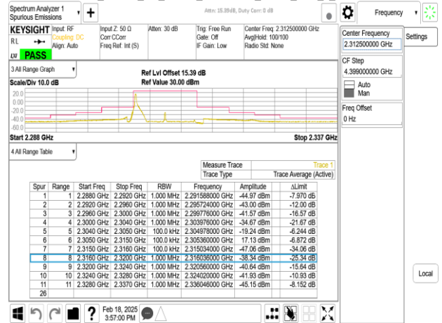
Band30_10MHz_CP_OFDM_SCS15kHz_QPSK_RB1_50_CH462000
