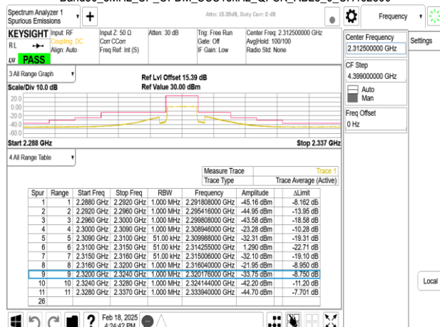
Band30_5MHz_CP_OFDM_SCS15kHz_QPSK_RB25_0_CH462500
