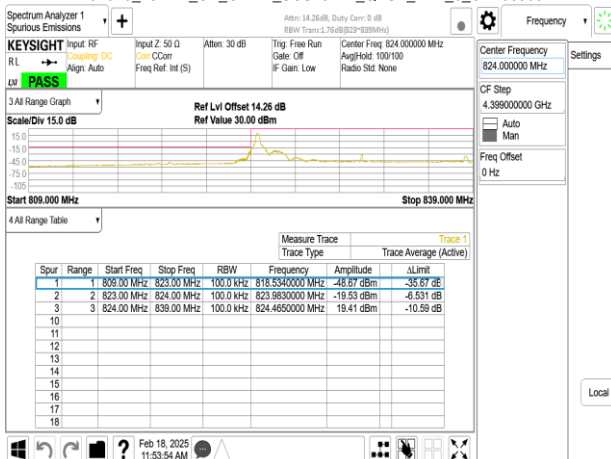
Band26_15MHz_CP_OFDM_SCS15kHz_QPSK_RB1_0_CH166300
