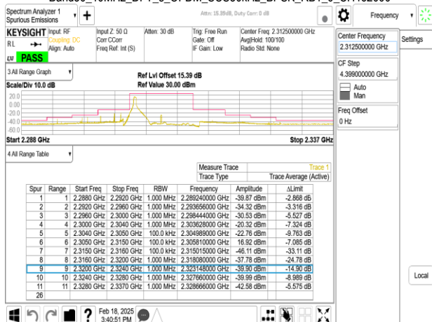
Band30_10MHz_DFT_s_OFDM_SCS30kHz_BPSK_RB1_23_CH462000
