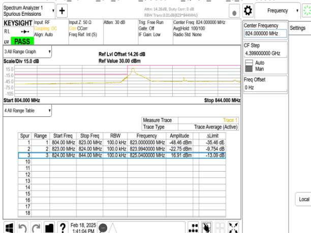
Band26_20MHz_CP_OFDM_SCS30kHz_QPSK_RB1_0_CH166800
