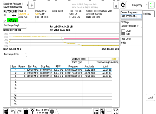
Band26_20MHz_CP_OFDM_SCS30kHz_QPSK_RB51_0_CH167800
