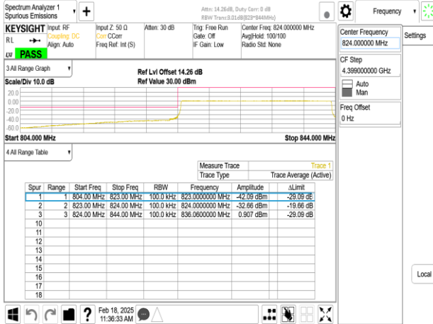
Band26_20MHz_CP_OFDM_SCS15kHz_QPSK_RB1_0_CH166800
