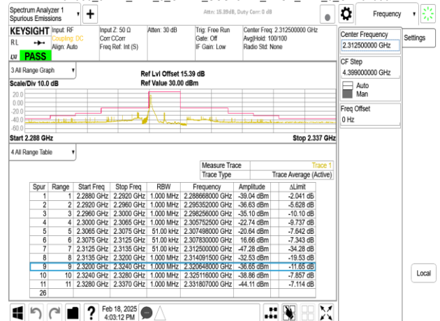
Band30_5MHz_DFT_s_OFDM_SCS15kHz_BPSK_RB1_24_CH462000
