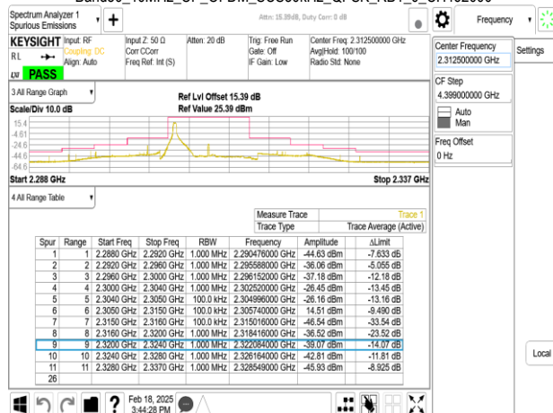
Band30_10MHz_CP_OFDM_SCS30kHz_QPSK_RB1_23_CH462000
