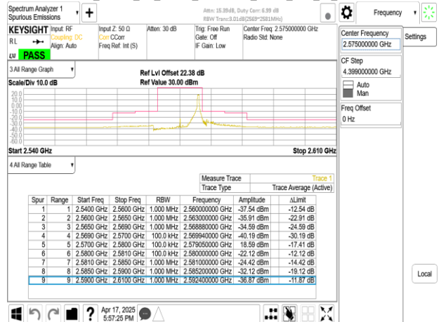
Band38_10MHz_CP_OFDM_SCS30kHz_QPSK_RB24_0_CH515000
