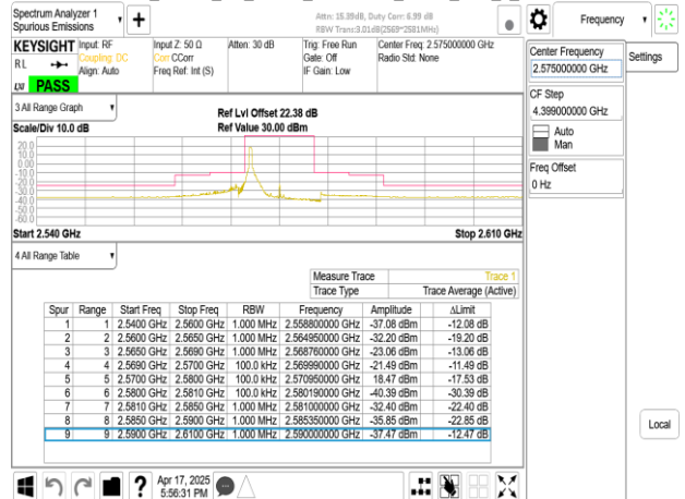
Band38_10MHz_CP_OFDM_SCS30kHz_QPSK_RB1_23_CH515000
