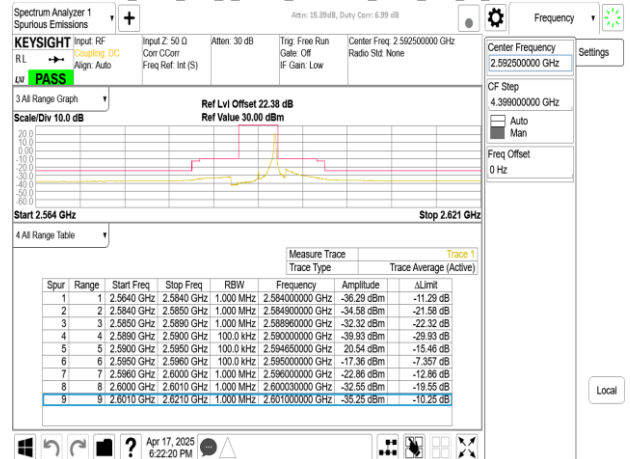
Band38_5MHz_DFT_s_OFDM_SCS15kHz_BPSK_RB25_0_CH518500
