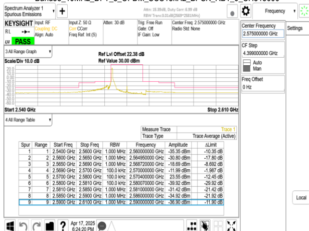
Band38_10MHz_DFT_s_OFDM_SCS15kHz_BPSK_RB1_51_CH515000
