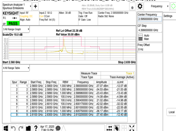
Band38_10MHz_CP_OFDM_SCS15kHz_QPSK_RB1_51_CH519000
