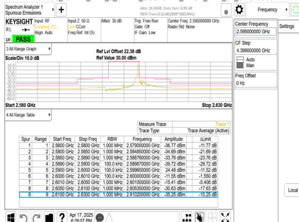
Band38_10MHz_DFT_s_OFDM_SCS15kHz_BPSK_RB50_0_CH519000
