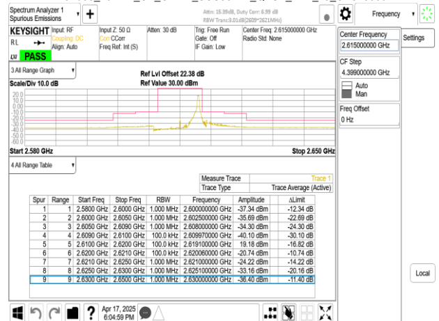
Band38_10MHz_CP_OFDM_SCS30kHz_QPSK_RB24_0_CH523000
