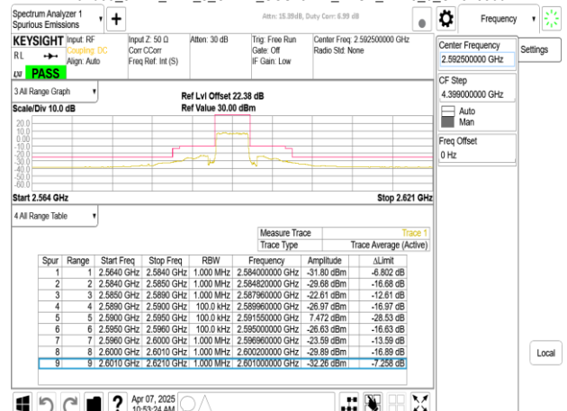
Band38_5MHz_DFT_s_OFDM_SCS15kHz_BPSK_RB25_0_CH518500
