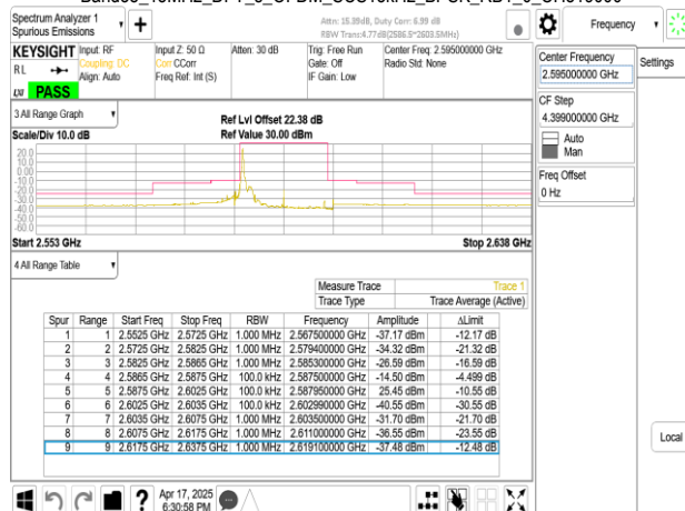
Band38_15MHz_DFT_s_OFDM_SCS15kHz_BPSK_RB1_78_CH519000
