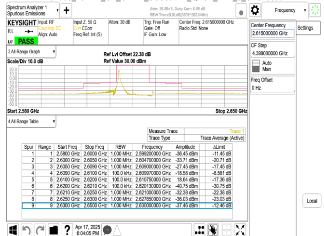
Band38_10MHz_CP_OFDM_SCS30kHz_QPSK_RB1_23_CH523000
