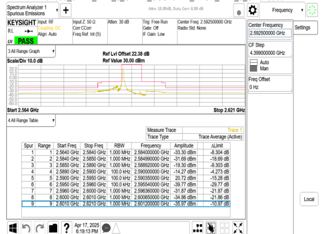
Band38_5MHz_DFT_s_OFDM_SCS15kHz_BPSK_RB1_24_CH518500
