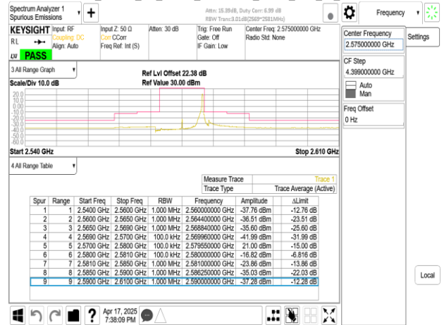
Band38_10MHz_CP_OFDM_SCS15kHz_QPSK_RB52_0_CH515000
