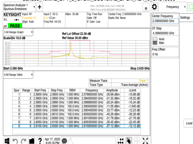
Band38_10MHz_DFT_s_OFDM_SCS15kHz_BPSK_RB1_51_CH519000
