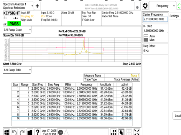
Band38_10MHz_CP_OFDM_SCS15kHz_QPSK_RB52_0_CH523000
