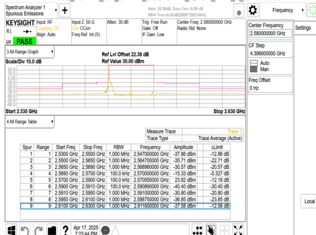
Band38_20MHz_CP_OFDM_SCS15kHz_QPSK_RB1_105_CH516000
