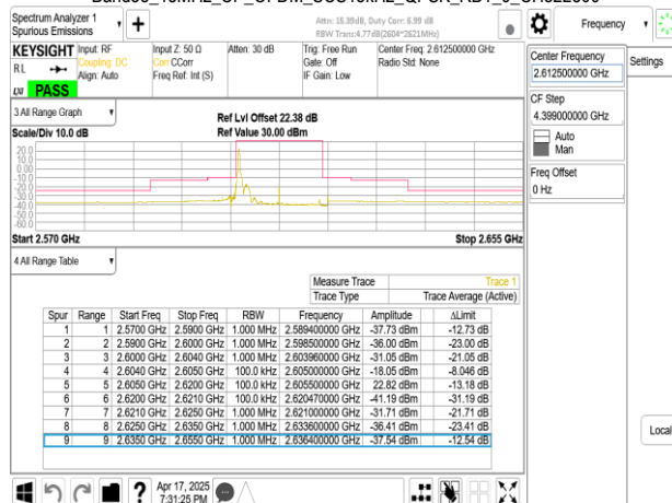
Band38_15MHz_CP_OFDM_SCS15kHz_QPSK_RB1_78_CH522500
