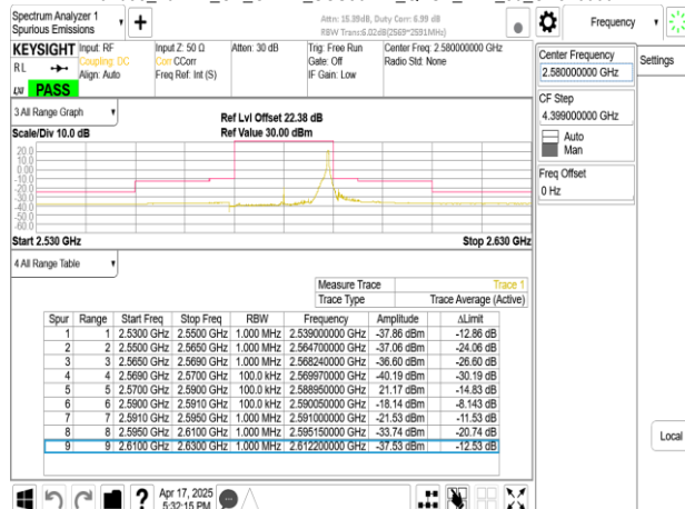
Band38_20MHz_CP_OFDM_SCS30kHz_QPSK_RB51_0_CH516000
