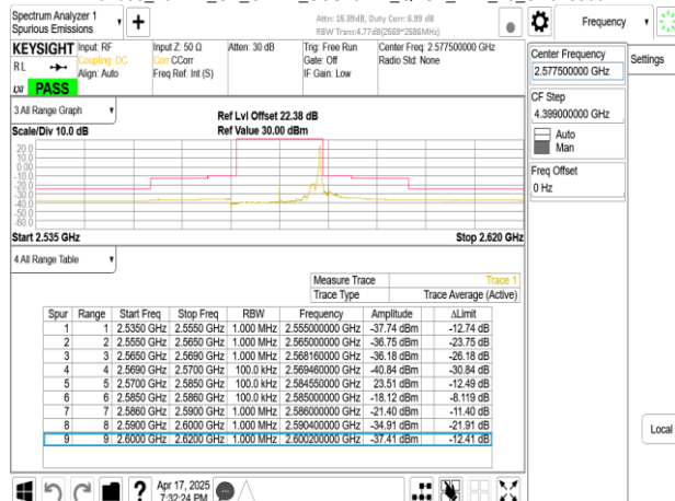
Band38_15MHz_CP_OFDM_SCS15kHz_QPSK_RB79_0_CH515500
