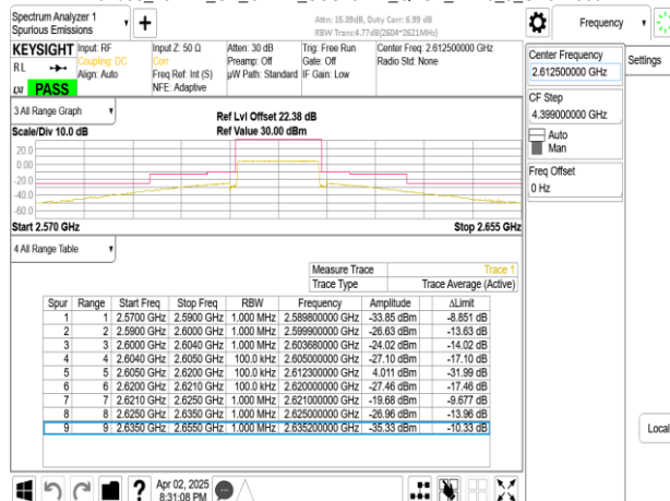
Band38_15MHz_CP_OFDM_SCS15kHz_QPSK_RB79_0_CH522500
