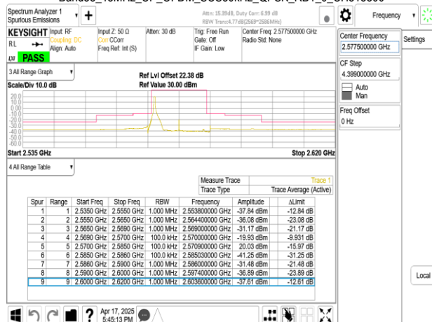
Band38_15MHz_CP_OFDM_SCS30kHz_QPSK_RB1_37_CH515500
