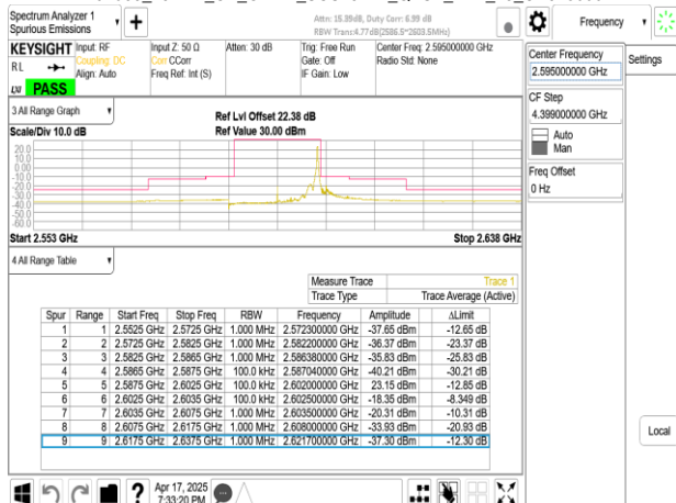
Band38_15MHz_CP_OFDM_SCS15kHz_QPSK_RB79_0_CH519000
