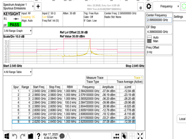
Band38_20MHz_DFT_s_OFDM_SCS15kHz_BPSK_RB1_105_CH519000
