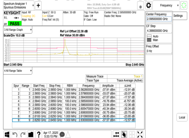
Band38_20MHz_DFT_s_OFDM_SCS30kHz_BPSK_RB1_50_CH519000
