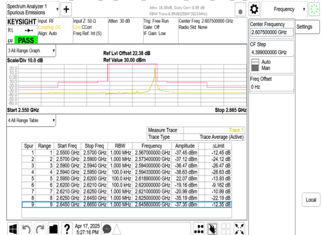
Band38_25MHz_CP_OFDM_SCS30kHz_QPSK_RB65_0_CH521500
