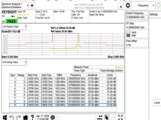
Band38_30MHz_CP_OFDM_SCS15kHz_QPSK_RB1_159_CH519000
