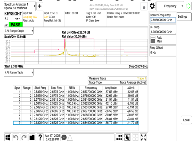
Band38_25MHz_DFT_s_OFDM_SCS15kHz_BPSK_RB1_132_CH519000
