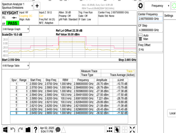
Band38_25MHz_DFT_s_OFDM_SCS15kHz_BPSK_RB1_0_CH521500
