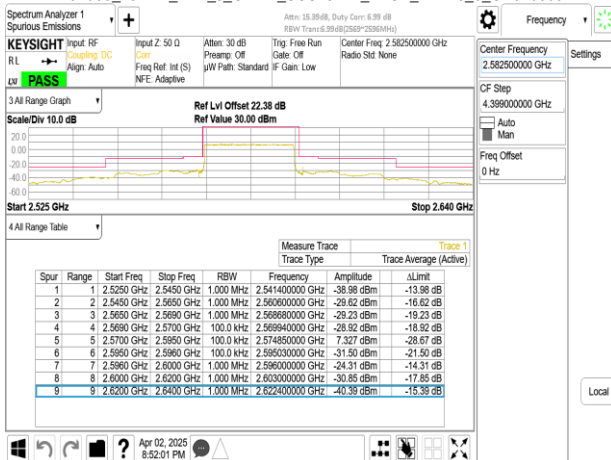
Band38_25MHz_DFT_s_OFDM_SCS15kHz_BPSK_RB1_0_CH516500
