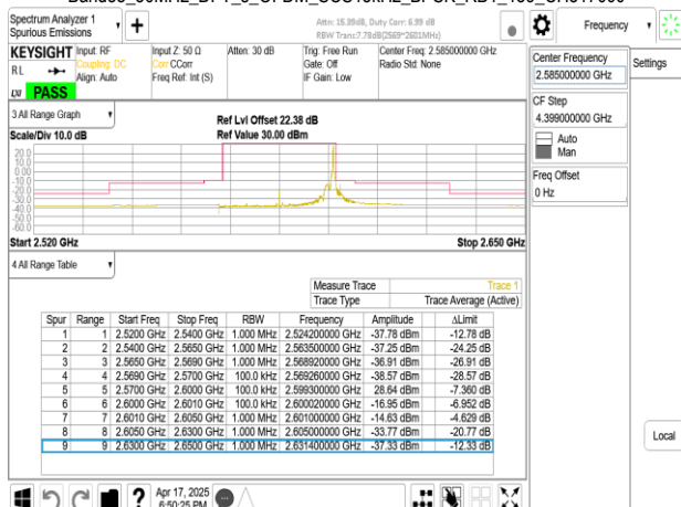
Band38_30MHz_DFT_s_OFDM_SCS15kHz_BPSK_RB1_159_CH517000
