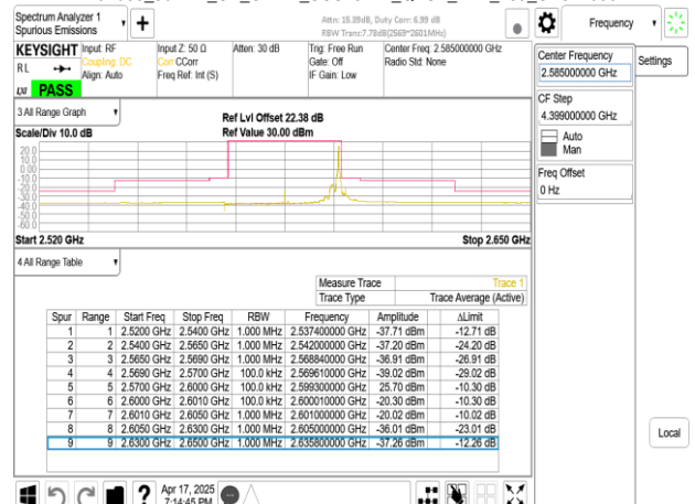
Band38_30MHz_CP_OFDM_SCS15kHz_QPSK_RB1_159_CH517000
