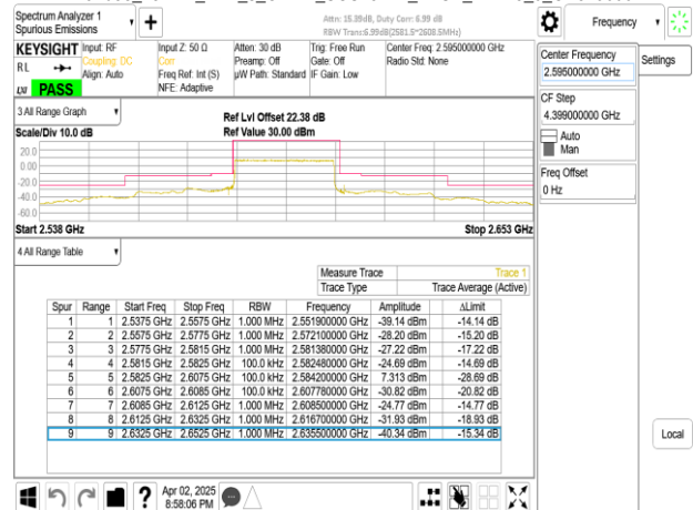
Band38_25MHz_DFT_s_OFDM_SCS15kHz_BPSK_RB1_0_CH519000
