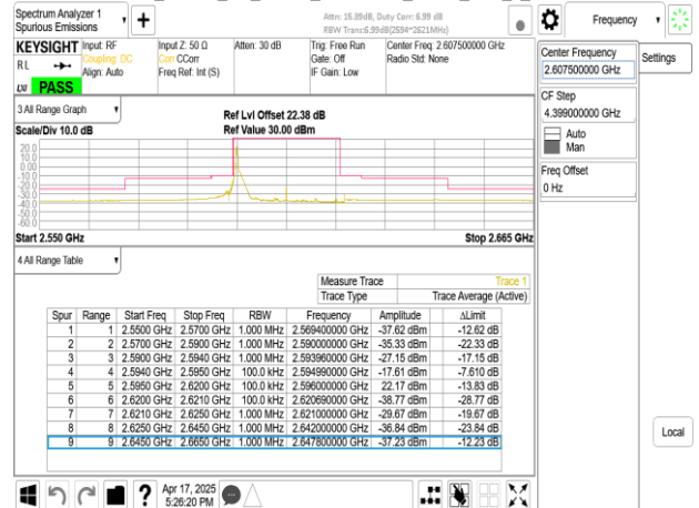
Band38_25MHz_CP_OFDM_SCS30kHz_QPSK_RB1_64_CH521500
