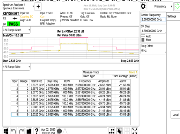
Band38_25MHz_CP_OFDM_SCS15kHz_QPSK_RB1_0_CH519000
