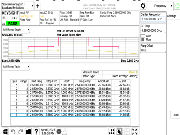
Band38_30MHz_CP_OFDM_SCS15kHz_QPSK_RB1_0_CH519000
