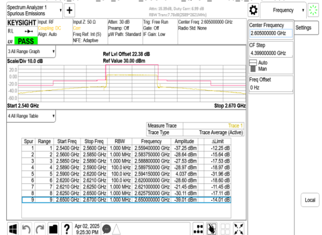
Band38_30MHz_CP_OFDM_SCS15kHz_QPSK_RB1_0_CH521000
