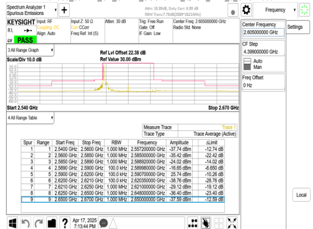
Band38_30MHz_CP_OFDM_SCS15kHz_QPSK_RB1_159_CH521000
