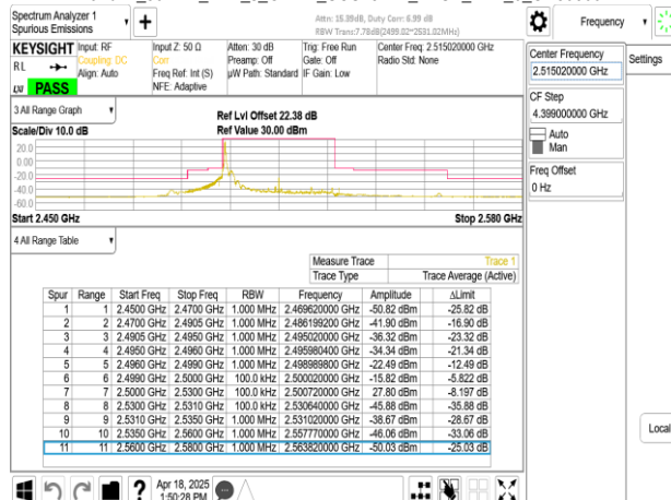
Band41_30MHz_DFT_s_OFDM_SCS15kHz_BPSK_RB1_159_CH503004
