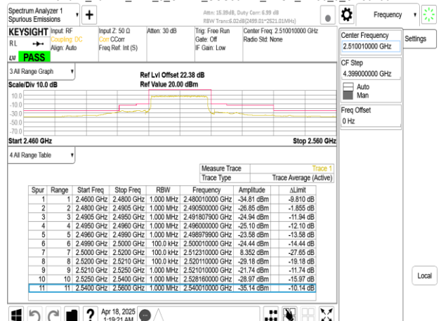
Band41_20MHz_DFT_s_OFDM_SCS30kHz_BPSK_RB50_0_CH502002
