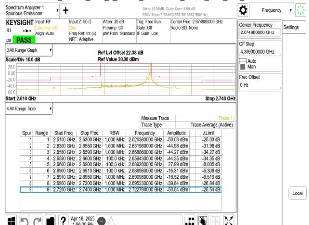
Band41_30MHz_DFT_s_OFDM_SCS15kHz_BPSK_RB1_159_CH534996
