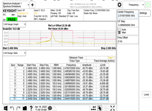
Band41_20MHz_DFT_s_OFDM_SCS30kHz_BPSK_RB1_50_CH502002
