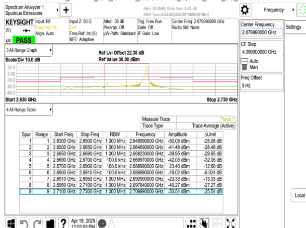
Band41_20MHz_CP_OFDM_SCS30kHz_QPSK_RB51_0_CH535998
