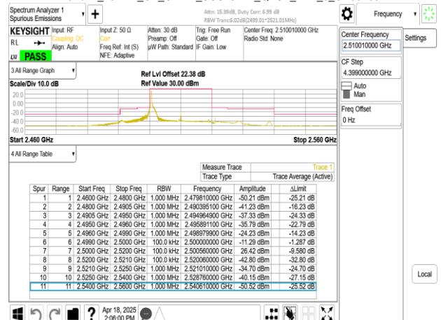
Band41_20MHz_CP_OFDM_SCS15kHz_QPSK_RB1_105_CH502002
