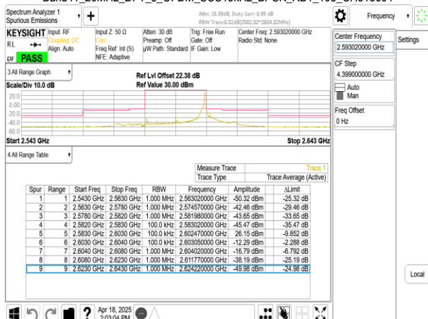
Band41_20MHz_DFT_s_OFDM_SCS15kHz_BPSK_RB1_105_CH518604
