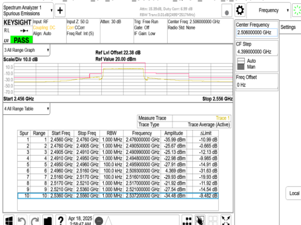
Band41_20MHz_CP_OFDM_SCS30kHz_QPSK_RB51_0_CH501204
