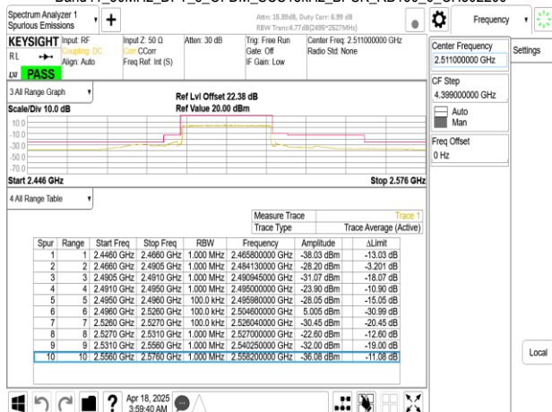
Band41_30MHz_DFT_s_OFDM_SCS15kHz_BPSK_RB1_0_CH502200
