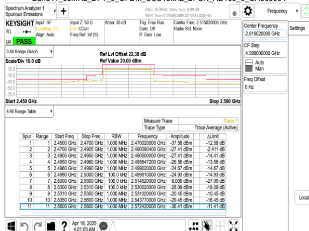
Band41_30MHz_DFT_s_OFDM_SCS15kHz_BPSK_RB1_0_CH503004
