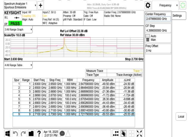
Band41_20MHz_CP_OFDM_SCS15kHz_QPSK_RB1_105_CH535998
