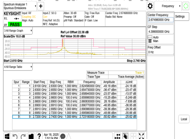
Band41_30MHz_DFT_s_OFDM_SCS15kHz_BPSK_RB1_159_CH534996
