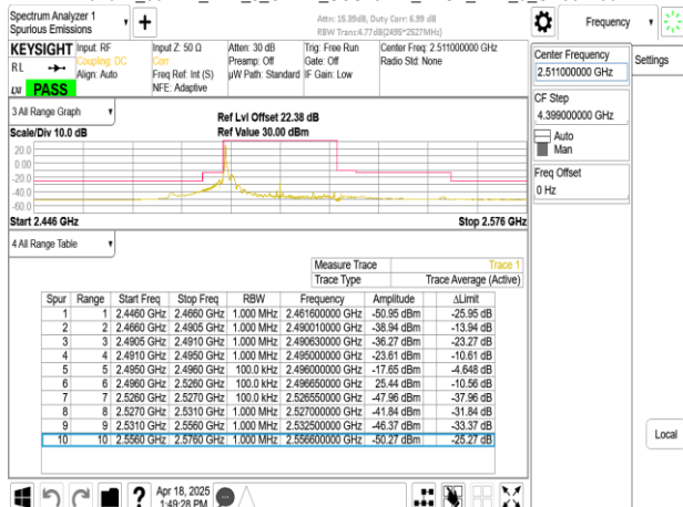
Band41_30MHz_DFT_s_OFDM_SCS15kHz_BPSK_RB1_159_CH502200
