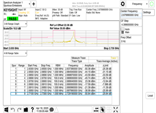
Band41_20MHz_DFT_s_OFDM_SCS30kHz_BPSK_RB50_0_CH535998
