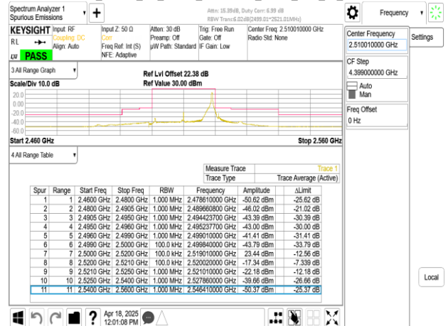
Band41_20MHz_CP_OFDM_SCS30kHz_QPSK_RB51_0_CH502002
