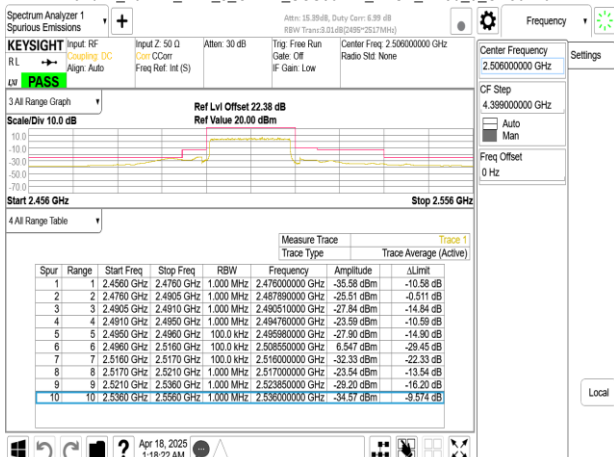
Band41_20MHz_DFT_s_OFDM_SCS30kHz_BPSK_RB50_0_CH501204
