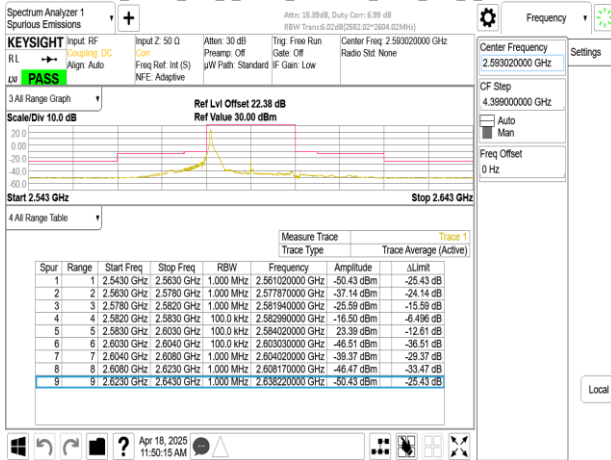
Band41_20MHz_DFT_s_OFDM_SCS30kHz_BPSK_RB1_50_CH518604
