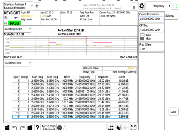
Band41_20MHz_CP_OFDM_SCS30kHz_QPSK_RB51_0_CH502002
