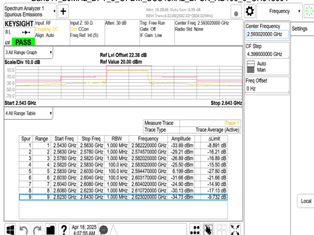
Band41_20MHz_DFT_s_OFDM_SCS15kHz_BPSK_RB1_0_CH518604
