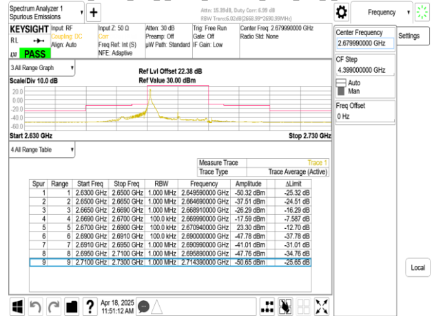
Band41_20MHz_DFT_s_OFDM_SCS30kHz_BPSK_RB1_50_CH535998
