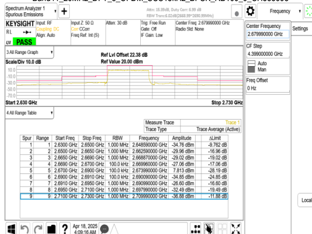
Band41_20MHz_DFT_s_OFDM_SCS15kHz_BPSK_RB1_0_CH535998
