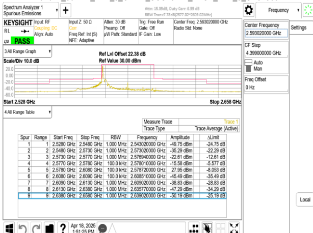
Band41_30MHz_DFT_s_OFDM_SCS15kHz_BPSK_RB1_159_CH518604
