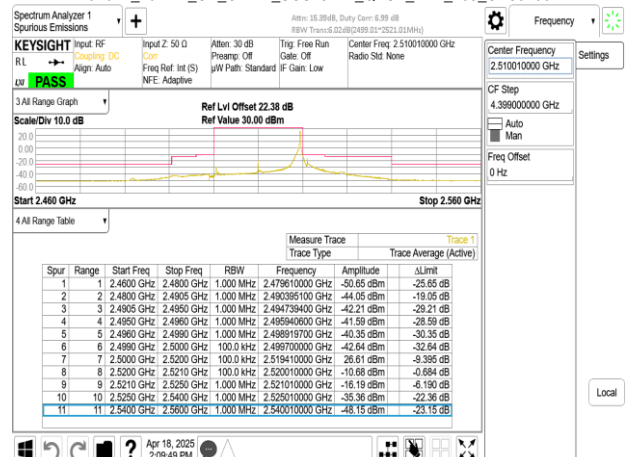
Band41_20MHz_CP_OFDM_SCS15kHz_QPSK_RB1_105_CH502002
