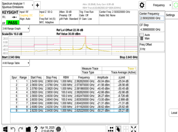
Band41_20MHz_CP_OFDM_SCS15kHz_QPSK_RB1_105_CH518604
