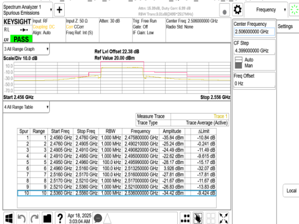
Band41_20MHz_CP_OFDM_SCS15kHz_QPSK_RB1_0_CH501204
