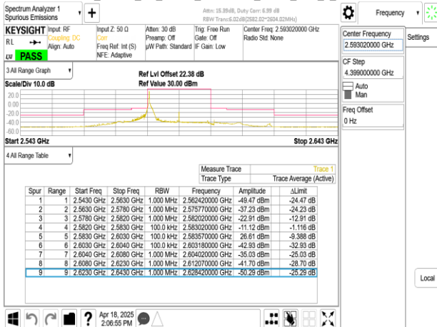
Band41_20MHz_CP_OFDM_SCS15kHz_QPSK_RB1_105_CH518604
