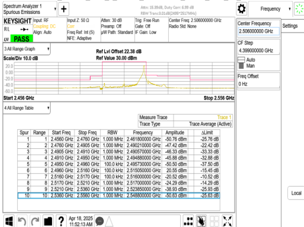
Band41_20MHz_DFT_s_OFDM_SCS30kHz_BPSK_RB50_0_CH501204
