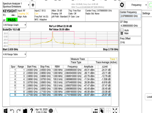
Band41_20MHz_DFT_s_OFDM_SCS15kHz_BPSK_RB1_105_CH535998
