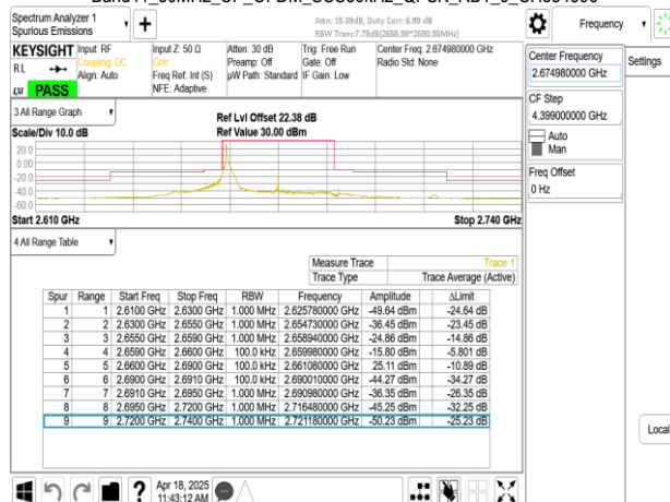
Band41_30MHz_CP_OFDM_SCS30kHz_QPSK_RB1_77_CH534996
