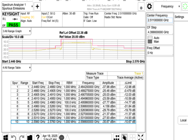
Band41_30MHz_CP_OFDM_SCS30kHz_QPSK_RB78_0_CH502200
