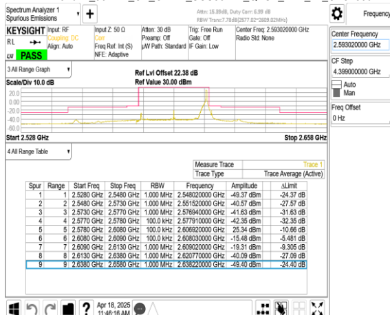
Band41_30MHz_CP_OFDM_SCS30kHz_QPSK_RB78_0_CH518604
