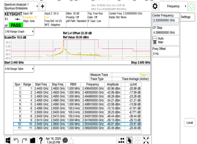
Band41_40MHz_DFT_s_OFDM_SCS15kHz_BPSK_RB1_215_CH504000
