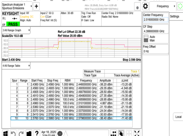
Band41_40MHz_DFT_s_OFDM_SCS15kHz_BPSK_RB216_0_CH503202
