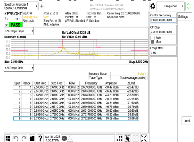
Band41_40MHz_DFT_s_OFDM_SCS15kHz_BPSK_RB1_215_CH534000
