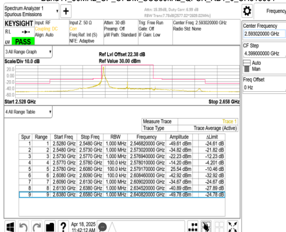
Band41_30MHz_CP_OFDM_SCS30kHz_QPSK_RB1_77_CH518604
