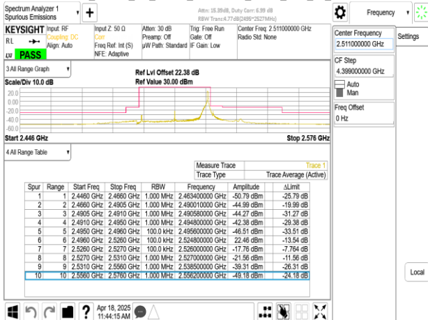
Band41_30MHz_CP_OFDM_SCS30kHz_QPSK_RB78_0_CH502200
