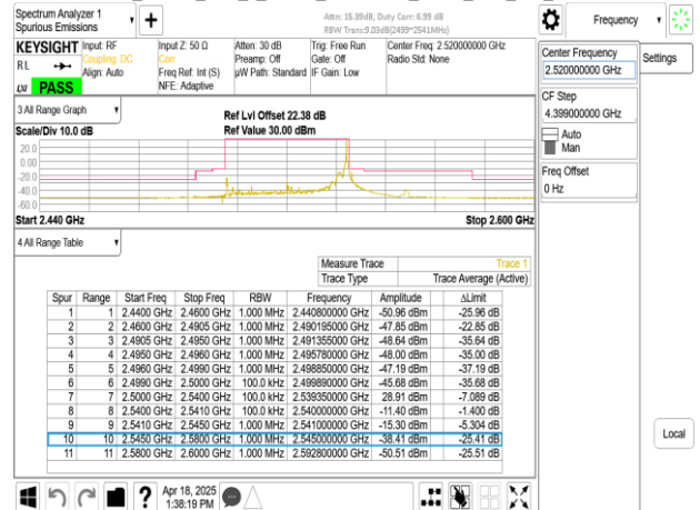
Band41_40MHz_DFT_s_OFDM_SCS15kHz_BPSK_RB216_0_CH504000
