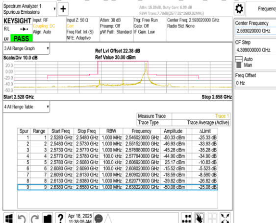
Band41_30MHz_DFT_s_OFDM_SCS30kHz_BPSK_RB75_0_CH518604
