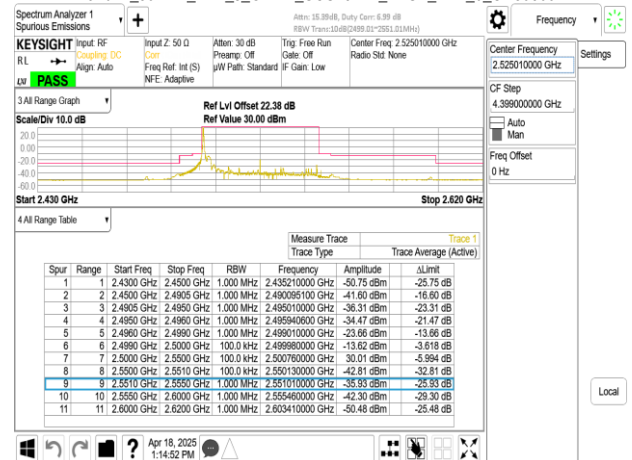
Band41_50MHz_DFT_s_OFDM_SCS15kHz_BPSK_RB1_269_CH505002
