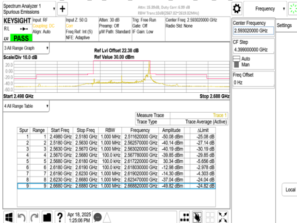
Band41_50MHz_CP_OFDM_SCS15kHz_QPSK_RB270_0_CH518604
