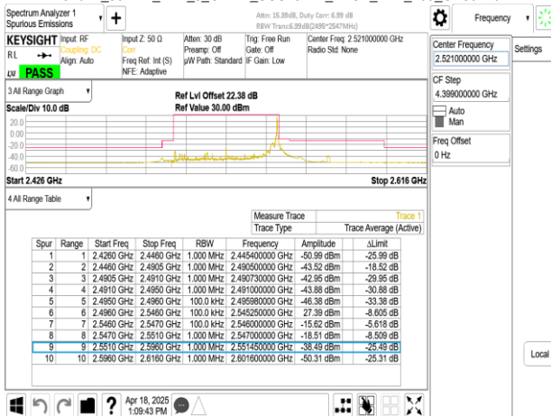
Band41_50MHz_DFT_s_OFDM_SCS15kHz_BPSK_RB270_0_CH504204
