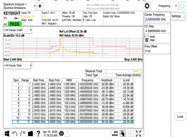
Band41_40MHz_DFT_s_OFDM_SCS30kHz_BPSK_RB1_105_CH504000
