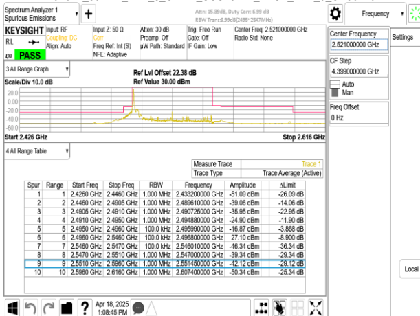
Band41_50MHz_DFT_s_OFDM_SCS15kHz_BPSK_RB1_269_CH504204
