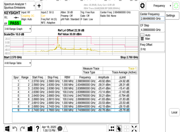
Band41_50MHz_CP_OFDM_SCS15kHz_QPSK_RB1_269_CH532998
