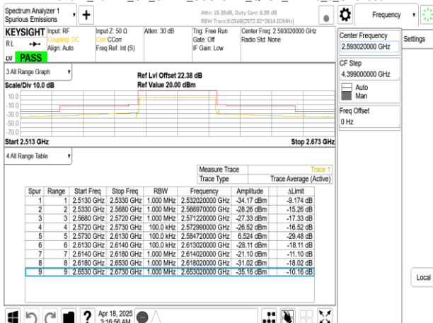
Band41_40MHz_CP_OFDM_SCS15kHz_QPSK_RB216_0_CH518604
