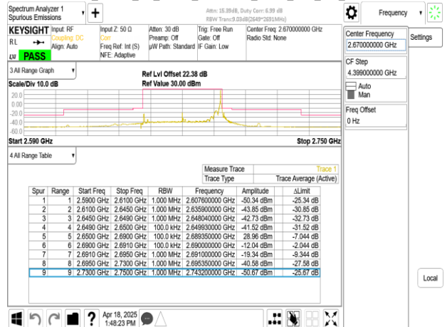
Band41_40MHz_CP_OFDM_SCS15kHz_QPSK_RB216_0_CH534000
