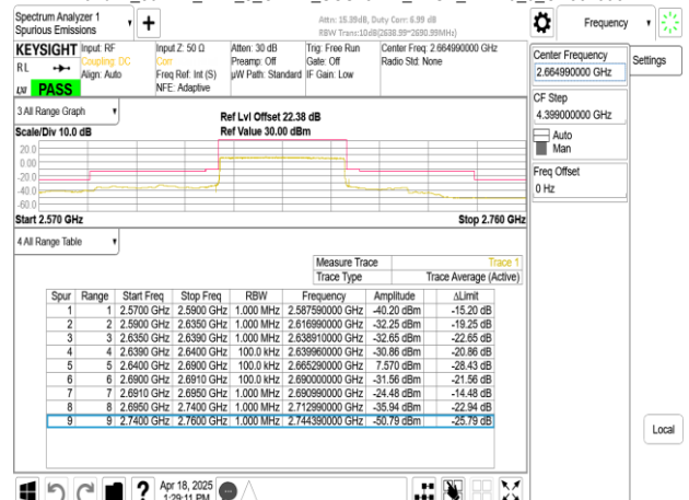
Band41_50MHz_DFT_s_OFDM_SCS15kHz_BPSK_RB270_0_CH532998
