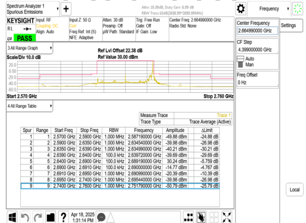
Band41_50MHz_CP_OFDM_SCS15kHz_QPSK_RB270_0_CH532998
