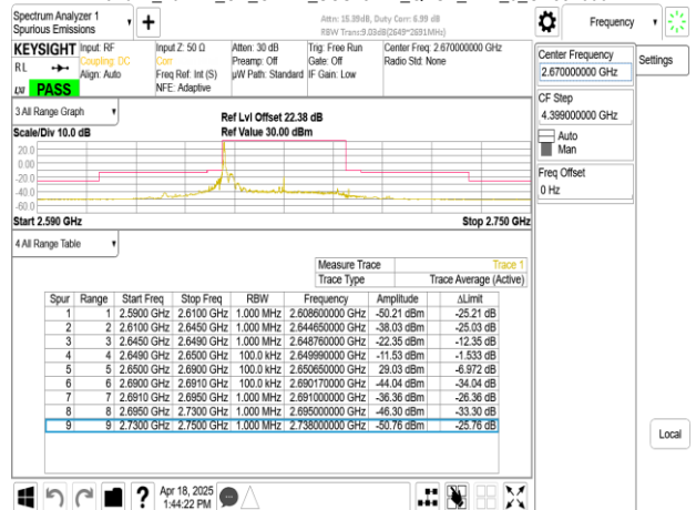
Band41_40MHz_CP_OFDM_SCS15kHz_QPSK_RB1_215_CH534000
