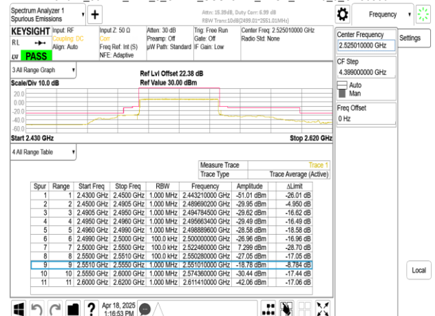
Band41_50MHz_DFT_s_OFDM_SCS15kHz_BPSK_RB270_0_CH505002
