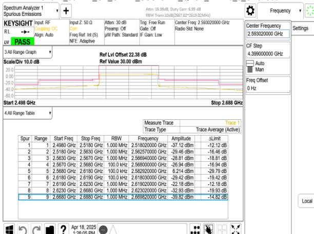
Band41_50MHz_CP_OFDM_SCS15kHz_QPSK_RB270_0_CH518604
