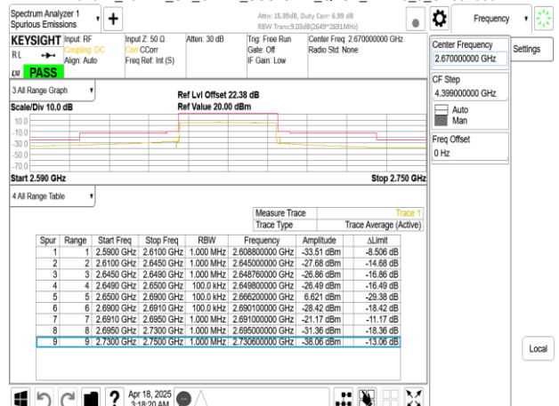
Band41_40MHz_CP_OFDM_SCS15kHz_QPSK_RB216_0_CH534000
