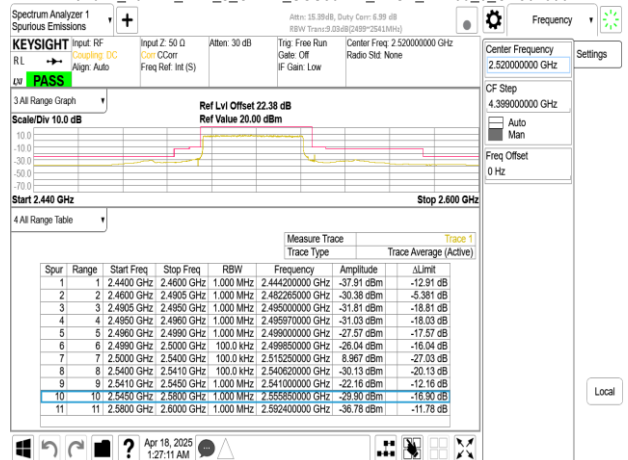
Band41_40MHz_DFT_s_OFDM_SCS30kHz_BPSK_RB1_0_CH504000
