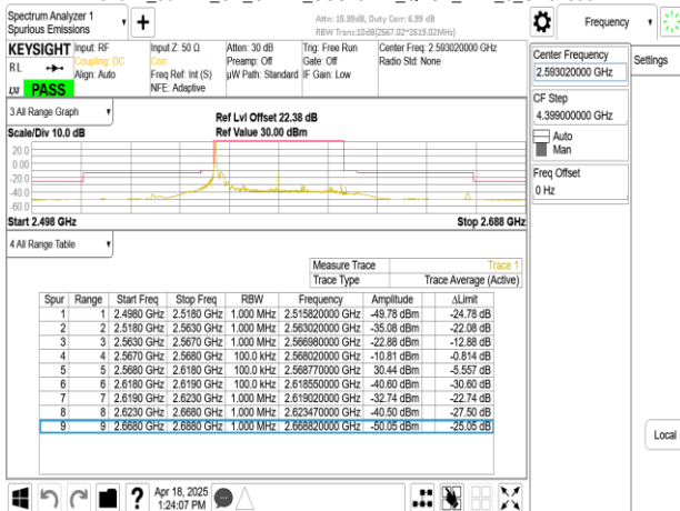
Band41_50MHz_CP_OFDM_SCS15kHz_QPSK_RB1_269_CH518604
