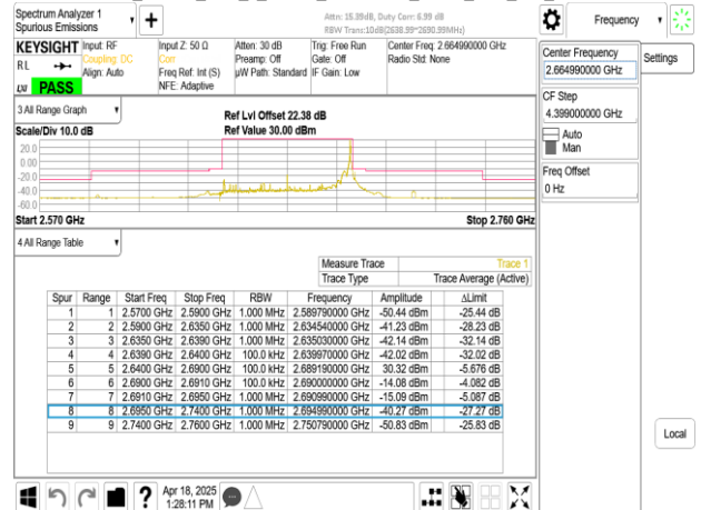
Band41_50MHz_DFT_s_OFDM_SCS15kHz_BPSK_RB270_0_CH532998
