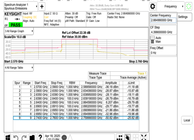
Band41_50MHz_CP_OFDM_SCS15kHz_QPSK_RB270_0_CH532998
