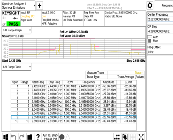
Band41_50MHz_CP_OFDM_SCS15kHz_QPSK_RB270_0_CH504204
