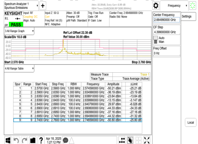
Band41_50MHz_DFT_s_OFDM_SCS15kHz_BPSK_RB1_269_CH532998
