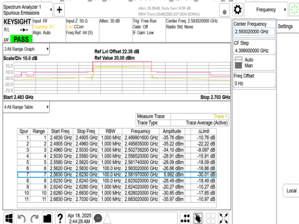
Band41_60MHz_CP_OFDM_SCS30kHz_QPSK_RB1_0_CH518604
