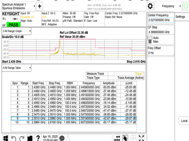
Band41_50MHz_DFT_s_OFDM_SCS30kHz_BPSK_RB1_132_CH504204
