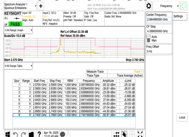
Band41_50MHz_DFT_s_OFDM_SCS30kHz_BPSK_RB1_132_CH532998
