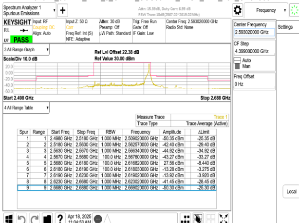
Band41_50MHz_DFT_s_OFDM_SCS30kHz_BPSK_RB1_132_CH518604
