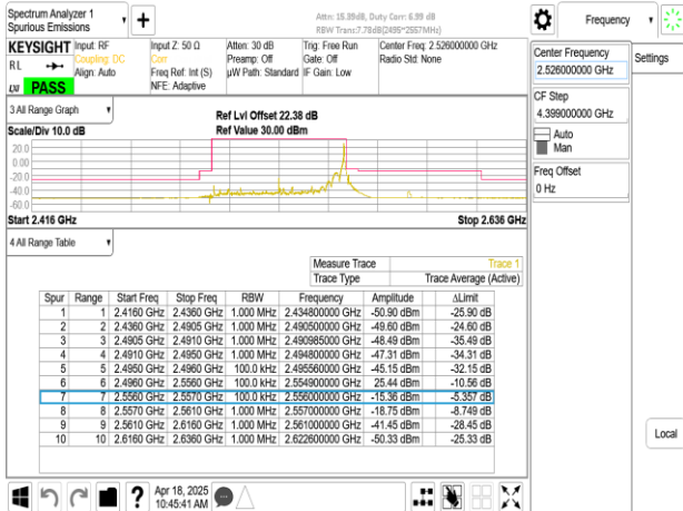
Band41_60MHz_DFT_s_OFDM_SCS30kHz_BPSK_RB1_161_CH505200
