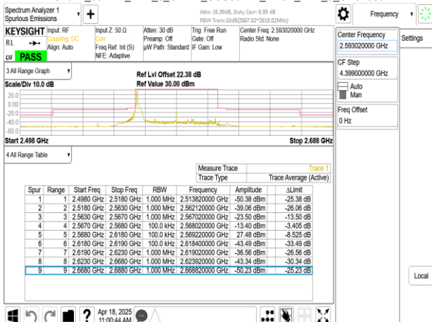
Band41_50MHz_DFT_s_OFDM_SCS30kHz_BPSK_RB1_132_CH518604
