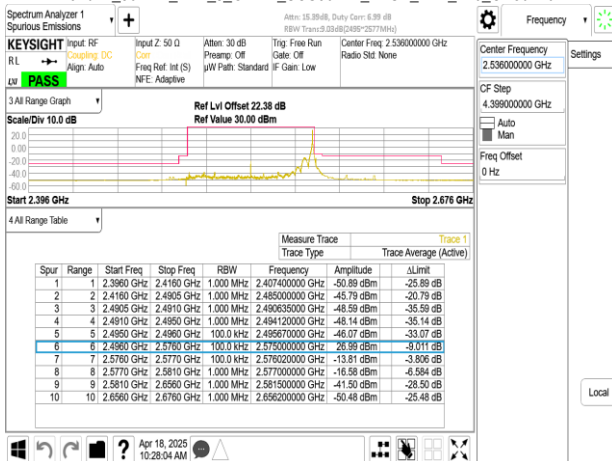
Band41_80MHz_DFT_s_OFDM_SCS30kHz_BPSK_RB216_0_CH507204
