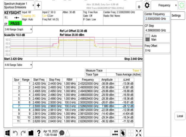
Band41_60MHz_DFT_s_OFDM_SCS30kHz_BPSK_RB1_0_CH506004
