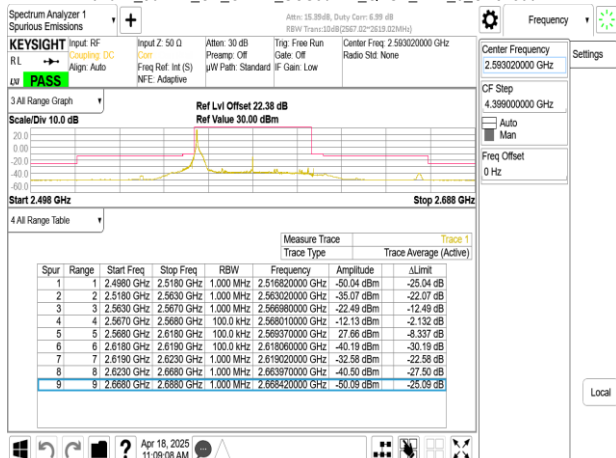
Band41_50MHz_CP_OFDM_SCS30kHz_QPSK_RB1_132_CH518604
