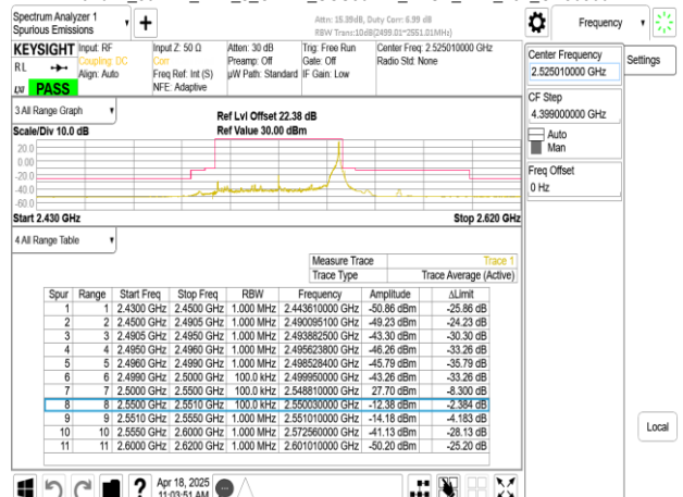
Band41_50MHz_DFT_s_OFDM_SCS30kHz_BPSK_RB1_132_CH505002
