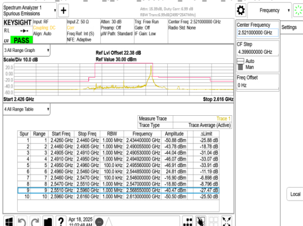
Band41_50MHz_DFT_s_OFDM_SCS30kHz_BPSK_RB1_132_CH504204
