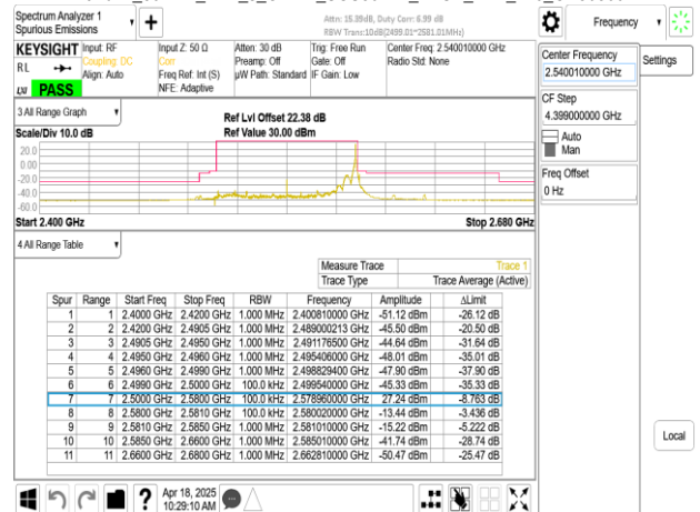
Band41_80MHz_DFT_s_OFDM_SCS30kHz_BPSK_RB216_0_CH508002
