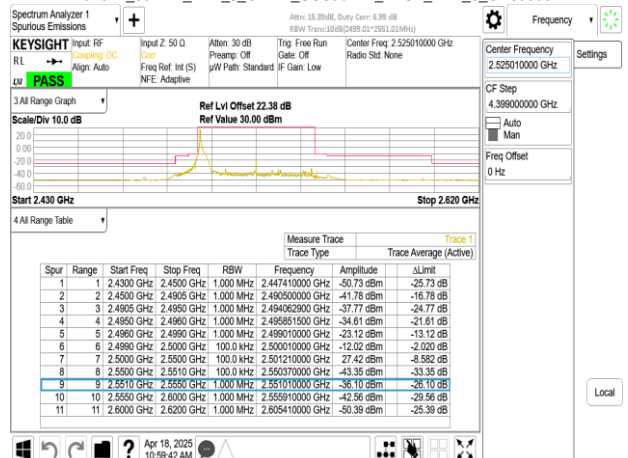
Band41_50MHz_DFT_s_OFDM_SCS30kHz_BPSK_RB1_132_CH505002
