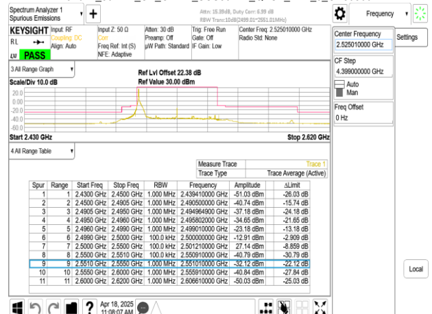
Band41_50MHz_CP_OFDM_SCS30kHz_QPSK_RB1_132_CH505002
