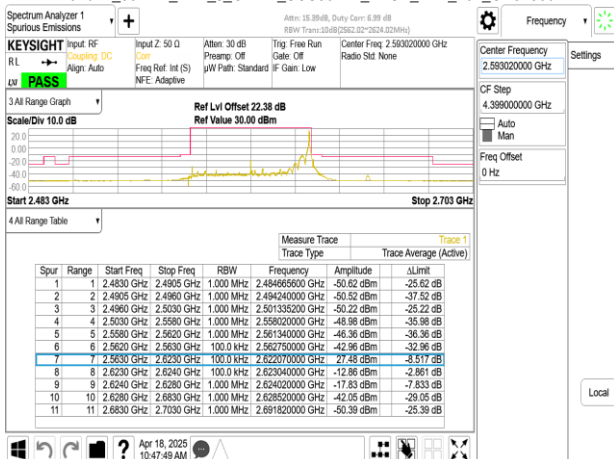
Band41_60MHz_DFT_s_OFDM_SCS30kHz_BPSK_RB1_161_CH518604
