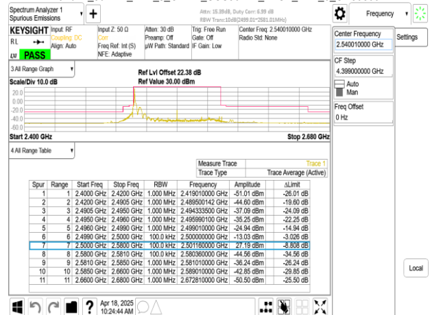
Band41_80MHz_DFT_s_OFDM_SCS30kHz_BPSK_RB1_216_CH508002
