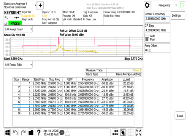
Band41_60MHz_DFT_s_OFDM_SCS30kHz_BPSK_RB1_161_CH531996
