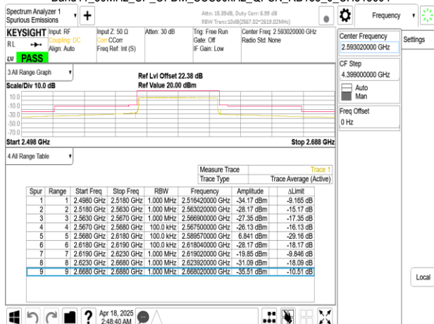
Band41_50MHz_CP_OFDM_SCS30kHz_QPSK_RB1_0_CH518604
