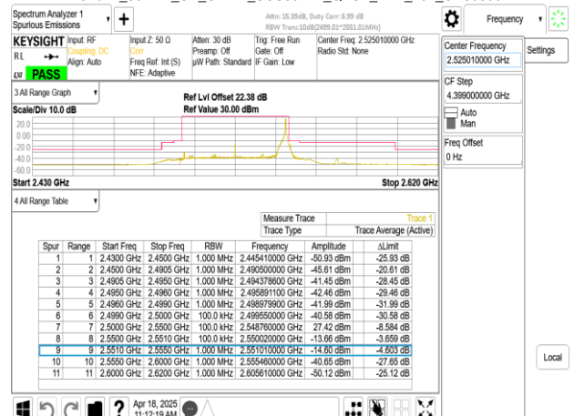
Band41_50MHz_CP_OFDM_SCS30kHz_QPSK_RB1_132_CH505002
