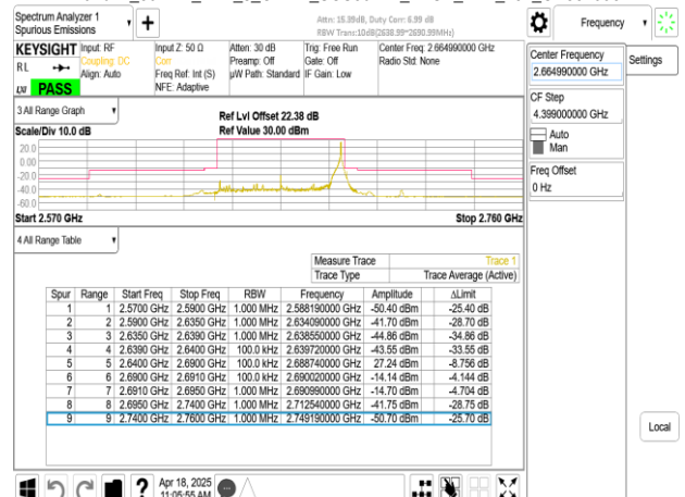
Band41_50MHz_DFT_s_OFDM_SCS30kHz_BPSK_RB1_132_CH532998
