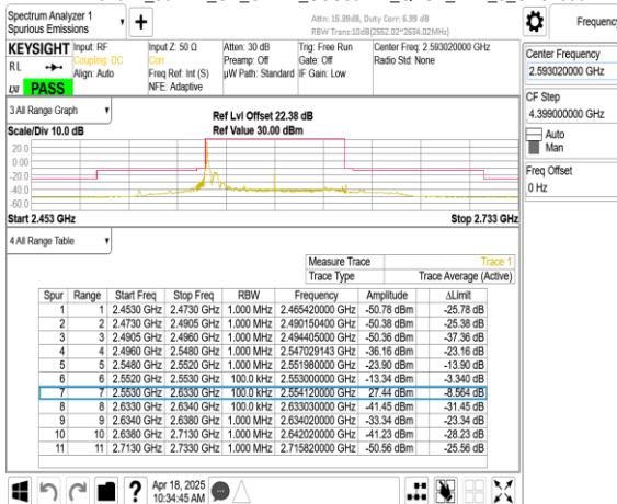
Band41_80MHz_CP_OFDM_SCS30kHz_QPSK_RB1_216_CH518604
