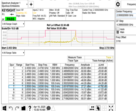
Band41_80MHz_DFT_s_OFDM_SCS30kHz_BPSK_RB216_0_CH518604
