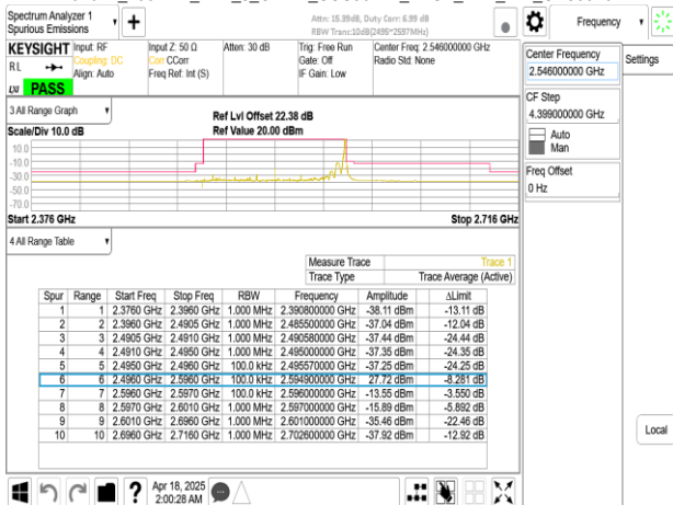
Band41_100MHz_DFT_s_OFDM_SCS30kHz_BPSK_RB270_0_CH509202
