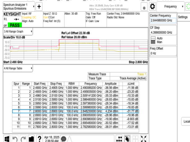
Band41_90MHz_CP_OFDM_SCS30kHz_QPSK_RB245_0_CH528996
