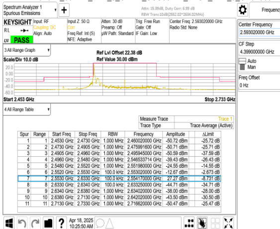
Band41_80MHz_DFT_s_OFDM_SCS30kHz_BPSK_RB1_216_CH518604
