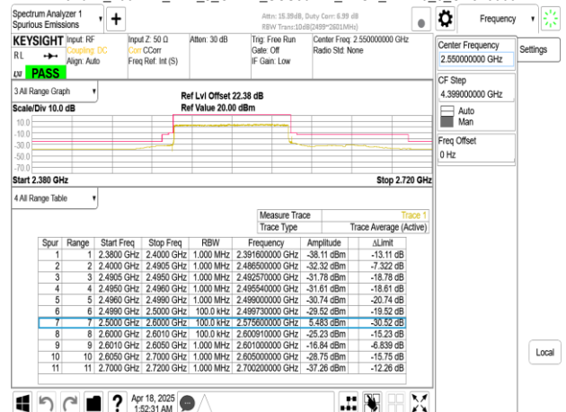
Band41_100MHz_DFT_s_OFDM_SCS30kHz_BPSK_RB270_0_CH510000
