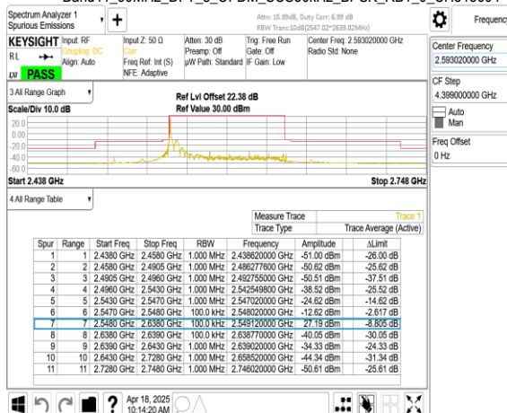
Band41_90MHz_DFT_s_OFDM_SCS30kHz_BPSK_RB1_244_CH518604
