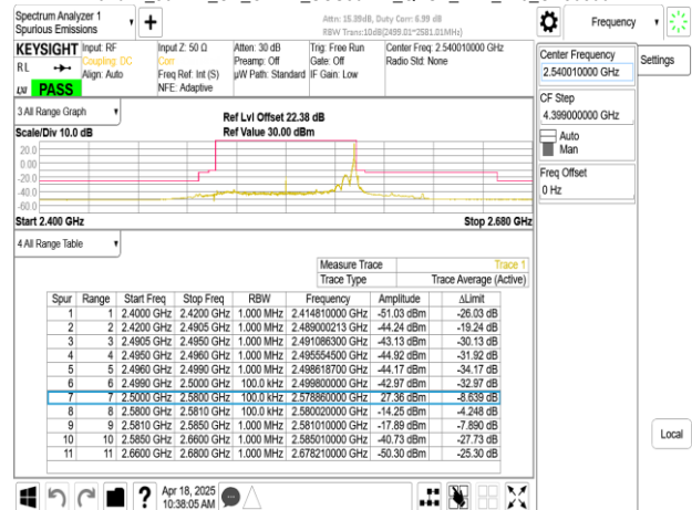
Band41_80MHz_CP_OFDM_SCS30kHz_QPSK_RB217_0_CH508002
