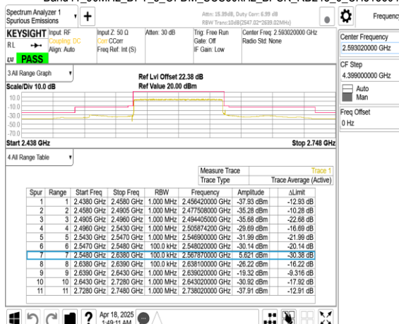
Band41_90MHz_DFT_s_OFDM_SCS30kHz_BPSK_RB243_0_CH518604
