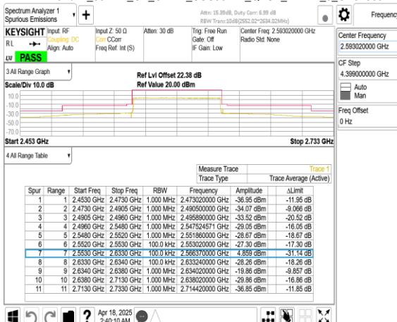
Band41_80MHz_CP_OFDM_SCS30kHz_QPSK_RB217_0_CH518604
