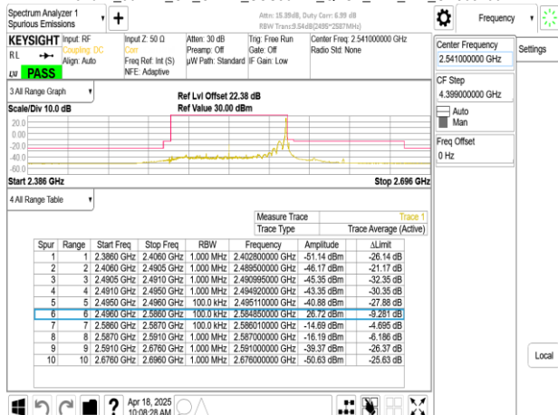
Band41_90MHz_CP_OFDM_SCS30kHz_QPSK_RB245_0_CH508200
