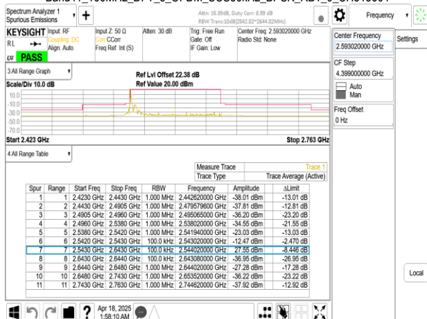
Band41_100MHz_DFT_s_OFDM_SCS30kHz_BPSK_RB1_272_CH518604
