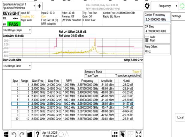
Band41_90MHz_DFT_s_OFDM_SCS30kHz_BPSK_RB243_0_CH508200
