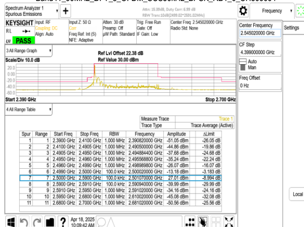
Band41_90MHz_DFT_s_OFDM_SCS30kHz_BPSK_RB1_244_CH509004
