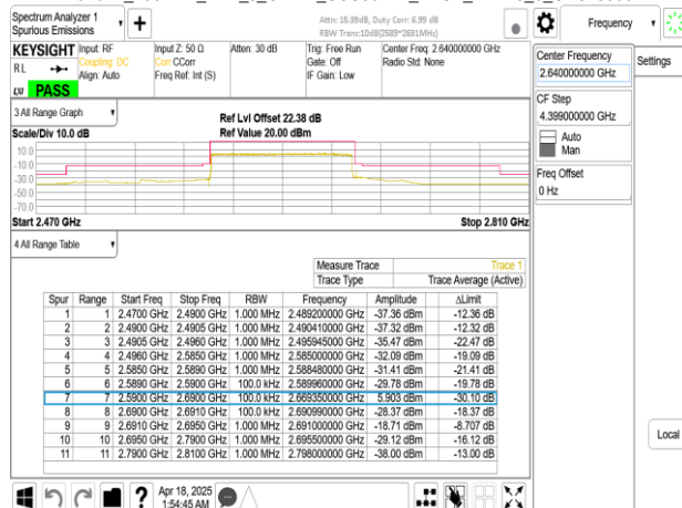
Band41_100MHz_DFT_s_OFDM_SCS30kHz_BPSK_RB270_0_CH528000
