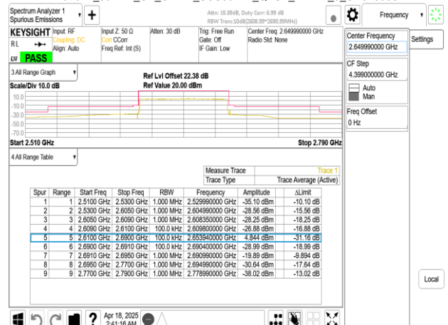
Band41_80MHz_CP_OFDM_SCS30kHz_QPSK_RB217_0_CH529998
