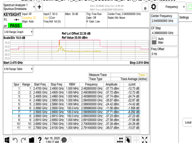
Band41_100MHz_DFT_s_OFDM_SCS30kHz_BPSK_RB1_272_CH528000
