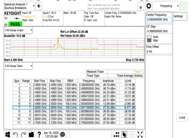
Band41_100MHz_DFT_s_OFDM_SCS30kHz_BPSK_RB1_272_CH510000
