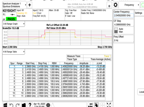
Band41_90MHz_CP_OFDM_SCS30kHz_QPSK_RB245_0_CH509004
