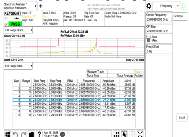
Band41_80MHz_CP_OFDM_SCS30kHz_QPSK_RB217_0_CH529998
