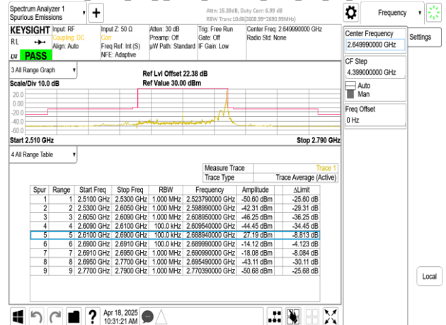
Band41_80MHz_DFT_s_OFDM_SCS30kHz_BPSK_RB216_0_CH529998
