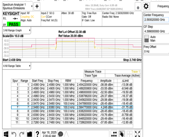
Band41_90MHz_CP_OFDM_SCS30kHz_QPSK_RB245_0_CH518604
