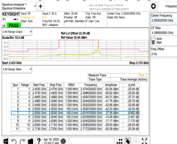
Band41_80MHz_CP_OFDM_SCS30kHz_QPSK_RB217_0_CH518604
