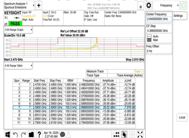
Band41_100MHz_CP_OFDM_SCS30kHz_QPSK_RB273_0_CH528000
