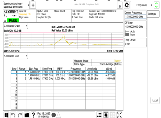
Band66_10MHz_DFT_s_OFDM_SCS15kHz_BPSK_RB50_0_CH355000
