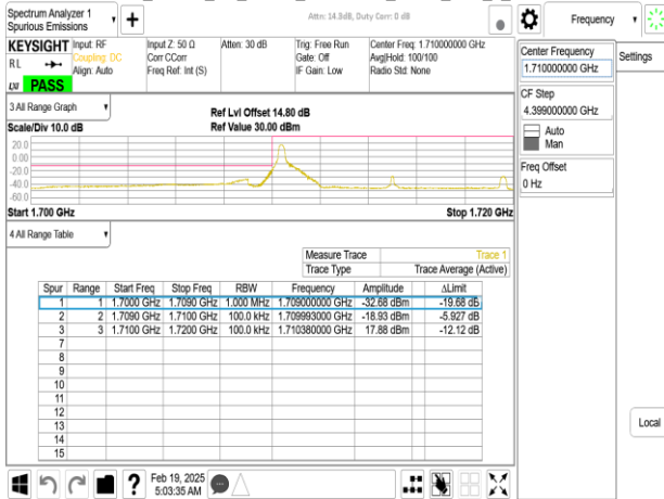
Band66_10MHz_CP_OFDM_SCS15kHz_QPSK_RB52_0_CH343000
