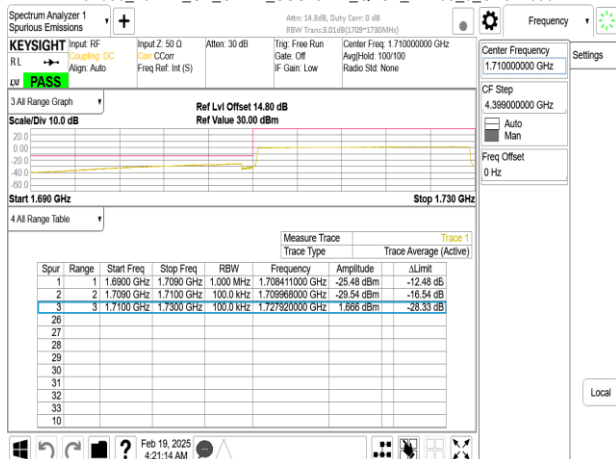
Band66_20MHz_CP_OFDM_SCS15kHz_QPSK_RB106_0_CH344000
