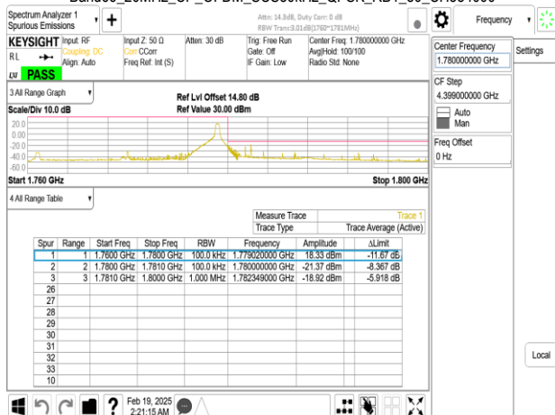
Band66_20MHz_CP_OFDM_SCS30kHz_QPSK_RB1_0_CH354000
