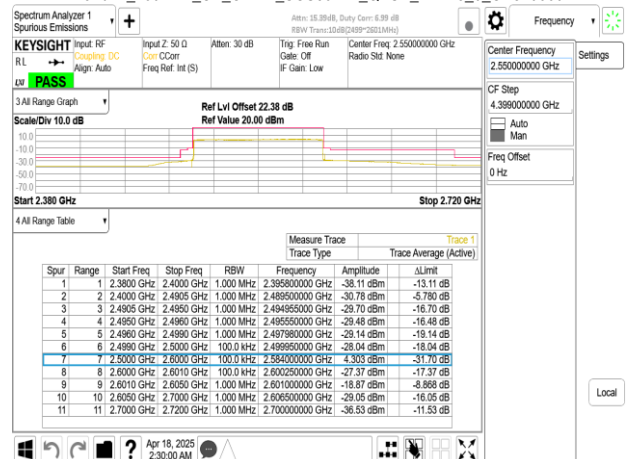
Band41_100MHz_CP_OFDM_SCS30kHz_QPSK_RB273_0_CH510000
