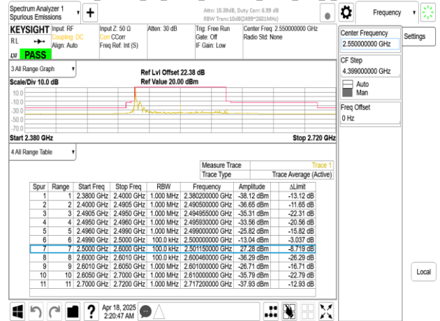
Band41_100MHz_CP_OFDM_SCS30kHz_QPSK_RB1_272_CH510000
