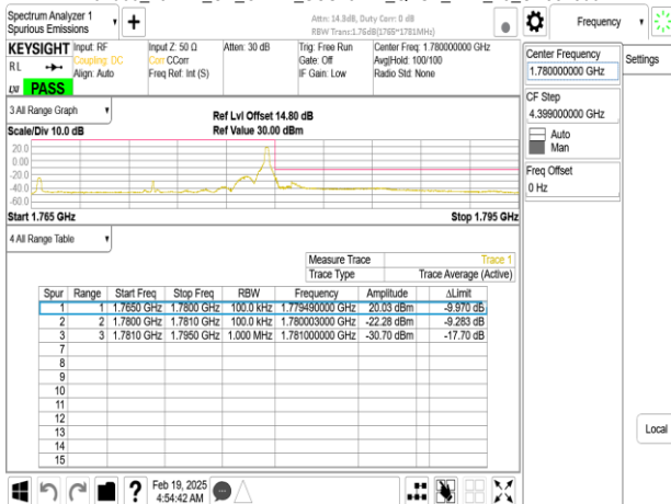
Band66_15MHz_CP_OFDM_SCS15kHz_QPSK_RB79_0_CH354500
