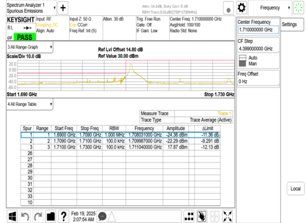
Band66_20MHz_CP_OFDM_SCS30kHz_QPSK_RB51_0_CH344000
