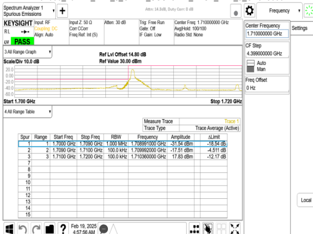
Band66_10MHz_DFT_s_OFDM_SCS15kHz_BPSK_RB1_0_CH343000
