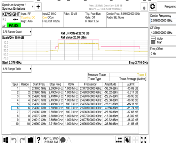
Band41_100MHz_CP_OFDM_SCS30kHz_QPSK_RB273_0_CH509202
