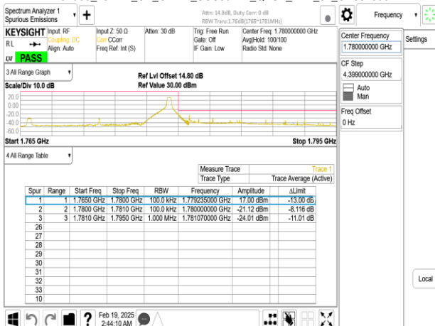
Band66_15MHz_CP_OFDM_SCS30kHz_QPSK_RB1_37_CH354500
