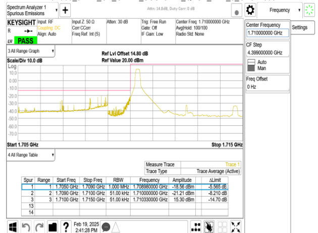
Band66_5MHz_CP_OFDM_SCS15kHz_QPSK_RB25_0_CH342500
