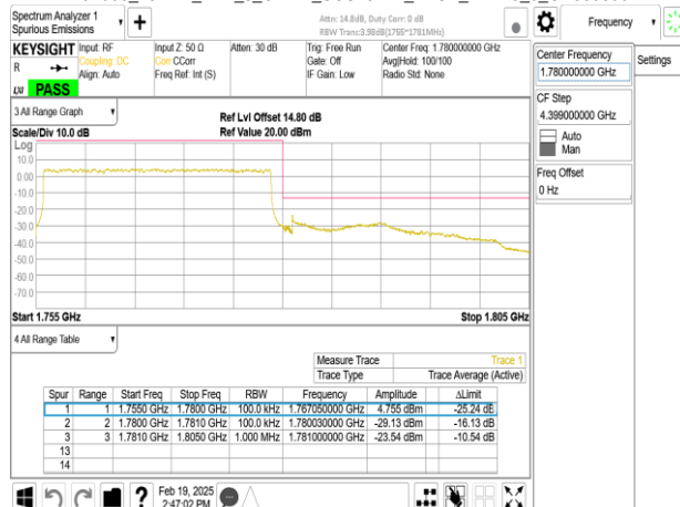
Band66_25MHz_DFT_s_OFDM_SCS15kHz_BPSK_RB1_132_CH353500
