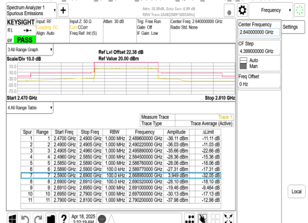
Band41_100MHz_CP_OFDM_SCS30kHz_QPSK_RB273_0_CH528000
