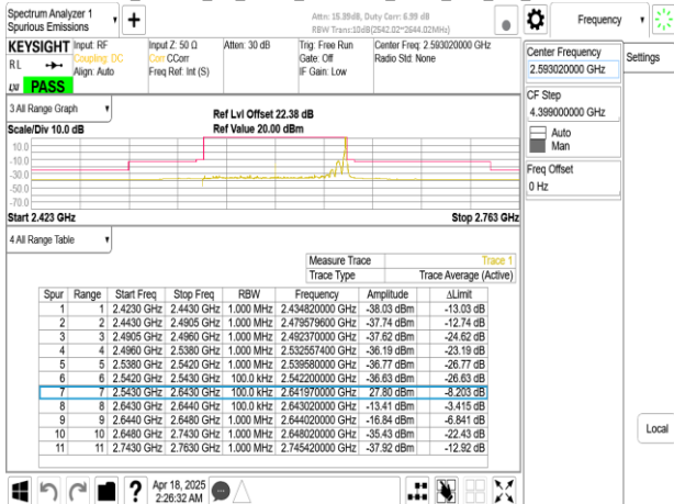
Band41_100MHz_CP_OFDM_SCS30kHz_QPSK_RB273_0_CH518604
