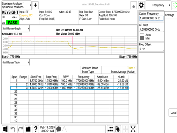
Band66_10MHz_DFT_s_OFDM_SCS30kHz_BPSK_RB24_0_CH355000
