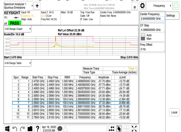
Band41_100MHz_CP_OFDM_SCS30kHz_QPSK_RB1_272_CH528000
