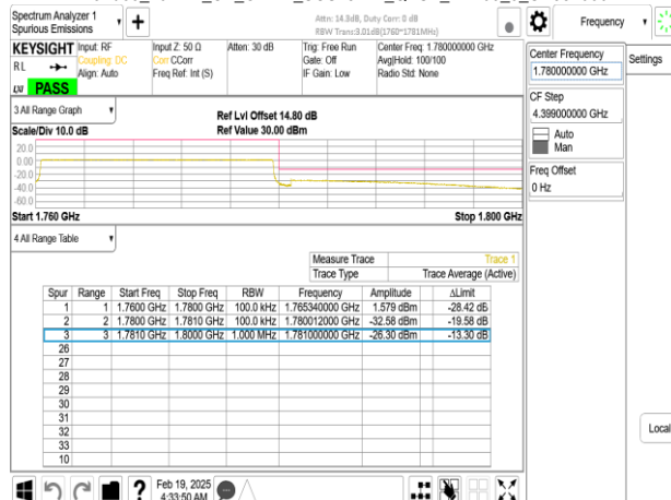
Band66_20MHz_CP_OFDM_SCS15kHz_QPSK_RB1_105_CH354000
