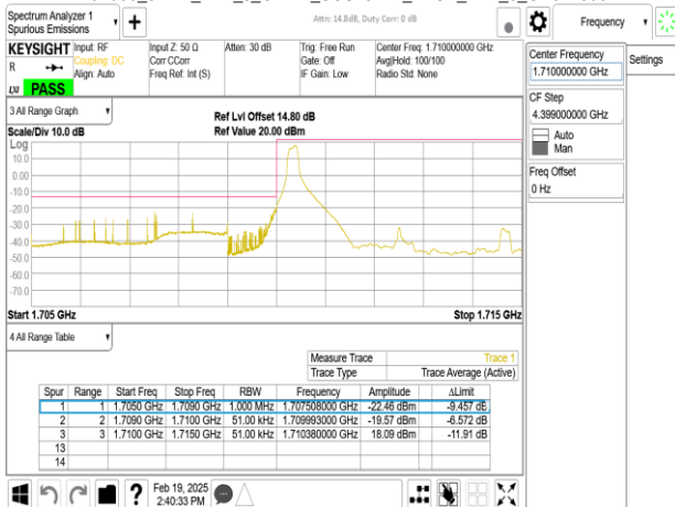
Band66_5MHz_DFT_s_OFDM_SCS15kHz_BPSK_RB25_0_CH342500
