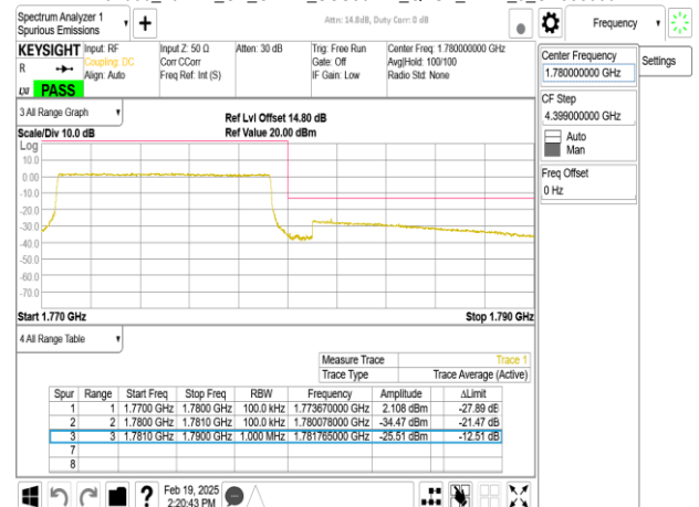
Band66_10MHz_CP_OFDM_SCS30kHz_QPSK_RB24_0_CH355000
