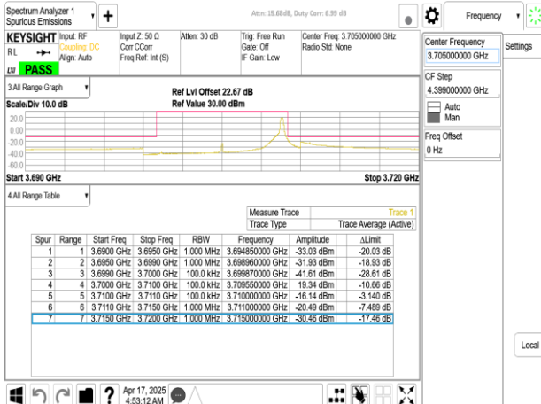
Band77-Part27_10MHz_CP_OFDM_SCS15kHz_QPSK_RB1_51_CH647000
