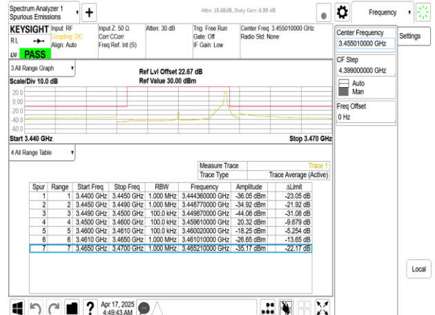
Band77-Part27_10MHz_CP_OFDM_SCS15kHz_QPSK_RB1_51_CH630334
