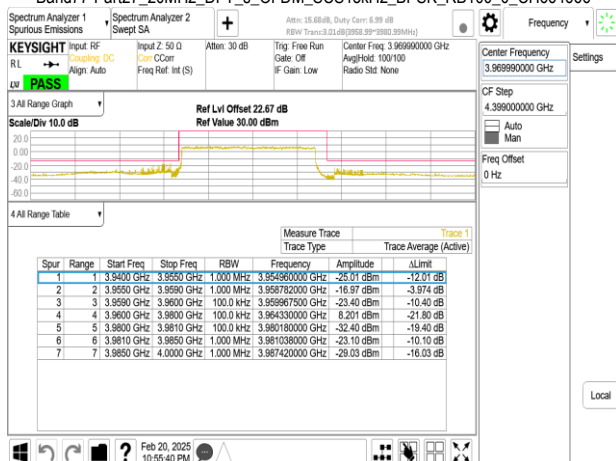
Band77-Part27_20MHz_DFT_s_OFDM_SCS15kHz_BPSK_RB1_0_CH664666
