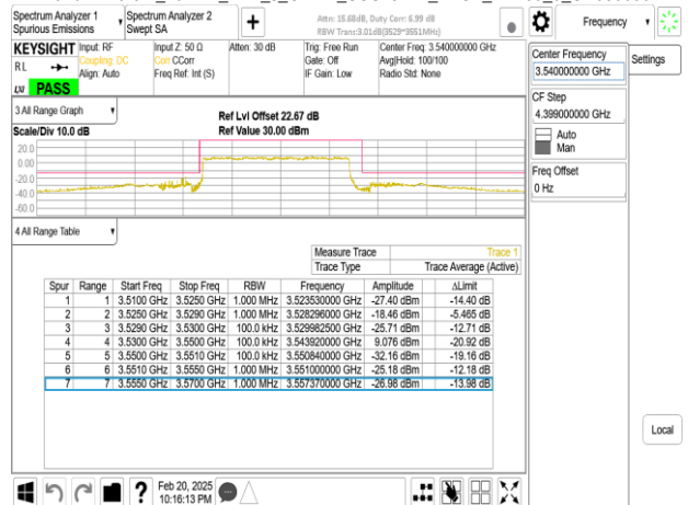
Band77-Part27_20MHz_DFT_s_OFDM_SCS15kHz_BPSK_RB1_0_CH636000
