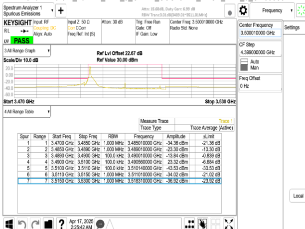
Band77-Part27_20MHz_DFT_s_OFDM_SCS15kHz_BPSK_RB1_0_CH633334
