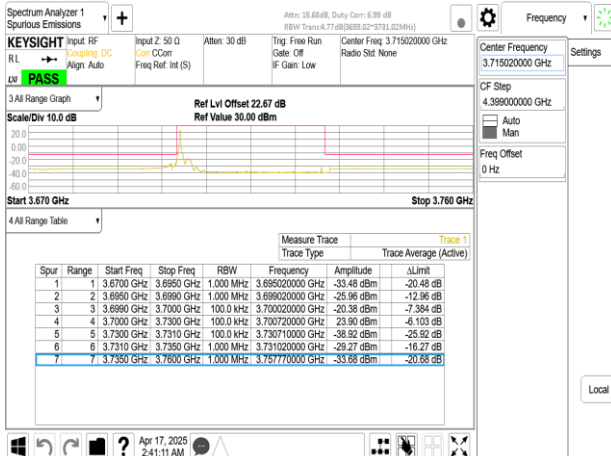
Band77-Part27_30MHz_DFT_s_OFDM_SCS15kHz_BPSK_RB1_0_CH647668
