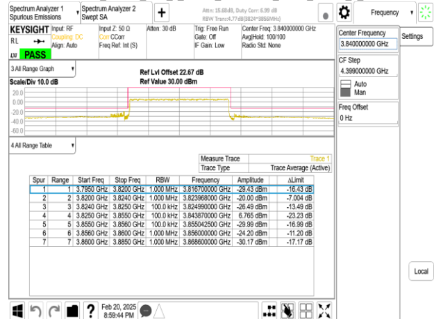
Band77-Part27_30MHz_DFT_s_OFDM_SCS15kHz_BPSK_RB1_0_CH656000
