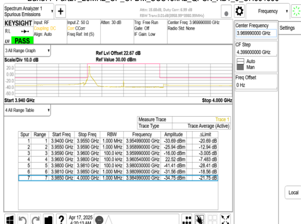
Band77-Part27_20MHz_CP_OFDM_SCS15kHz_QPSK_RB1_0_CH664666
