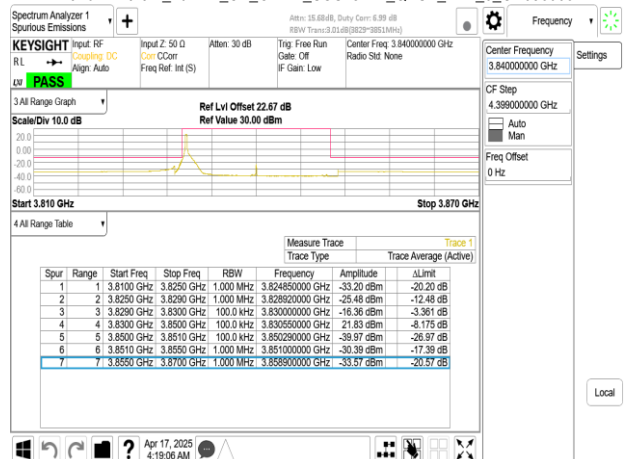
Band77-Part27_20MHz_CP_OFDM_SCS15kHz_QPSK_RB1_0_CH656000
