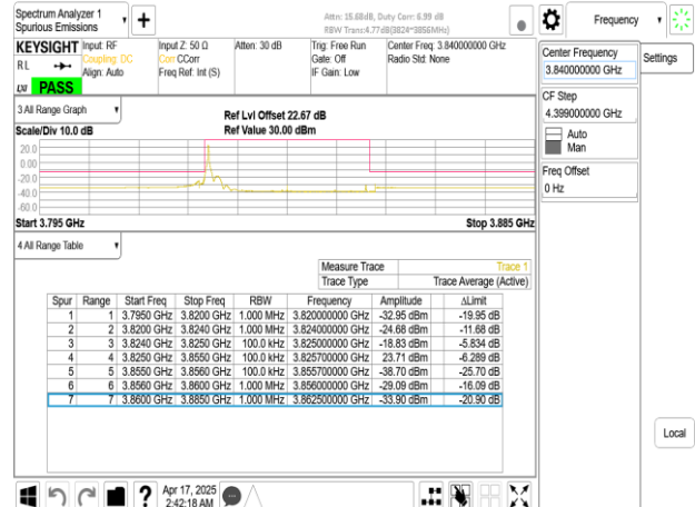
Band77-Part27_30MHz_DFT_s_OFDM_SCS15kHz_BPSK_RB1_0_CH656000
