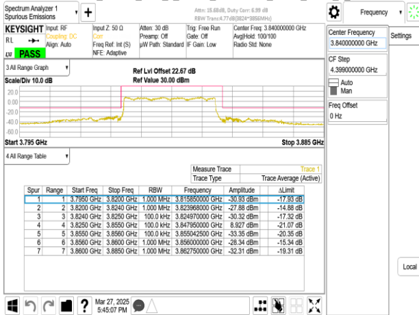
Band77-Part27_30MHz_DFT_s_OFDM_SCS30kHz_BPSK_RB1_0_CH664332
