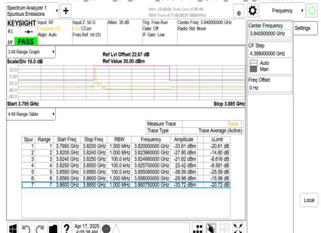
Band77-Part27_30MHz_CP_OFDM_SCS15kHz_QPSK_RB1_0_CH656000
