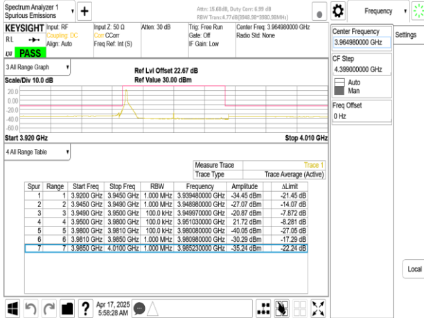
Band77-Part27_30MHz_DFT_s_OFDM_SCS30kHz_BPSK_RB1_77_CH664332
