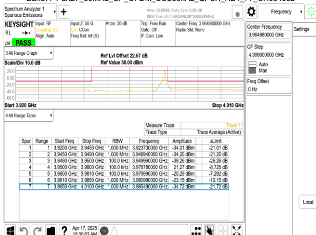
Band77-Part27_30MHz_CP_OFDM_SCS30kHz_QPSK_RB1_77_CH664332
