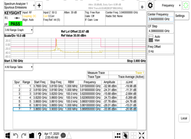
Band77-Part27_40MHz_DFT_s_OFDM_SCS15kHz_BPSK_RB1_215_CH656000
