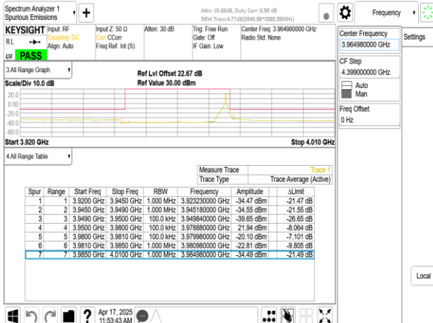
Band77-Part27_30MHz_DFT_s_OFDM_SCS30kHz_BPSK_RB1_77_CH664332
