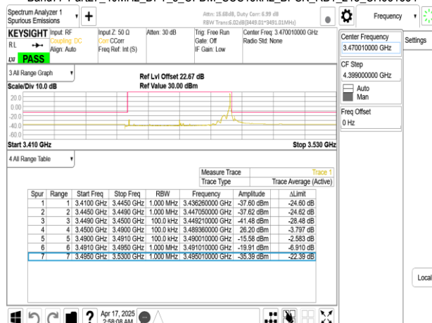
Band77-Part27_40MHz_DFT_s_OFDM_SCS15kHz_BPSK_RB1_215_CH631334
