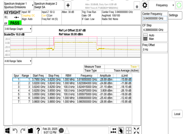
Band77-Part27_30MHz_CP_OFDM_SCS15kHz_QPSK_RB1_0_CH656000
