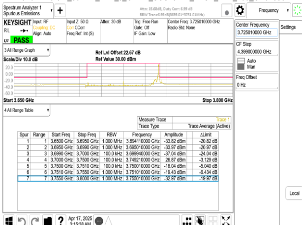
Band77-Part27_50MHz_DFT_s_OFDM_SCS15kHz_BPSK_RB1_269_CH648334
