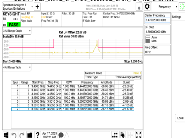
Band77-Part27_50MHz_CP_OFDM_SCS30kHz_QPSK_RB133_0_CH633334
