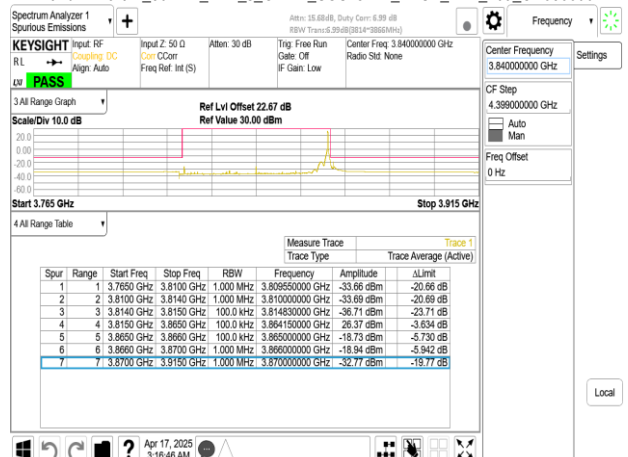
Band77-Part27_50MHz_DFT_s_OFDM_SCS15kHz_BPSK_RB1_269_CH656000
