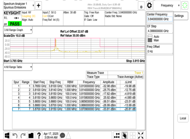
Band77-Part27_50MHz_DFT_s_OFDM_SCS15kHz_BPSK_RB1_269_CH656000
