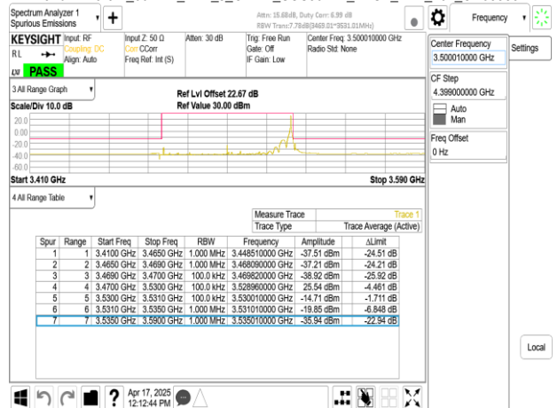
Band77-Part27_60MHz_DFT_s_OFDM_SCS30kHz_BPSK_RB162_0_CH634666
