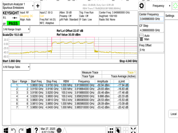
Band77-Part27_60MHz_DFT_s_OFDM_SCS30kHz_BPSK_RB1_0_CH663332
