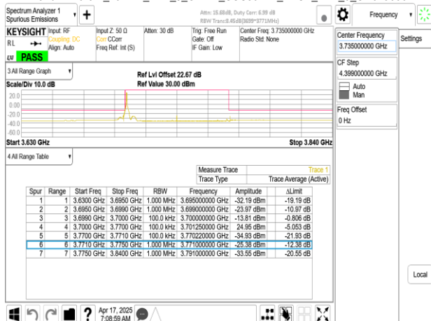
Band77-Part27_70MHz_DFT_s_OFDM_SCS30kHz_BPSK_RB1_0_CH649000
