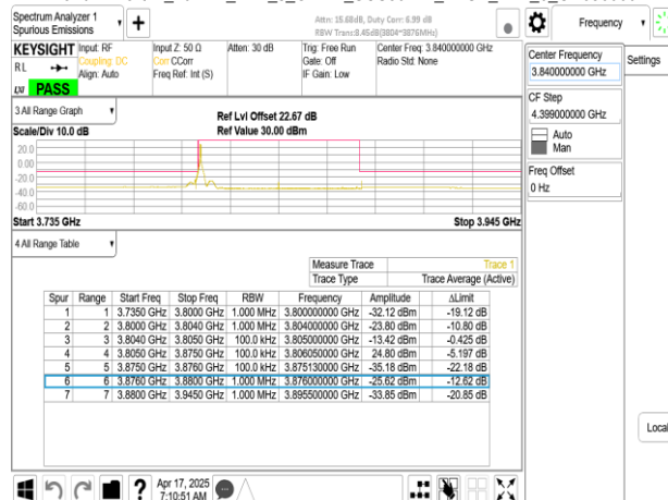
Band77-Part27_70MHz_DFT_s_OFDM_SCS30kHz_BPSK_RB1_0_CH656000
