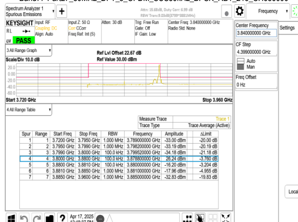
Band77-Part27_80MHz_DFT_s_OFDM_SCS30kHz_BPSK_RB1_216_CH656000
