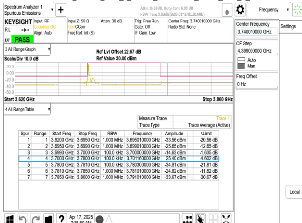
Band77-Part27_80MHz_DFT_s_OFDM_SCS30kHz_BPSK_RB1_216_CH649334
