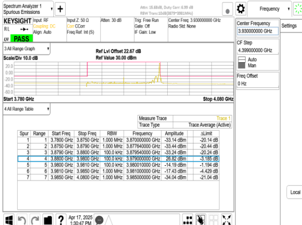
Band77-Part27_100MHz_DFT_s_OFDM_SCS30kHz_BPSK_RB1_272_CH662000
