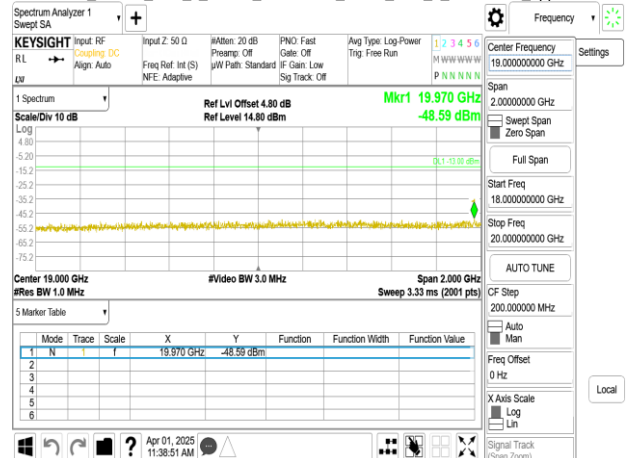
Band25_15MHz_DFT_s_OFDM_SCS30kHz_BPSK_RB1_1_CH376500_upper 18G
