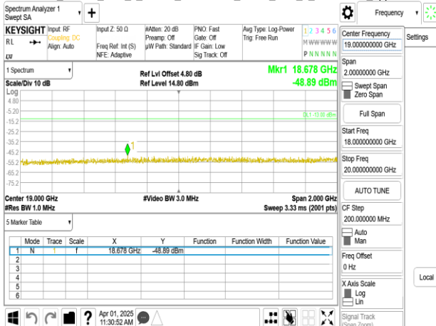
Band25_15MHz_DFT_s_OFDM_SCS15kHz_BPSK_RB1_1_CH376500_upper 18G
