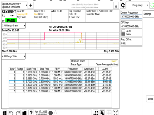
Band77-Part27_100MHz_DFT_s_OFDM_SCS30kHz_BPSK_RB1_272_CH650000
