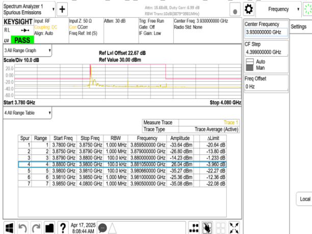
Band77-Part27_100MHz_DFT_s_OFDM_SCS30kHz_BPSK_RB1_272_CH662000
