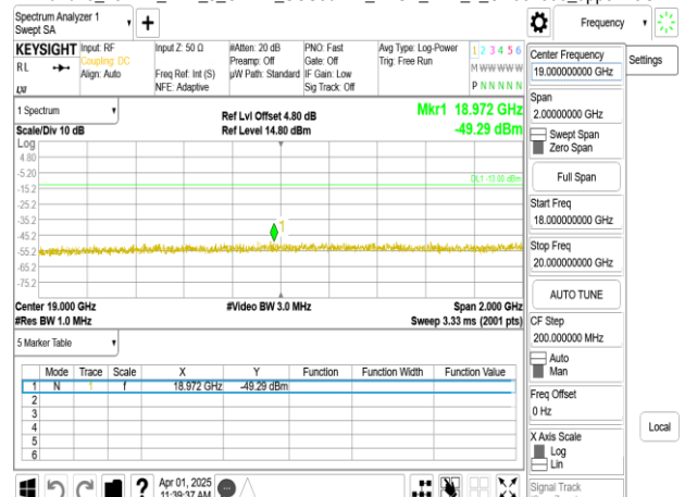
Band25_15MHz_DFT_s_OFDM_SCS30kHz_BPSK_RB1_1_CH381500_upper 18G
