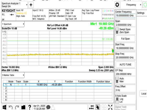
Band25_20MHz_DFT_s_OFDM_SCS15kHz_BPSK_RB1_1_CH381000_upper 18G
