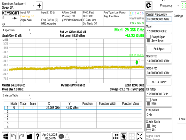
Band38_25MHz_DFT_s_OFDM_SCS30kHz_BPSK_RB1_1_CH516500_upper 18G
