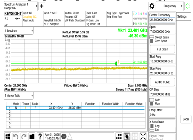
Band30_5MHz_DFT_s_OFDM_SCS15kHz_BPSK_RB1_1_CH462500_upper 18G
