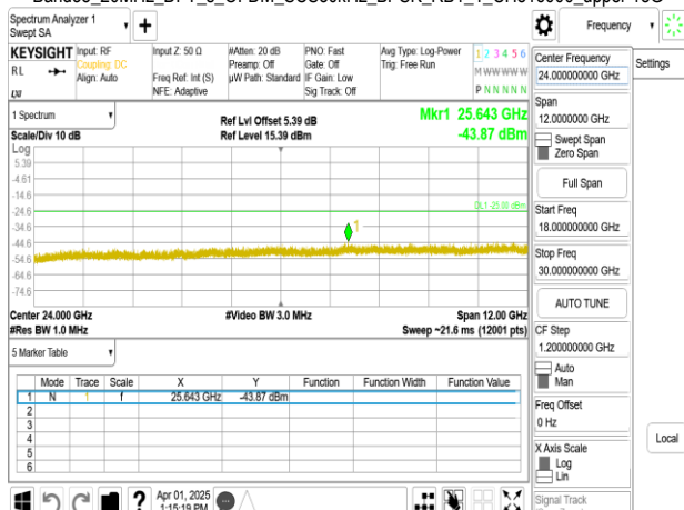
Band38_20MHz_DFT_s_OFDM_SCS30kHz_BPSK_RB1_1_CH516000_upper 18G
