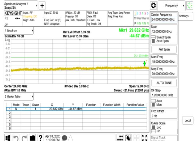
Band38_30MHz_DFT_s_OFDM_SCS15kHz_BPSK_RB1_1_CH517000_upper 18G
