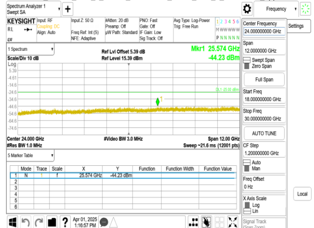
Band38_25MHz_DFT_s_OFDM_SCS30kHz_BPSK_RB1_1_CH521500_upper 18G
