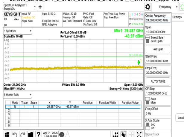
Band38_25MHz_DFT_s_OFDM_SCS15kHz_BPSK_RB1_1_CH516500_upper 18G
