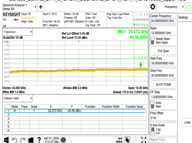
Band38_20MHz_DFT_s_OFDM_SCS15kHz_BPSK_RB1_1_CH522000_upper 18G
