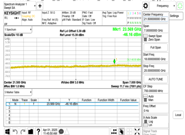
Band30_10MHz_DFT_s_OFDM_SCS15kHz_BPSK_RB1_1_CH515000_upper 18G
