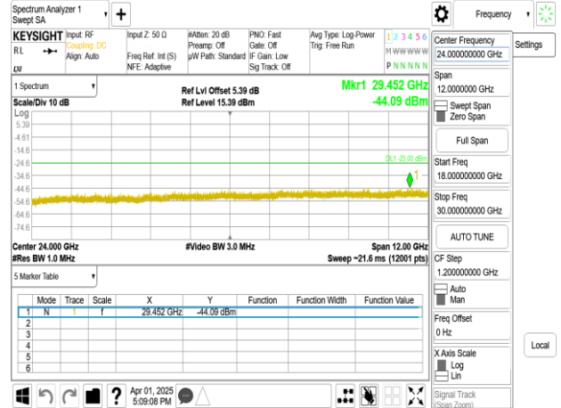
Band41_40MHz_DFT_s_OFDM_SCS15kHz_BPSK_RB1_1_CH503202_upper 18G
