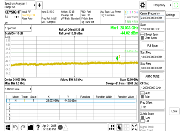
Band41_60MHz_DFT_s_OFDM_SCS30kHz_BPSK_RB1_1_CH531996_upper 18G
