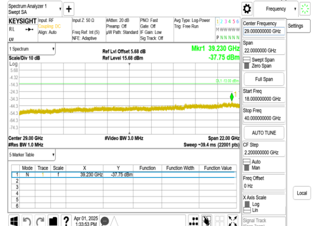
Band77-Part27_10MHz_DFT_s_OFDM_SCS15kHz_BPSK_RB1_1_CH656000_upper 18G
