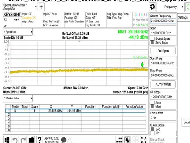
Band41_100MHz_DFT_s_OFDM_SCS30kHz_BPSK_RB1_1_CH518604_upper 18G
