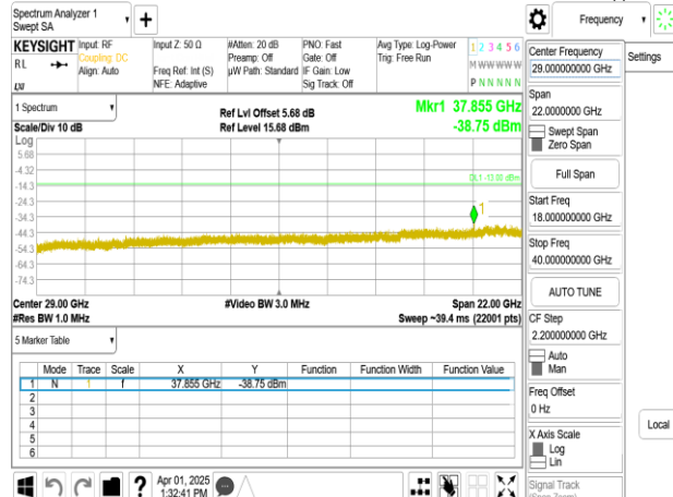
Band77-Part27_10MHz_DFT_s_OFDM_SCS15kHz_BPSK_RB1_1_CH636332_upper 18G
