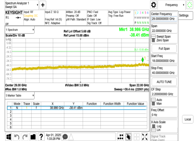
Band77-Part27_10MHz_DFT_s_OFDM_SCS15kHz_BPSK_RB1_1_CH656000_upper 18G
