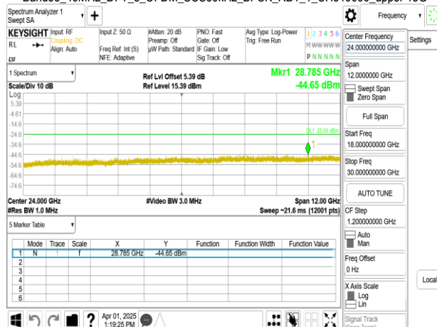
Band38_40MHz_DFT_s_OFDM_SCS30kHz_BPSK_RB1_1_CH520000_upper 18G
