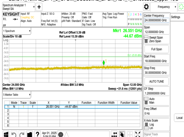
Band41_40MHz_DFT_s_OFDM_SCS30kHz_BPSK_RB1_1_CH503202_upper 18G
