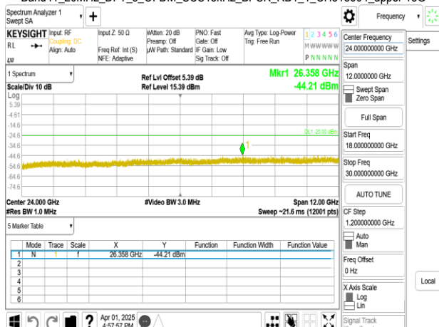
Band41_20MHz_DFT_s_OFDM_SCS15kHz_BPSK_RB1_1_CH518604_upper 18G
