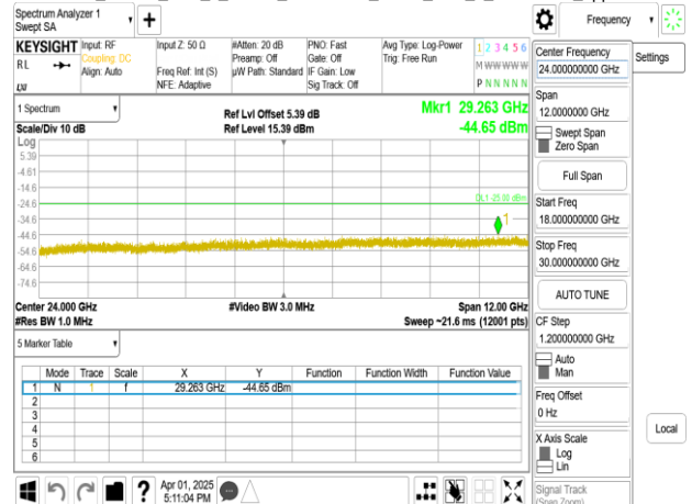
Band41_50MHz_DFT_s_OFDM_SCS30kHz_BPSK_RB1_1_CH505002_upper 18G
