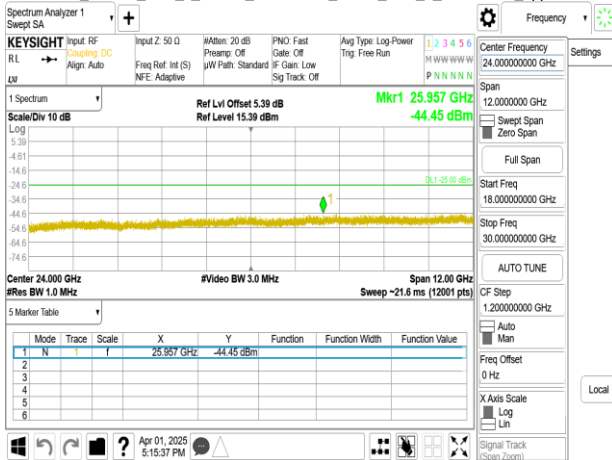
Band41_80MHz_DFT_s_OFDM_SCS30kHz_BPSK_RB1_1_CH508002_upper 18G
