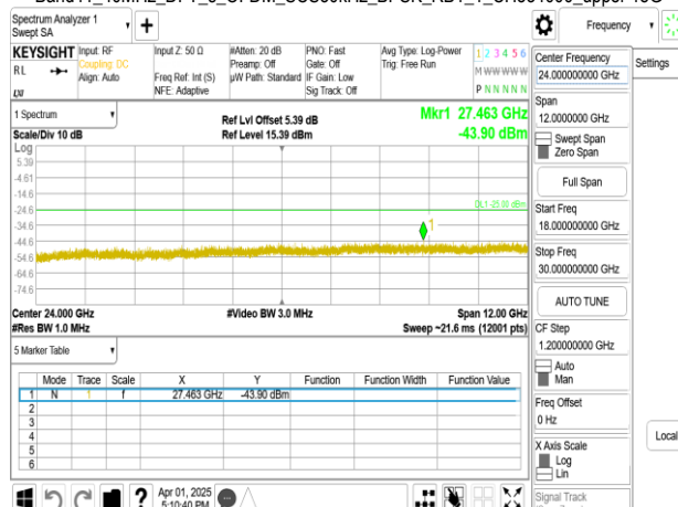
Band41_40MHz_DFT_s_OFDM_SCS30kHz_BPSK_RB1_1_CH534000_upper 18G
