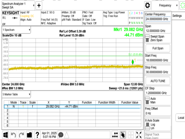
Band41_20MHz_DFT_s_OFDM_SCS30kHz_BPSK_RB1_1_CH535998_upper 18G
