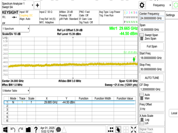
Band41_50MHz_DFT_s_OFDM_SCS15kHz_BPSK_RB1_1_CH518604_upper 18G
