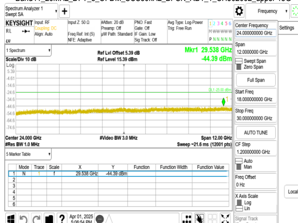
Band41_20MHz_DFT_s_OFDM_SCS30kHz_BPSK_RB1_1_CH502002_upper 18G
