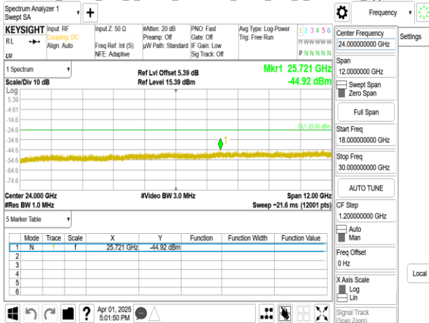
Band41_50MHz_DFT_s_OFDM_SCS15kHz_BPSK_RB1_1_CH505002_upper 18G
