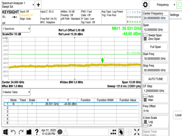
Band41_60MHz_DFT_s_OFDM_SCS30kHz_BPSK_RB1_1_CH505200_upper 18G
