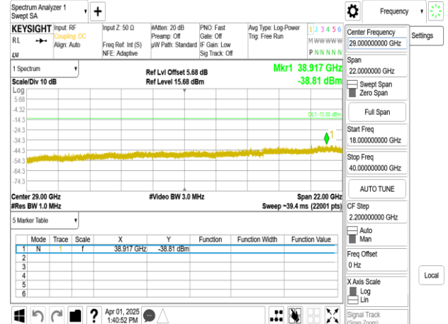
Band77-Part27_30MHz_DFT_s_OFDM_SCS15kHz_BPSK_RB1_1_CH64332_upper 18G
