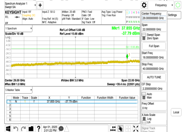
Band77-Part27_50MHz_DFT_s_OFDM_SCS30kHz_BPSK_RB1_1_CH663666_upper 18G
