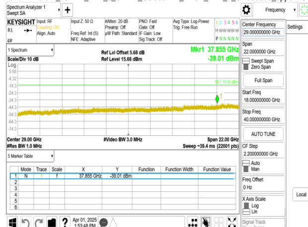
Band77-Part27_20MHz_DFT_s_OFDM_SCS30kHz_BPSK_RB1_1_CH664666_upper 18G
