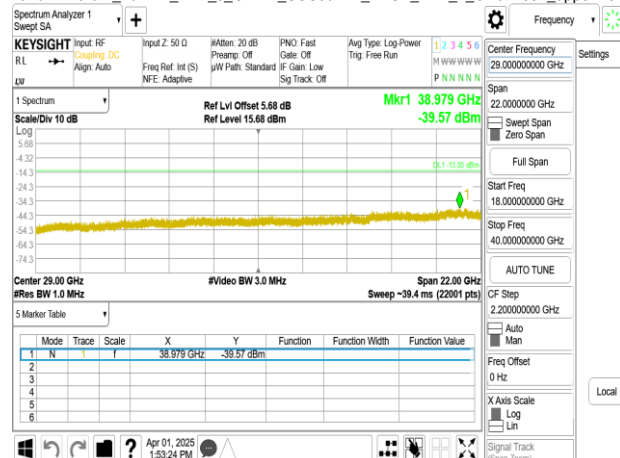
Band77-Part27_20MHz_DFT_s_OFDM_SCS30kHz_BPSK_RB1_1_CH656000_upper 18G
