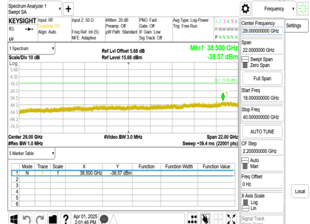
Band77-Part27_50MHz_DFT_s_OFDM_SCS30kHz_BPSK_RB1_1_CH663666_upper 18G
