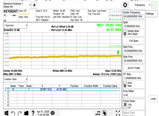
Band7_30MHz_DFT_s_OFDM_SCS30kHz_BPSK_RB1_1_CH507000_upper 18G
