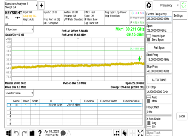
Band77-Part27_80MHz_DFT_s_OFDM_SCS30kHz_BPSK_RB1_1_CH662666_upper 18G
