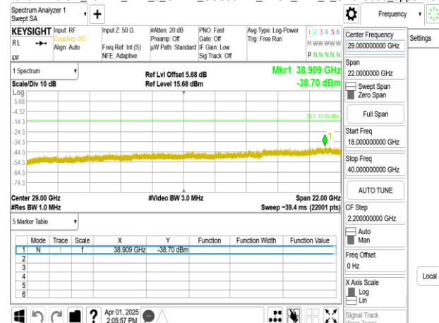
Band77-Part27_70MHz_DFT_s_OFDM_SCS30kHz_BPSK_RB1_1_CH656000_upper 18G
