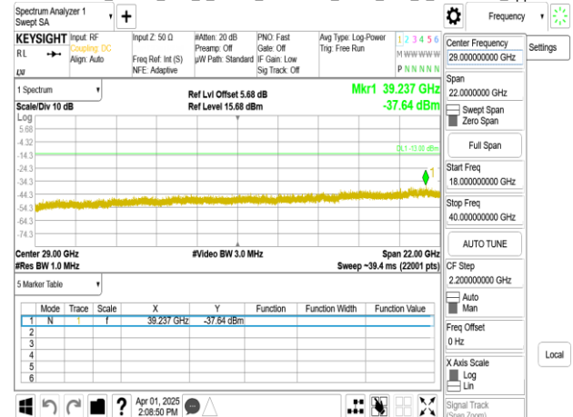
Band77-Part27_80MHz_DFT_s_OFDM_SCS30kHz_BPSK_RB1_1_CH662666_upper 18G
