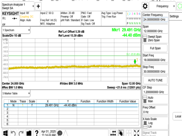
Band7_25MHz_DFT_s_OFDM_SCS15kHz_BPSK_RB1_1_CH511500_upper 18G
