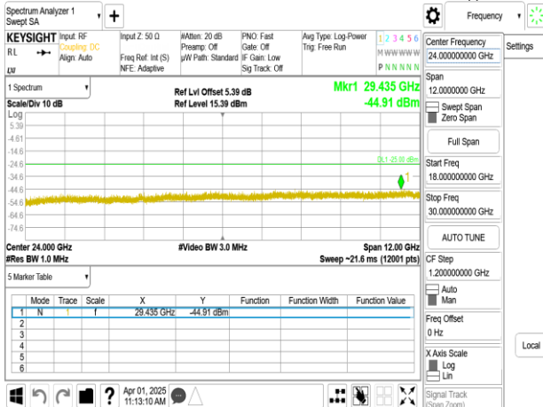
Band7_20MHz_DFT_s_OFDM_SCS15kHz_BPSK_RB1_1_CH512000_upper 18G
