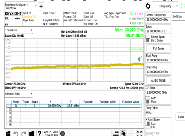
Band77-Part27_70MHz_DFT_s_OFDM_SCS30kHz_BPSK_RB1_1_CH663000_upper 18G
