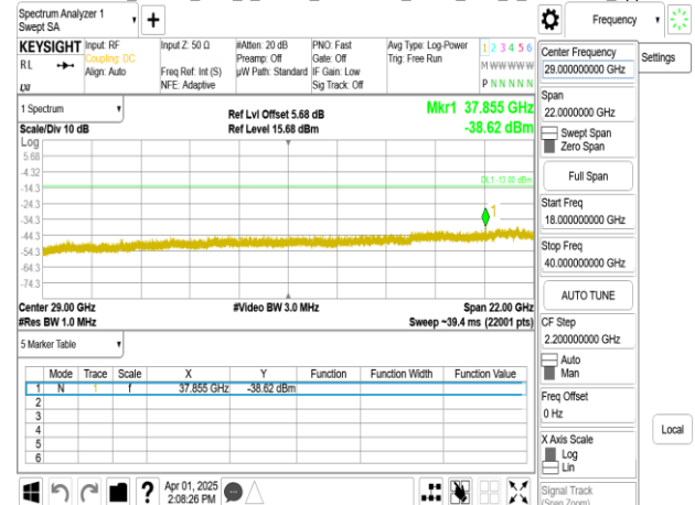
Band77-Part27_80MHz_DFT_s_OFDM_SCS30kHz_BPSK_RB1_1_CH656000_upper 18G
