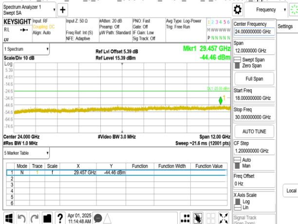
Band7_30MHz_DFT_s_OFDM_SCS15kHz_BPSK_RB1_1_CH507000_upper 18G
