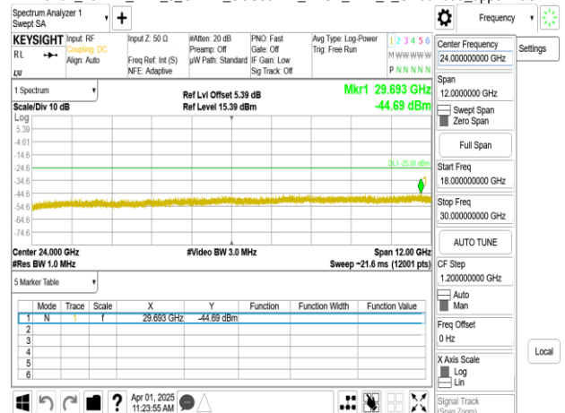
Band7_25MHz_DFT_s_OFDM_SCS30kHz_BPSK_RB1_1_CH511500_upper 18G
