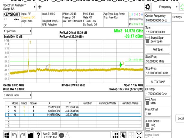
Band7_50MHz_DFT_s_OFDM_SCS30kHz_BPSK_RB1_1_CH509000_below 18G
