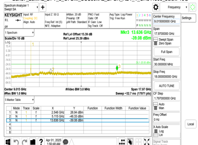
Band7_25MHz_DFT_s_OFDM_SCS30kHz_BPSK_RB1_1_CH511500_below 18G
