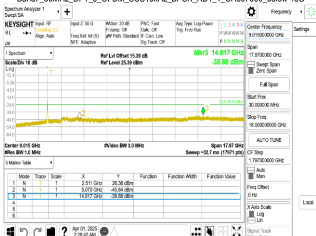
Band7_50MHz_DFT_s_OFDM_SCS15kHz_BPSK_RB1_1_CH509000_below 18G
