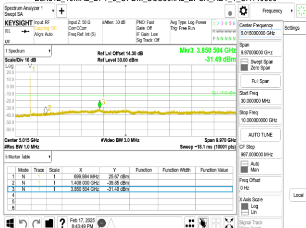
Band12_10MHz_DFT_s_OFDM_SCS30kHz_BPSK_RB1_1.CH141500
