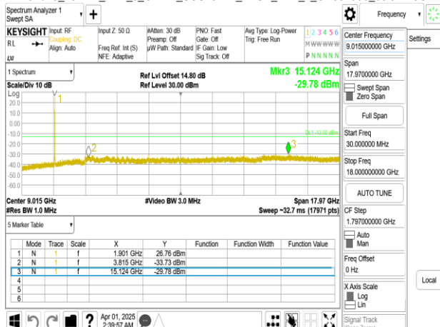
Band25_15MHz_DFT_s_OFDM_SCS30kHz_BPSK_RB1_1_CH371500_below 18G
