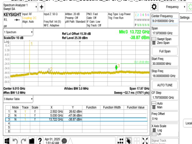
Band7_30MHz_DFT_s_OFDM_SCS30kHz_BPSK_RB1_1_CH507000_below 18G
