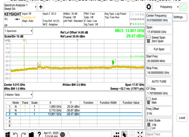
Band25_10MHz_DFT_s_OFDM_SCS15kHz_BPSK_RB1_1_CH371000_below 18G
