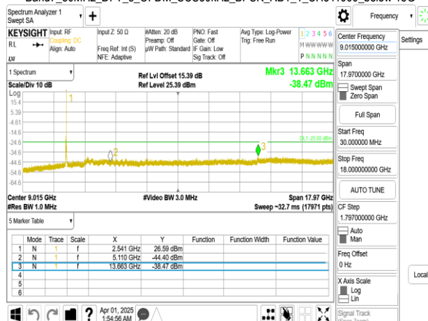
Band7_30MHz_DFT_s_OFDM_SCS30kHz_BPSK_RB1_1_CH511000_below 18G
