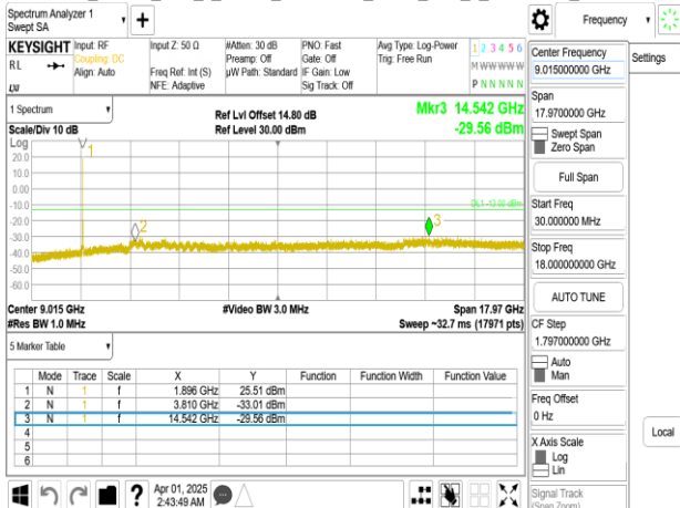
Band25_20MHz_DFT_s_OFDM_SCS30kHz_BPSK_RB1_1_CH372000_below 18G
