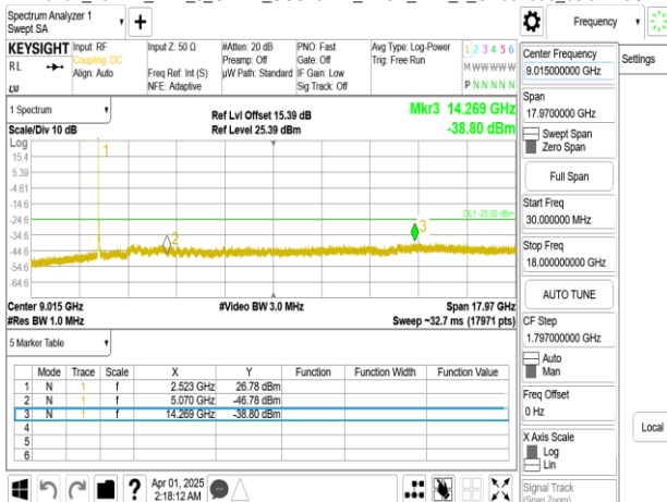
Band7_25MHz_DFT_s_OFDM_SCS15kHz_BPSK_RB1_1_CH511500_below 18G
