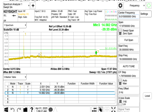
Band7_40MHz_DFT_s_OFDM_SCS30kHz_BPSK_RB1_1_CH510000_below 18G
