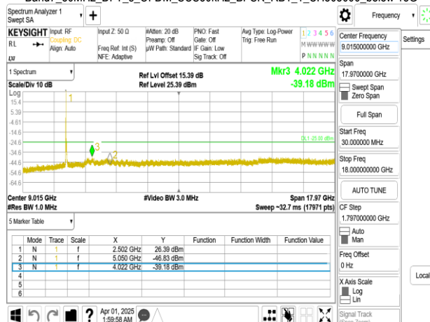
Band7_50MHz_DFT_s_OFDM_SCS30kHz_BPSK_RB1_1_CH507000_below 18G
