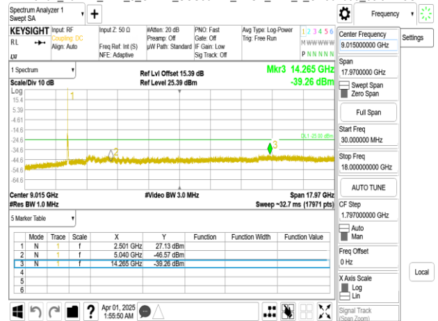
Band7_40MHz_DFT_s_OFDM_SCS30kHz_BPSK_RB1_1_CH507000_below 18G
