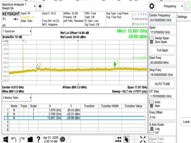
Band25_10MHz_DFT_s_OFDM_SCS15kHz_BPSK_RB1_1_CH382000_below 18G
