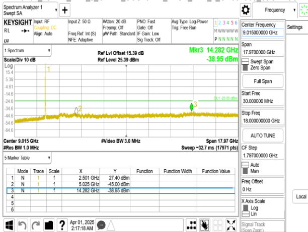
Band7_25MHz_DFT_s_OFDM_SCS15kHz_BPSK_RB1_1_CH507000_below 18G
