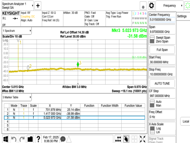
Band12_15MHz_DFT_s_OFDM_SCS30kHz_BPSK_RB1_1_CH141700
