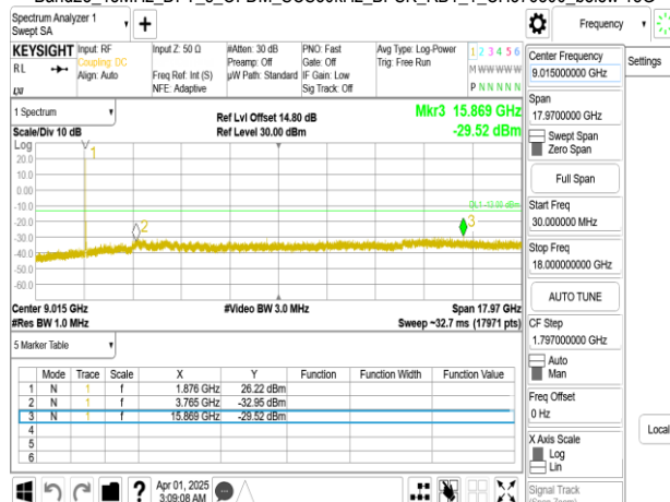
Band25_15MHz_DFT_s_OFDM_SCS30kHz_BPSK_RB1_1_CH381500_below 18G
