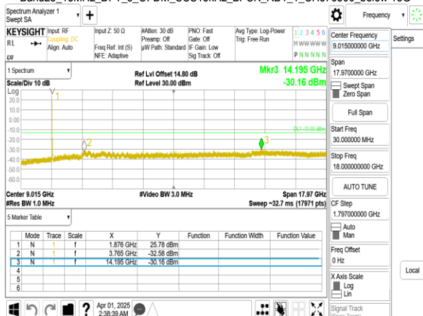
Band25_15MHz_DFT_s_OFDM_SCS15kHz_BPSK_RB1_1_CH381500_below 18G
