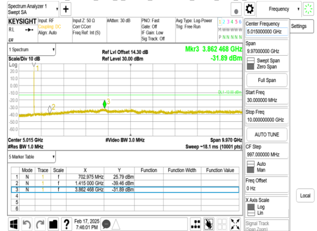
Band12_10MHz_DFT_s_OFDM_SCS15kHz_BPSK_RB1_1.CH142200
