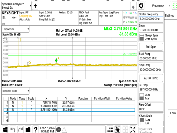
Band14_10MHz_DFT_s_OFDM_SCS30kHz_BPSK_RB1_1_CH158600
