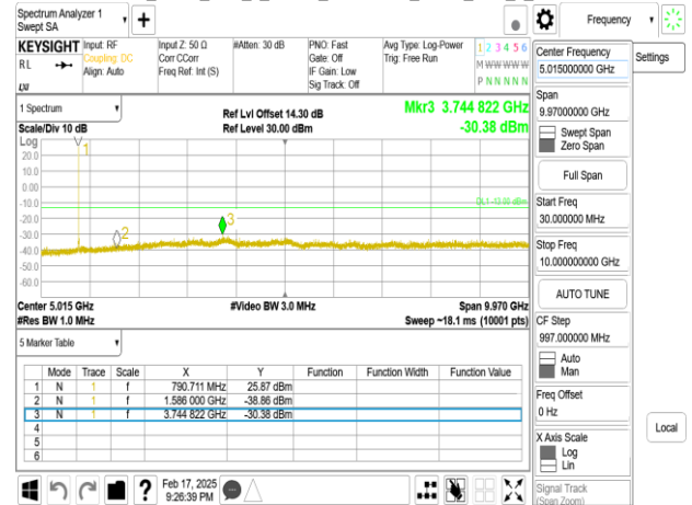
Band14_5MHz_DFT_s_OFDM_SCS15kHz_BPSK_RB1_1_CH159100
