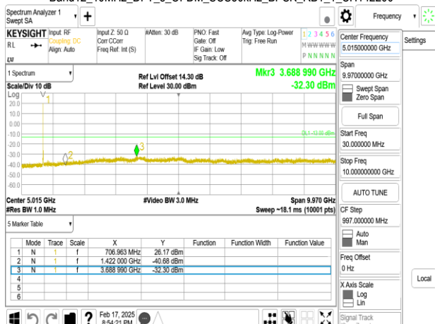
Band12_10MHz_DFT_s_OFDM_SCS30kHz_BPSK_RB1_1.CH142200
