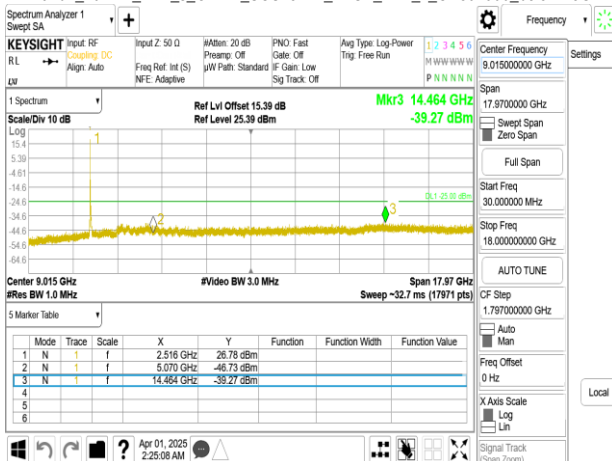
Band7_40MHz_DFT_s_OFDM_SCS15kHz_BPSK_RB1_1_CH510000_below 18G
