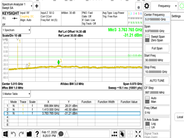
Band12_15MHz_DFT_s_OFDM_SCS30kHz_BPSK_RB1_1_CH141500
