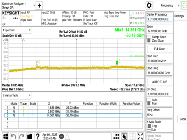
Band25_30MHz_DFT_s_OFDM_SCS30kHz_BPSK_RB1_1_CH373000_below 18G
