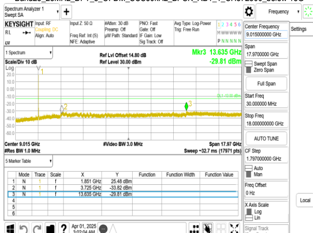
Band25_25MHz_DFT_s_OFDM_SCS30kHz_BPSK_RB1_1_CH372500_below 18G
