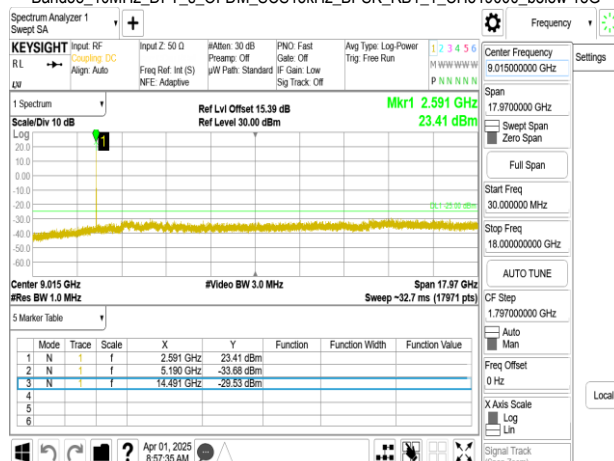
Band38_10MHz_DFT_s_OFDM_SCS15kHz_BPSK_RB1_1_CH523000_below 18G
