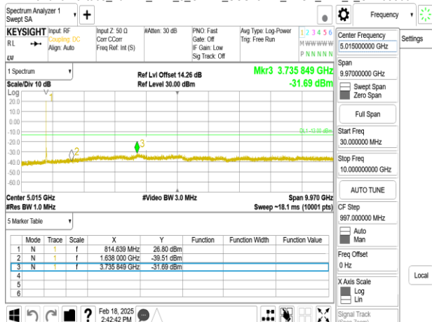
Band26-Part90s_10MHz_DFT_s_OFDM_SCS15kHz_BPSK_RB1_1_CH163800
