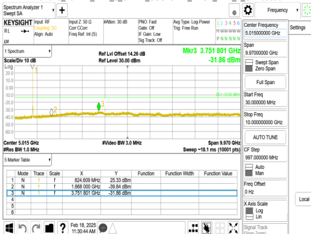
Band26_20MHz_DFT_s_OFDM_SCS15kHz_BPSK_RB1_1_CH167300
