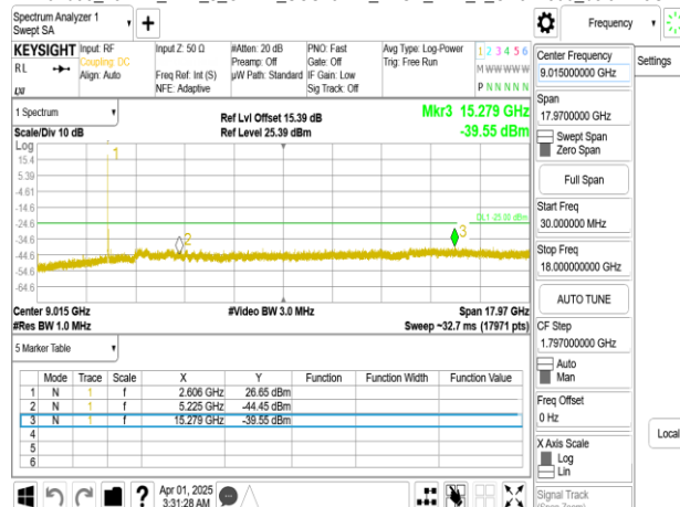
Band38_15MHz_DFT_s_OFDM_SCS15kHz_BPSK_RB1_1_CH522500_below 18G
