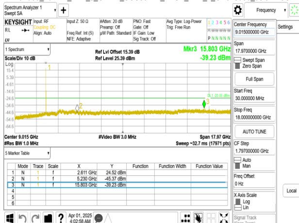
Band38_10MHz_DFT_s_OFDM_SCS30kHz_BPSK_RB1_1_CH523000_below 18G
