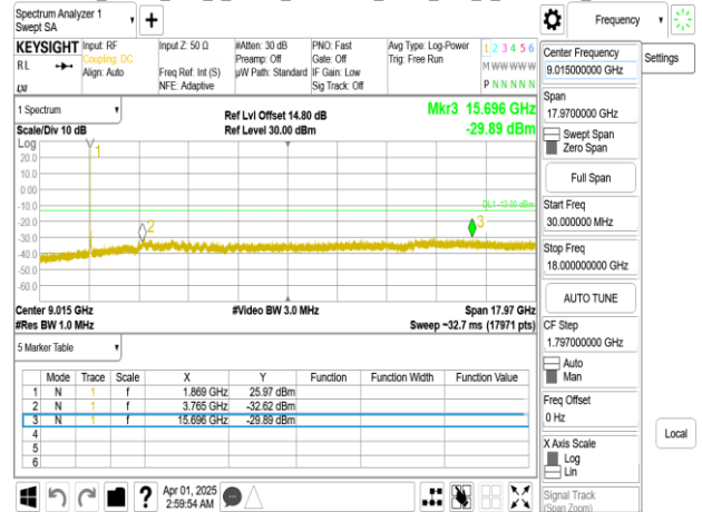
Band25_30MHz_DFT_s_OFDM_SCS30kHz_BPSK_RB1_1_CH380000_below 18G
