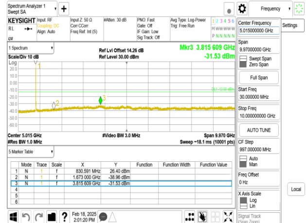
Band26_15MHz_DFT_s_OFDM_SCS30kHz_BPSK_RB1_1_CH167300
