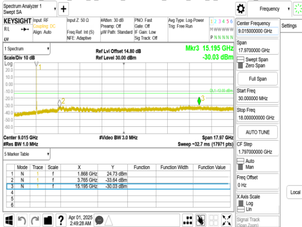
Band25_30MHz_DFT_s_OFDM_SCS15kHz_BPSK_RB1_1_CH380000_below 18G
