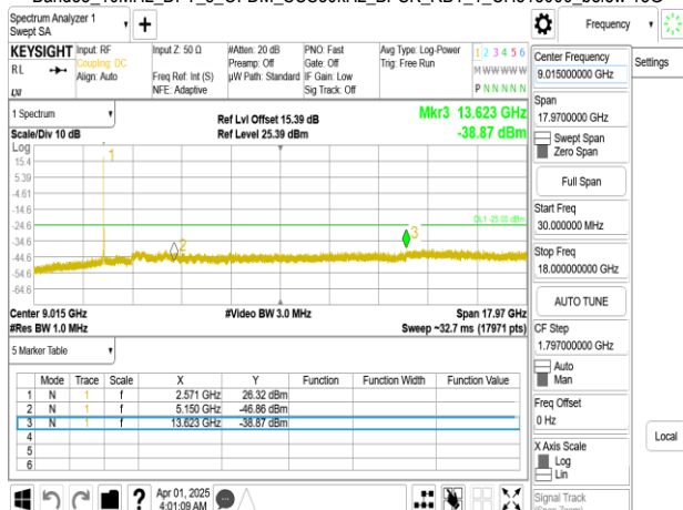
Band38_10MHz_DFT_s_OFDM_SCS30kHz_BPSK_RB1_1_CH519000_below 18G
