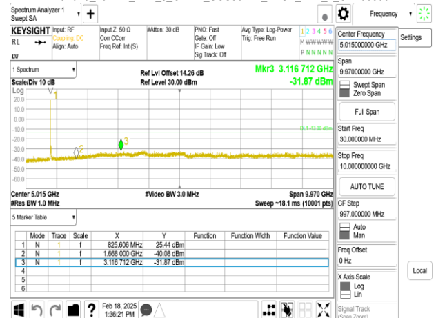
Band26_20MHz_DFT_s_OFDM_SCS30kHz_BPSK_RB1_1_CH167300
