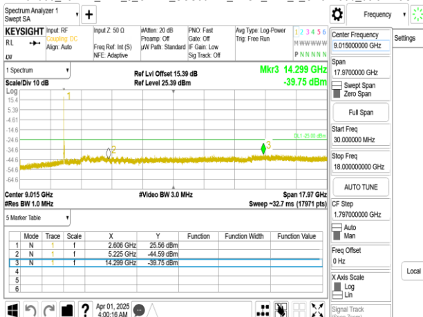
Band38_15MHz_DFT_s_OFDM_SCS30kHz_BPSK_RB1_1_CH522500_below 18G
