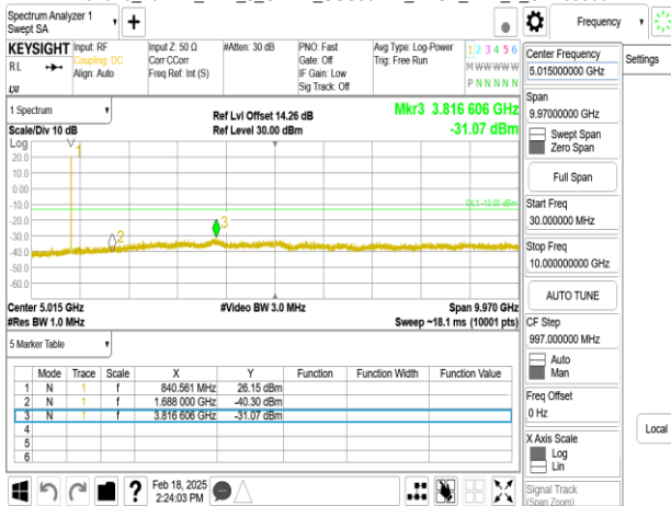
Band26_15MHz_DFT_s_OFDM_SCS15kHz_BPSK_RB1_1_CH166300
