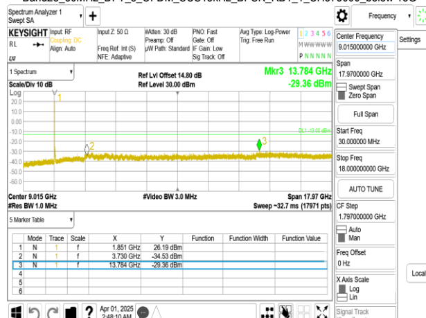
Band25_30MHz_DFT_s_OFDM_SCS15kHz_BPSK_RB1_1_CH373000_below 18G
