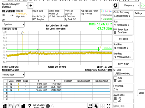
Band38_5MHz_DFT_s_OFDM_SCS15kHz_BPSK_RB1_1_CH523500_below 18G
