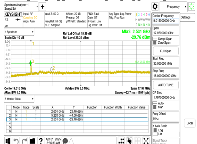
Band38_20MHz_DFT_s_OFDM_SCS15kHz_BPSK_RB1_1_CH522000_below 18G
