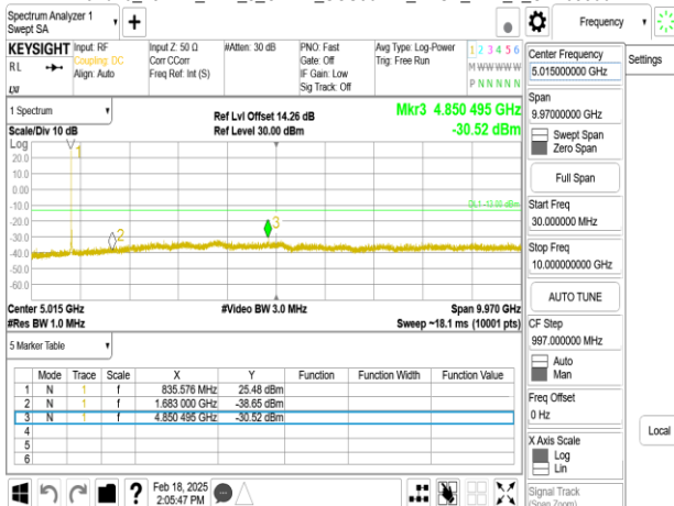
Band26_20MHz_DFT_s_OFDM_SCS15kHz_BPSK_RB1_1_CH166800
