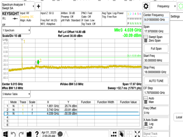
Band25_40MHz_DFT_s_OFDM_SCS30kHz_BPSK_RB1_1_CH374000_below 18G
