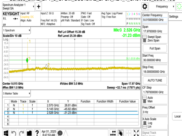
Band38_5MHz_DFT_s_OFDM_SCS15kHz_BPSK_RB1_1_CH518500_below 18G
