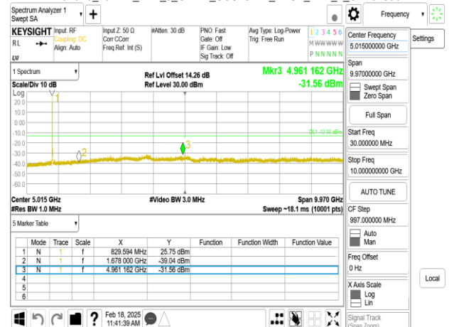
Band26_20MHz_DFT_s_OFDM_SCS30kHz_BPSK_RB1_1_CH166800
