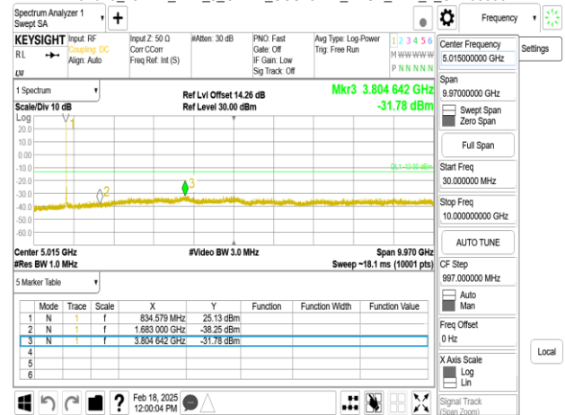
Band26_15MHz_DFT_s_OFDM_SCS30kHz_BPSK_RB1_1_CH166300
