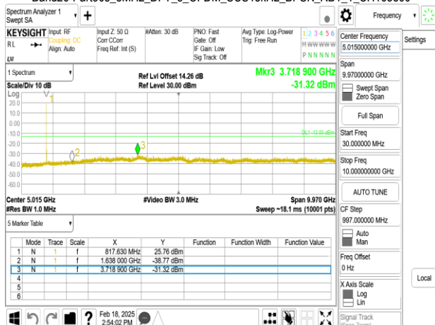
Band26-Part90s_5MHz_DFT_s_OFDM_SCS15kHz_BPSK_RB1_1_CH164300
