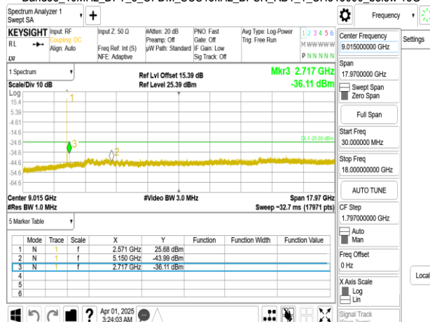
Band38_10MHz_DFT_s_OFDM_SCS15kHz_BPSK_RB1_1_CH519000_below 18G
