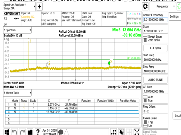
Band38_15MHz_DFT_s_OFDM_SCS15kHz_BPSK_RB1_1_CH519000_below 18G
