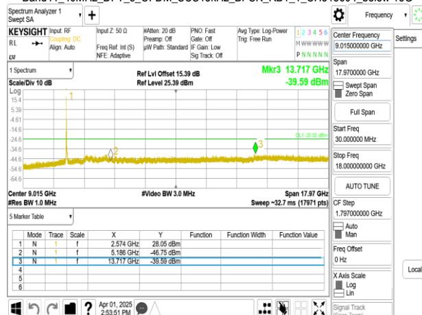
Band41_40MHz_DFT_s_OFDM_SCS15kHz_BPSK_RB1_1_CH534000_below 18G
