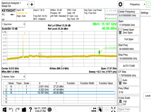
Band41_60MHz_DFT_s_OFDM_SCS30kHz_BPSK_RB1_1_CH531996_below 18G
