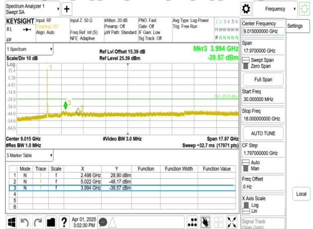
Band41_30MHz_DFT_s_OFDM_SCS30kHz_BPSK_RB1_1_CH503004_below 18G
