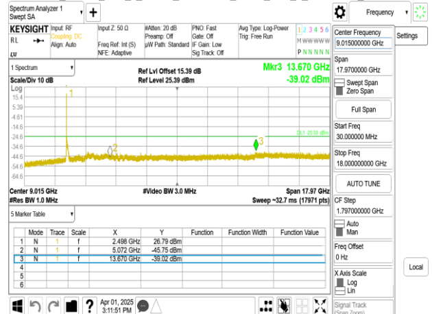
Band41_80MHz_DFT_s_OFDM_SCS30kHz_BPSK_RB1_1_CH508002_below 18G
