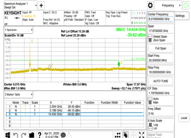
Band41_80MHz_DFT_s_OFDM_SCS30kHz_BPSK_RB1_1_CH518604_below 18G
