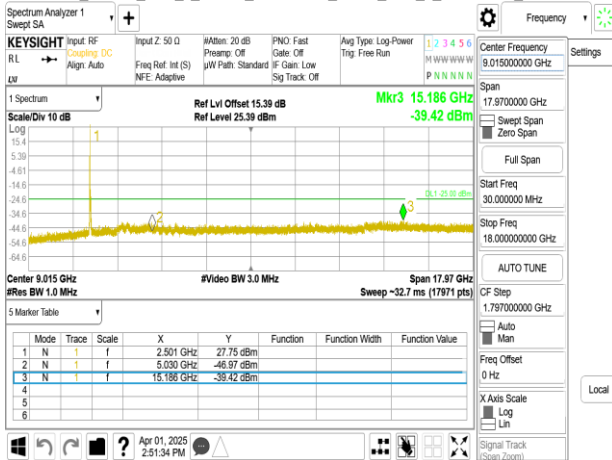
Band41_30MHz_DFT_s_OFDM_SCS15kHz_BPSK_RB1_1_CH518604_below 18G
