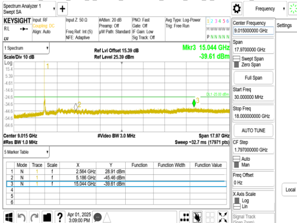
Band41_60MHz_DFT_s_OFDM_SCS30kHz_BPSK_RB1_1_CH531996_below 18G
