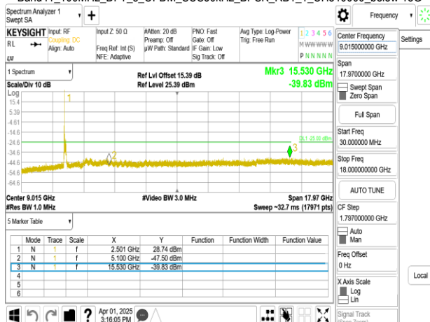
Band41_100MHz_DFT_s_OFDM_SCS30kHz_BPSK_RB1_1_CH518604 below 18G
