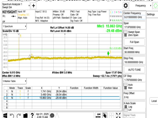
Band66_10MHz_DFT_s_OFDM_SCS30kHz_BPSK_RB1_1_CH355000
