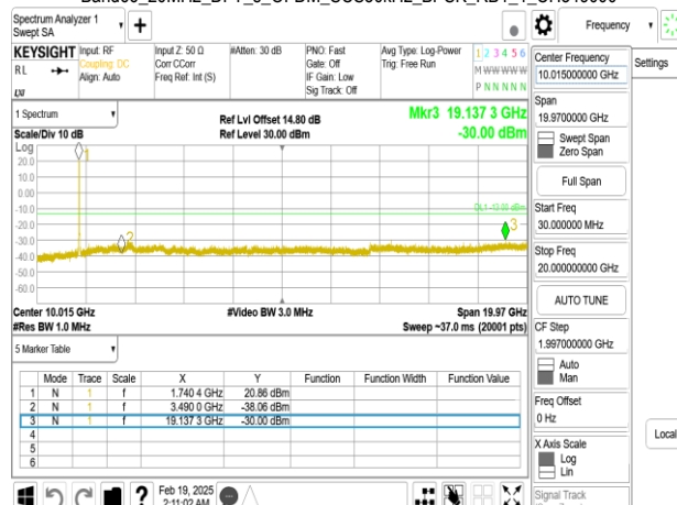
Band66_20MHz_DFT_s_OFDM_SCS30kHz_BPSK_RB1_1_CH349000
