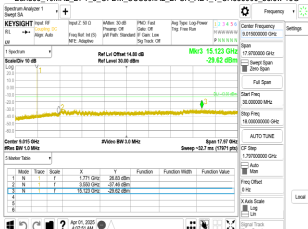
Band66_10MHz_DFT_s_OFDM_SCS30kHz_BPSK_RB1_1_CH355000_below 18G
