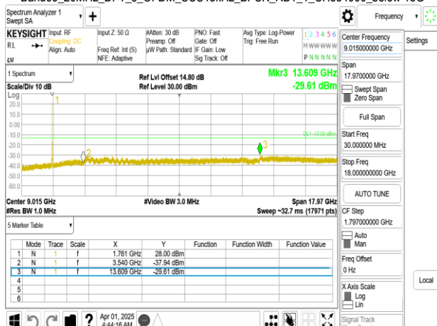
Band66_20MHz_DFT_s_OFDM_SCS15kHz_BPSK_RB1_1_CH354000_below 18G
