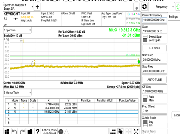
Band66_15MHz_DFT_s_OFDM_SCS15kHz_BPSK_RB1_1_CH349000
