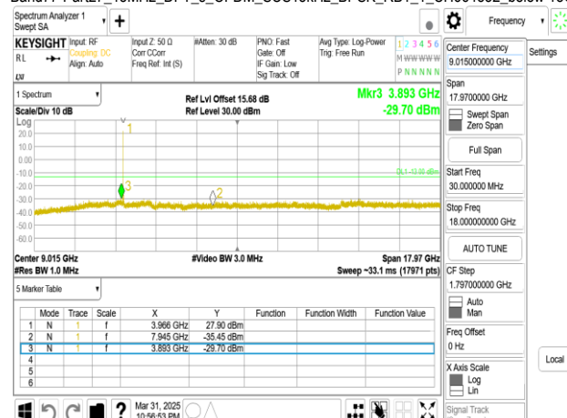
Band77-Part27 15MHz DFT s OFDM SCS15kHz BPSK RB1 1 CH664832 below 18G
