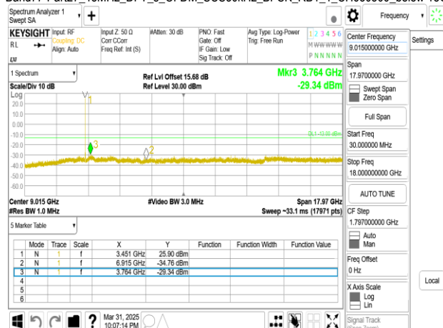
Band77-Part27 15MHz DFT s OFDM SCS30kHz BPSK RB1 1 CH633334 below 18G
