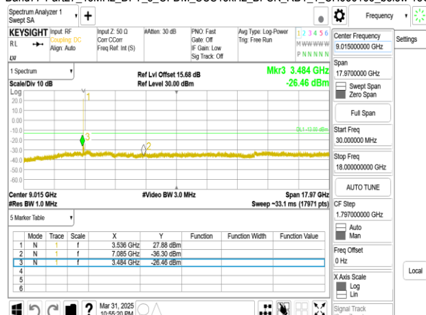
Band77-Part27 15MHz DFT s OFDM SCS15kHz BPSK RB1 1 CH636166 below 18G
