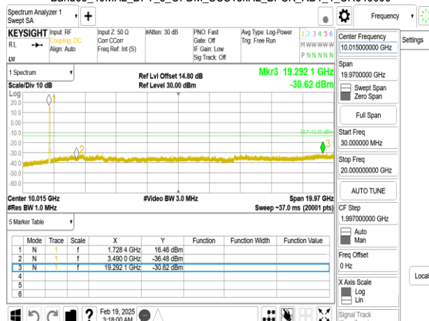
Band66_40MHz_DFT_s_OFDM_SCS15kHz_BPSK_RB1_1_CH349000
