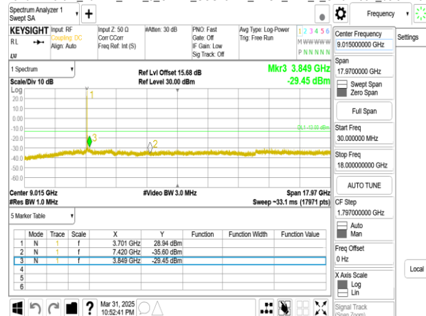
Band77-Part27_20MHz_DFT_s_OFDM_SCS15kHz_BPSK_RB1_1_CH656000_below 18G
