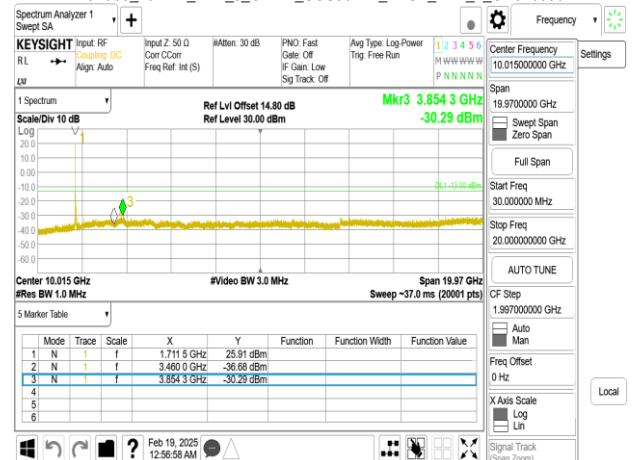
Band66_40MHz_DFT_s_OFDM_SCS30kHz_BPSK_RB1_1_CH346000_below 18G
