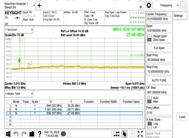
Band71_15MHz_DFT_s_OFDM_SCS30kHz_BPSK_RB1_1_CH138100
