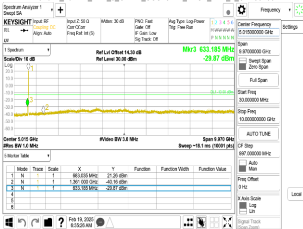
Band71_10MHz_DFT_s_OFDM_SCS15kHz_BPSK_RB1_1.CH136600
