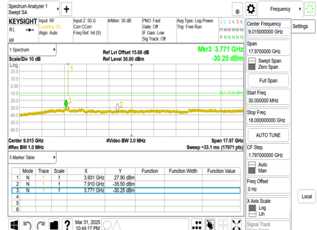
Band77-Part27_50MHz_DFT_s_OFDM_SCS15kHz_BPSK_RB1_1_CH636666_below 18G
