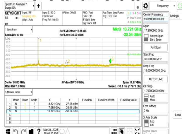
Band77-Part27_40MHz_DFT_s_OFDM_SCS15kHz_BPSK_RB1_1_CH664000_below 18G
