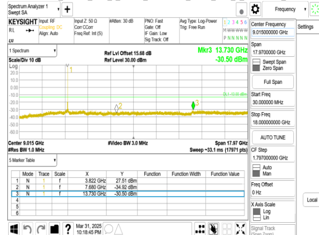
Band77-Part27_40MHz_DFT_s_OFDM_SCS30kHz_BPSK_RB1_1_CH664000_below 18G
