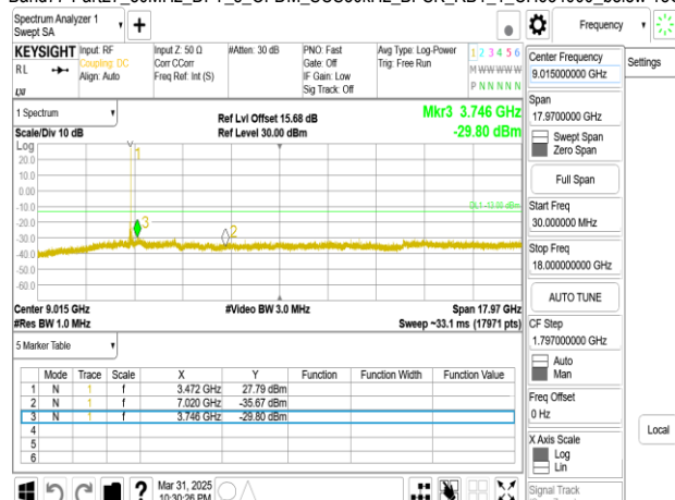
Band77-Part27 80MHz DFT s OFDM SCS30kHz BPSK RB1 1 CH634000 below 18G
