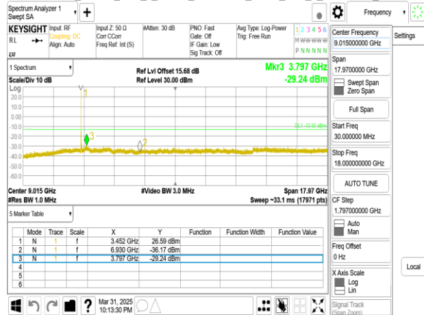
Band77-Part27_30MHz_DFT_s_OFDM_SCS30kHz_BPSK_RB1_1_CH633334_below 18G
