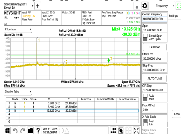
Band77-Part27_90MHz_DFT_s_OFDM_SCS30kHz_BPSK_RB1_1_CH656000_below 18G
