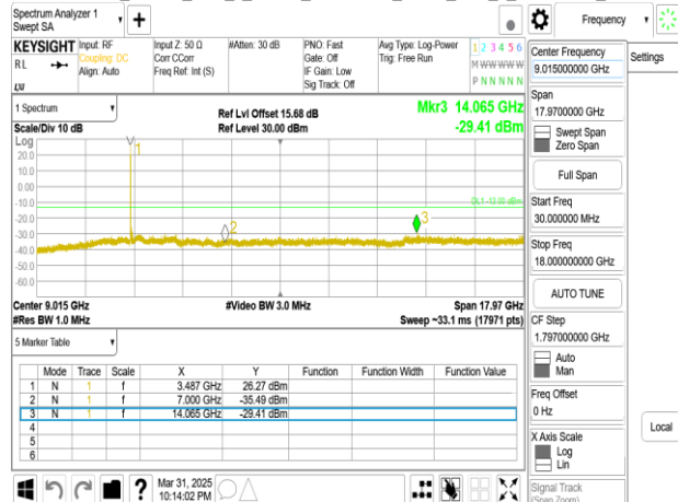
Band77-Part27_30MHz_DFT_s_OFDM_SCS30kHz_BPSK_RB1_1_CH635666_below 18G
