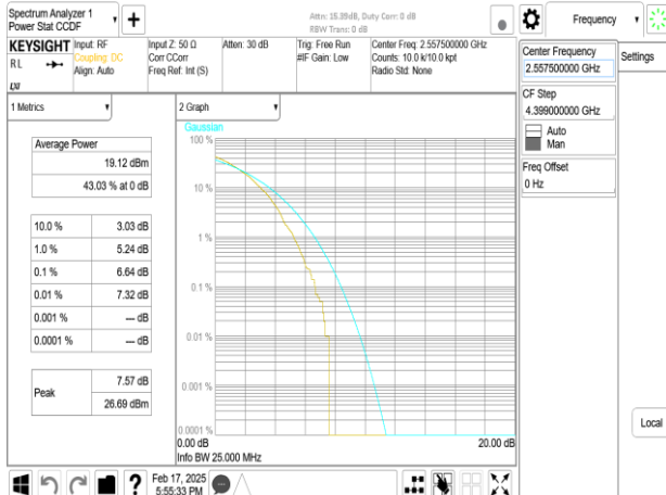
Band7_25MHz_DFT_s_OFDM_SCS30kHz_256QAM_RB64_0_CH511500
