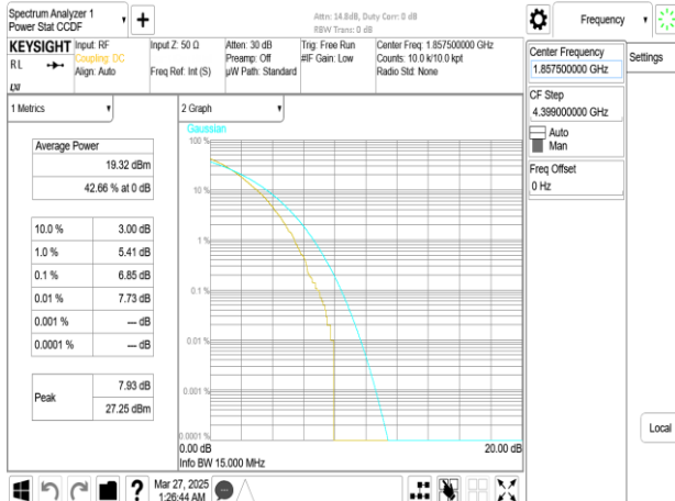
Band25_15MHz_DFT_s_OFDM_SCS15kHz_256QAM_RB75_0_CH371500
