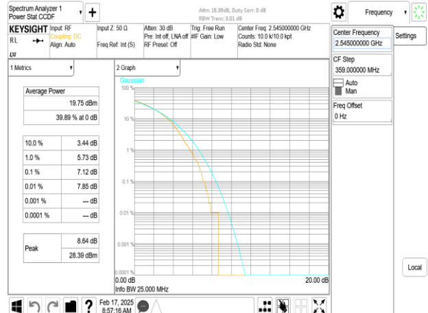
Band7_50MHz_DFT_s_OFDM_SCS15kHz_256QAM_RB270_0_CH509000
