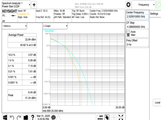
Band41_50MHz_DFT_s_OFDM_SCS15kHz_256QAM_RB270_0_CH505002
