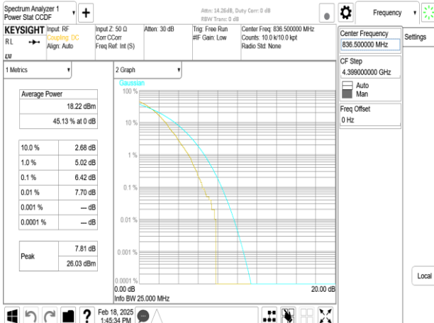
Band26_20MHz_DFT_s_OFDM_SCS30kHz_256QAM_RB50_0_CH167300
