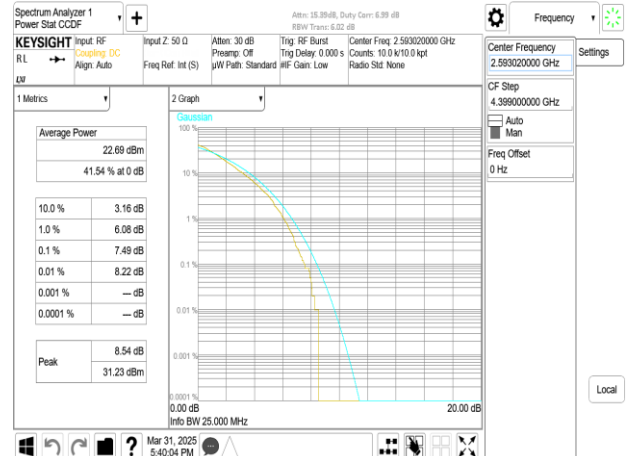
Band41_100MHz_DFT_s_OFDM_SCS30kHz_256QAM_RB270_0_CH518604
