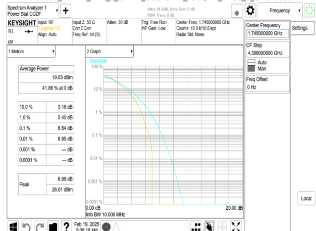
Band66_10MHz_DFT_s_OFDM_SCS15kHz_256QAM_RB50_0_CH349000
