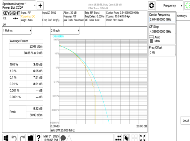
Band41_90MHz_DFT_s_OFDM_SCS30kHz_256QAM_RB243_0_CH528996
