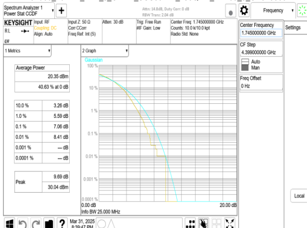
Band66_40MHz_DFT_s_OFDM_SCS30kHz_256QAM_RB100_0_CH349000
