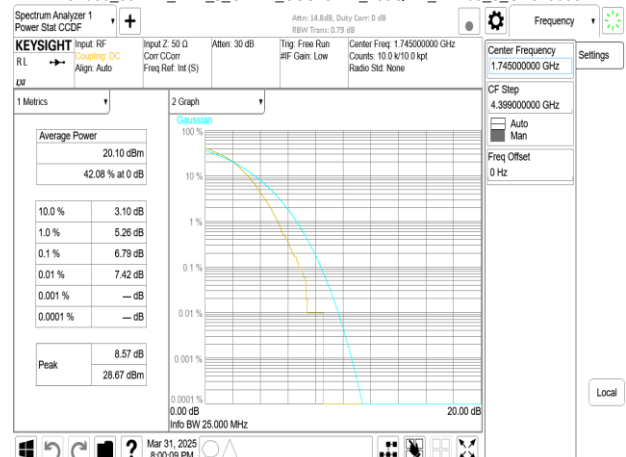
Band66_30MHz_DFT_s_OFDM_SCS15kHz_256QAM_RB160_0_CH349000
