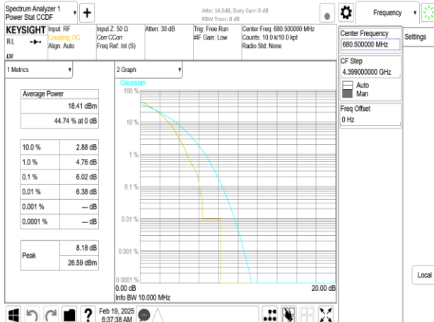
Band71_10MHz_DFT_s_OFDM_SCS15kHz_256QAM_RB50_0_CH136100
