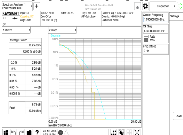
Band66_25MHz_DFT_s_OFDM_SCS30kHz_256QAM_RB64_0_CH349000
