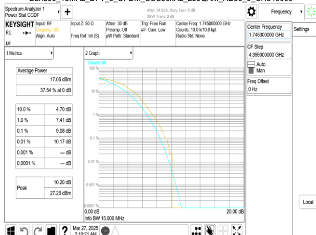
Band66_15MHz_DFT_s_OFDM_SCS30kHz_256QAM_RB36_0_CH349000
