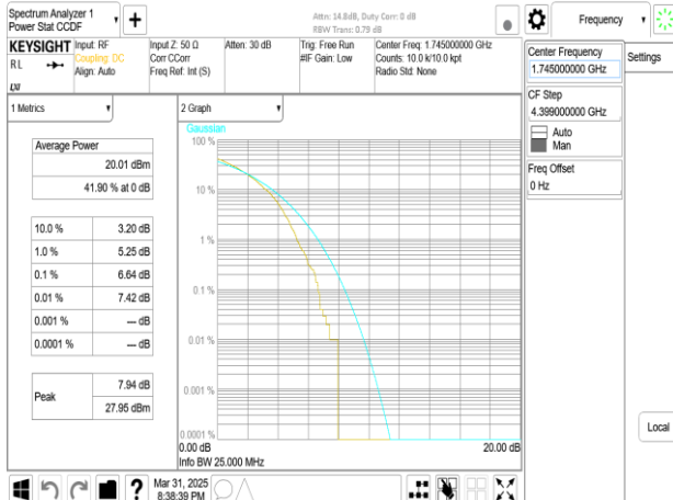
Band66_30MHz_DFT_s_OFDM_SCS30kHz_256QAM_RB75_0_CH349000
