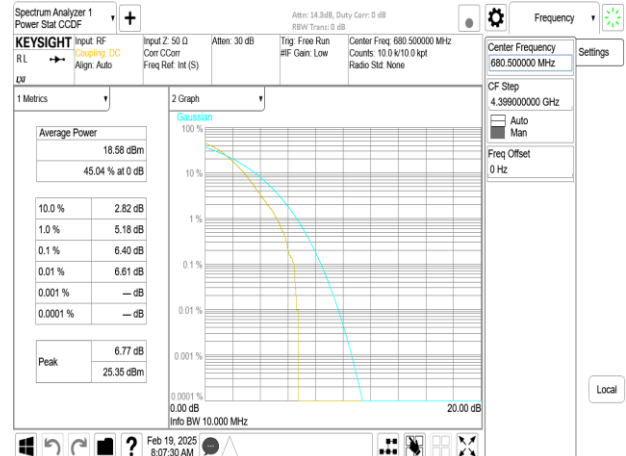
Band71_10MHz_DFT_s_OFDM_SCS30kHz_256QAM_RB24_0_CH136100
