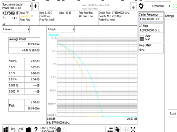
Band66_5MHz_DFT_s_OFDM_SCS15kHz_256QAM_RB25_0_CH349000
