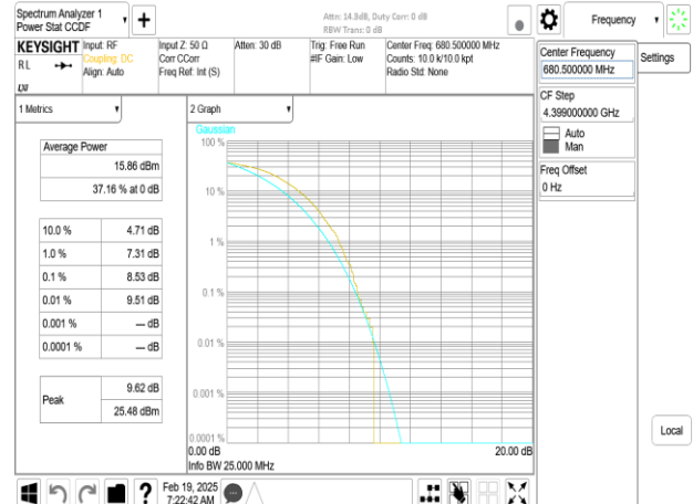
Band71_20MHz_DFT_s_OFDM_SCS30kHz_256QAM_RB50_0_CH136100
