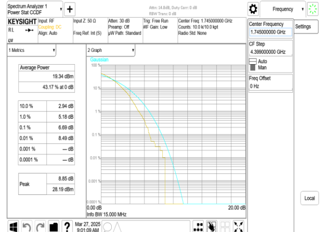
Band66_15MHz_DFT_s_OFDM_SCS15kHz_256QAM_RB75_0_CH349000
