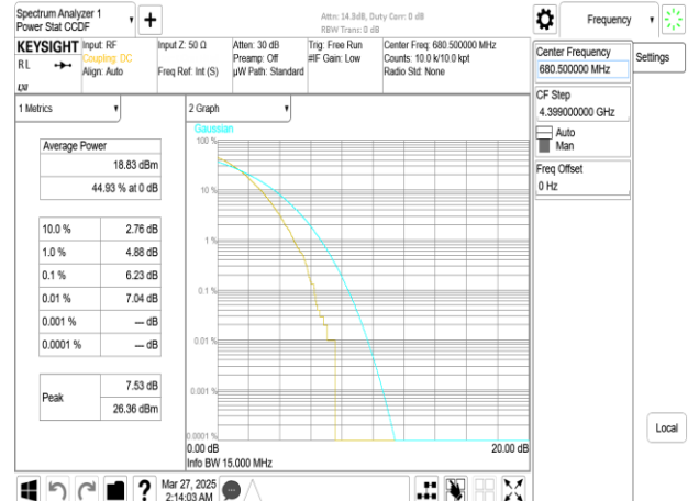
Band71_15MHz_DFT_s_OFDM_SCS30kHz_256QAM_RB36_0_CH136100
