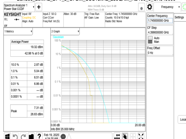
Band66_20MHz_DFT_s_OFDM_SCS15kHz_256QAM_RB100_0_CH349000
