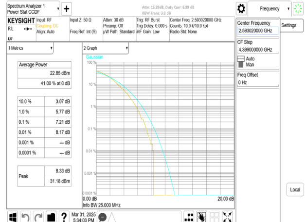
Band41_60MHz_DFT_s_OFDM_SCS30kHz_256QAM_RB162_0_CH518604
