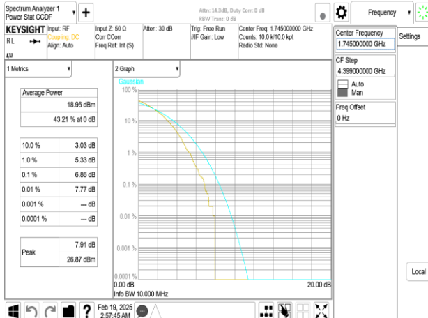
Band66_10MHz_DFT_s_OFDM_SCS30kHz_256QAM_RB24_0_CH349000
