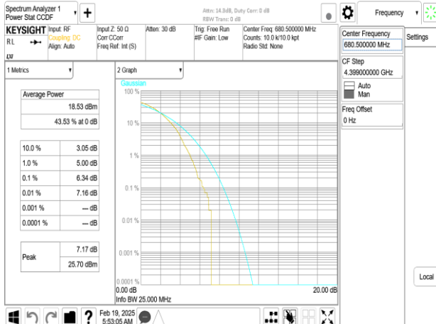
Band71_20MHz_DFT_s_OFDM_SCS15kHz_256QAM_RB100_0_CH136100
