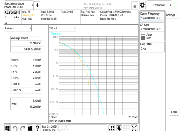
Band66_40MHz_DFT_s_OFDM_SCS15kHz_256QAM_RB216_0_CH349000
