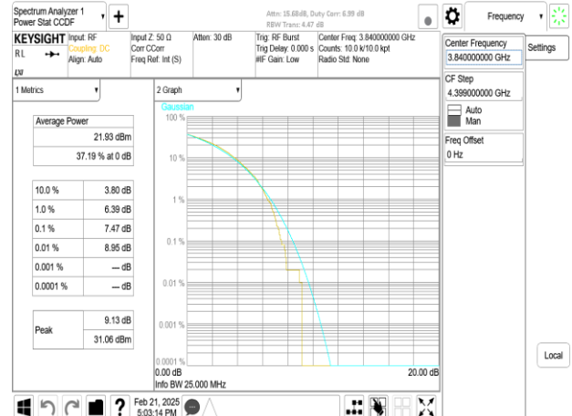
Band77-Part27_70MHz_DFT_s_OFDM_SCS30kHz_256QAM_RB180_0_CH656000
