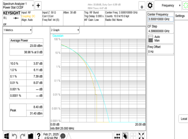
Band77-Part27_70MHz_DFT_s_OFDM_SCS30kHz_256QAM_RB180_0_CH63334
