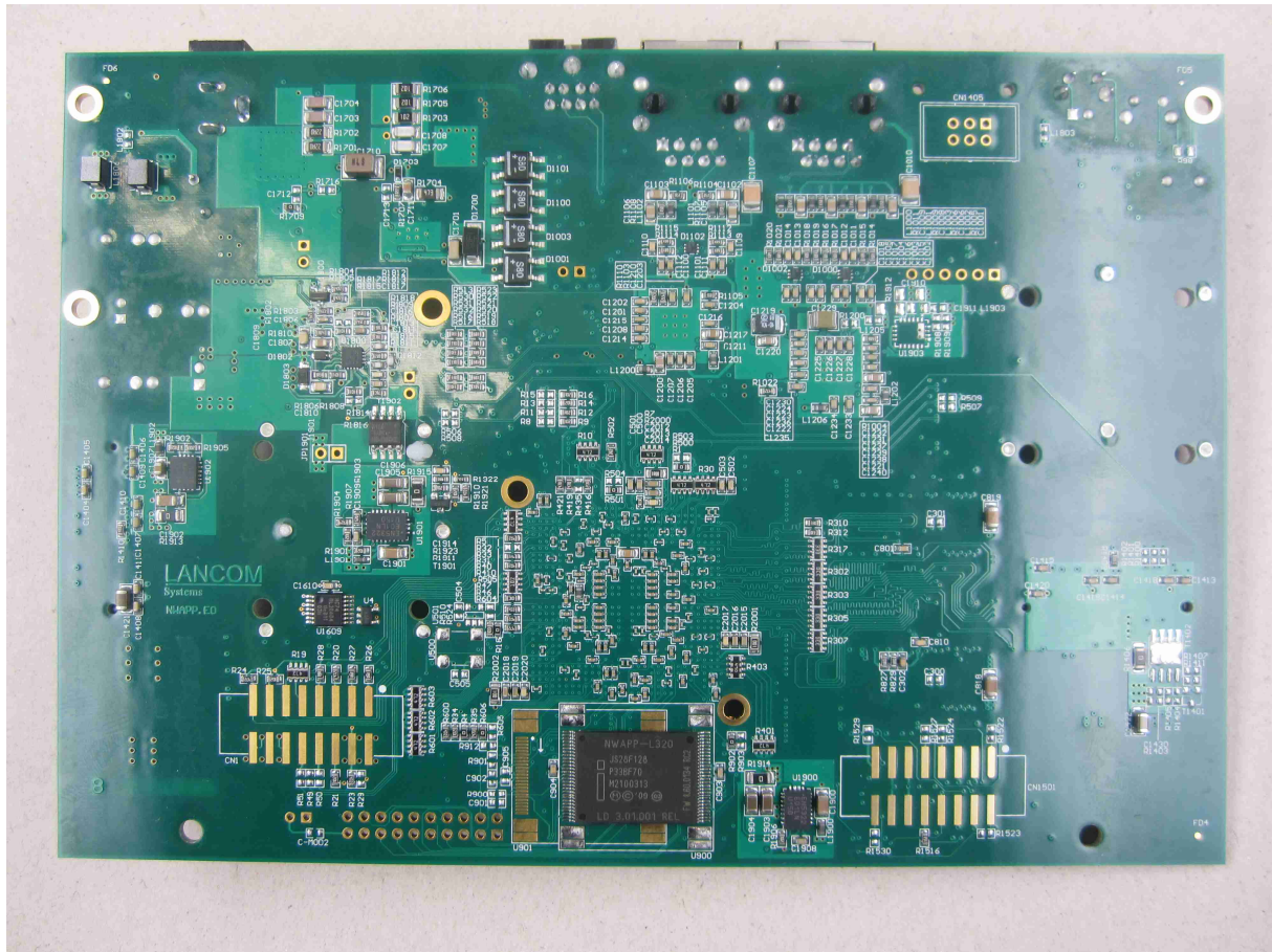
122165_11.JPG: EUT, main PCB, bottom view
