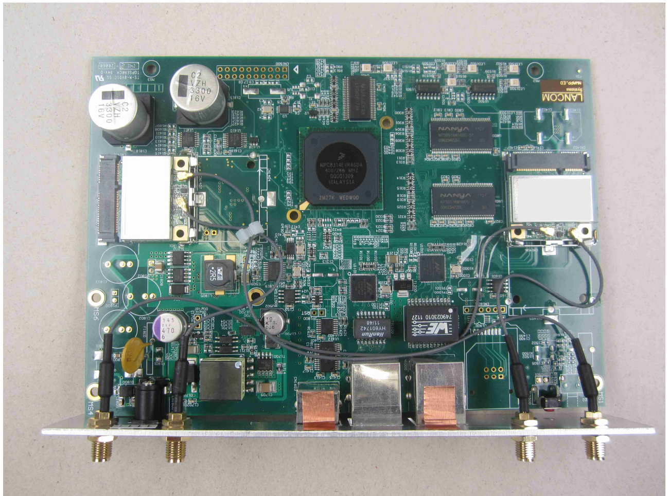
122165_08.JPG: EUT - internal, top view
