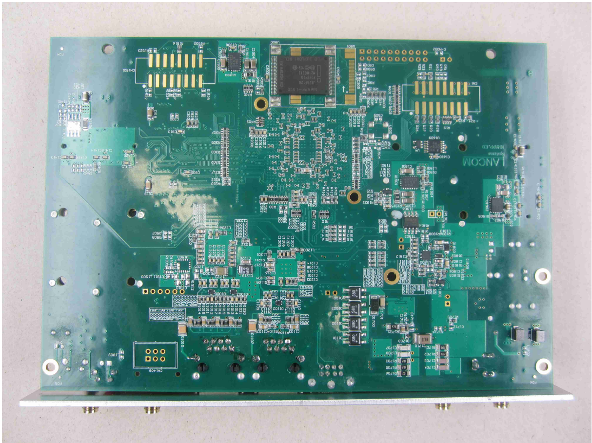
122165_09.JPG: EUT - internal, top view
