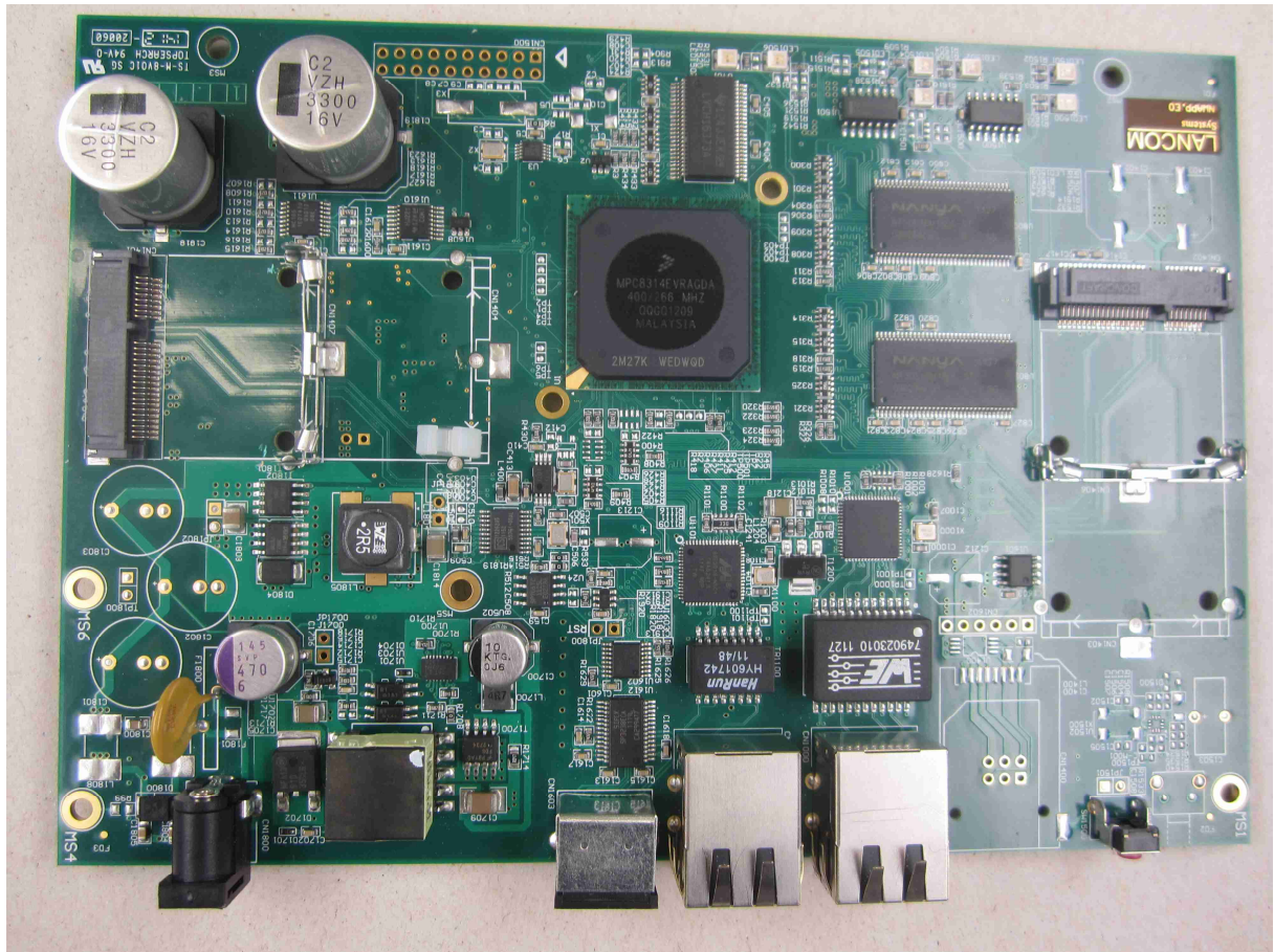
122165_10.JPG: EUT, main PCB, top view
