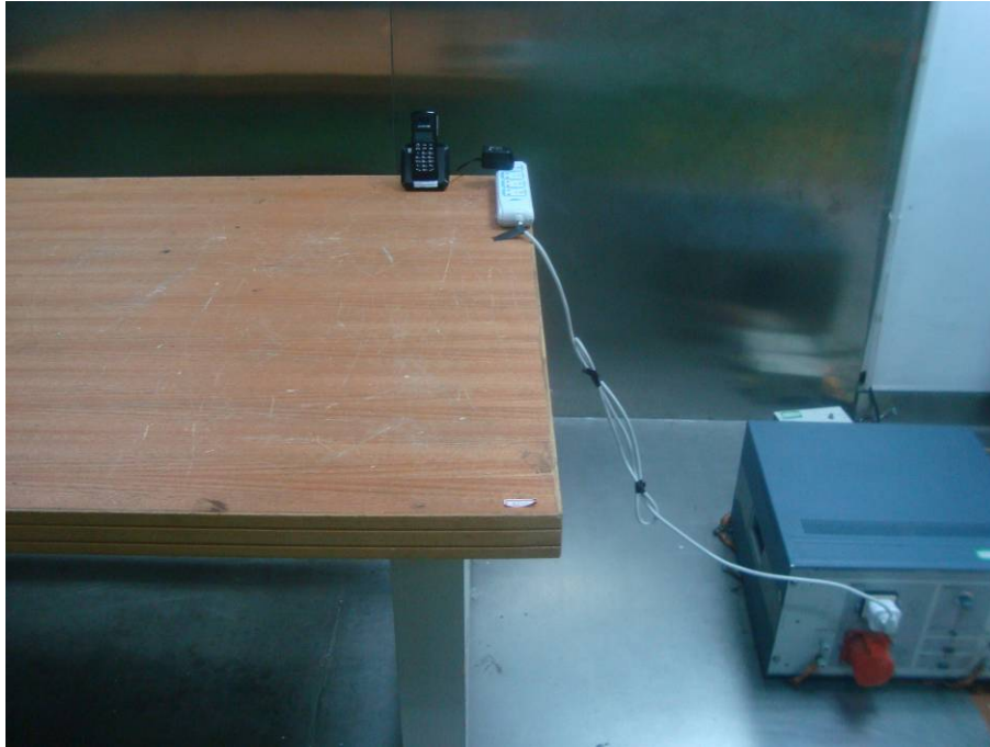
Conducted Emissions - Rear View for charging mode (model 31331)
