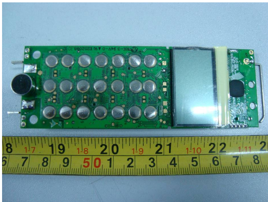
EUT – Main Board Top View (model 31331)
