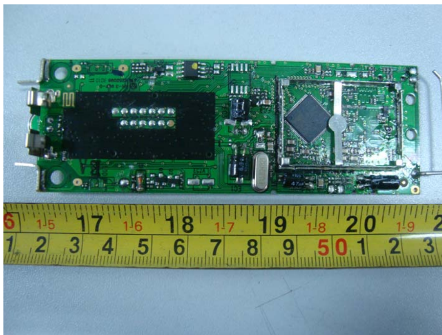
EUT – Main Board Bottom Shielding off View (model 31130)
