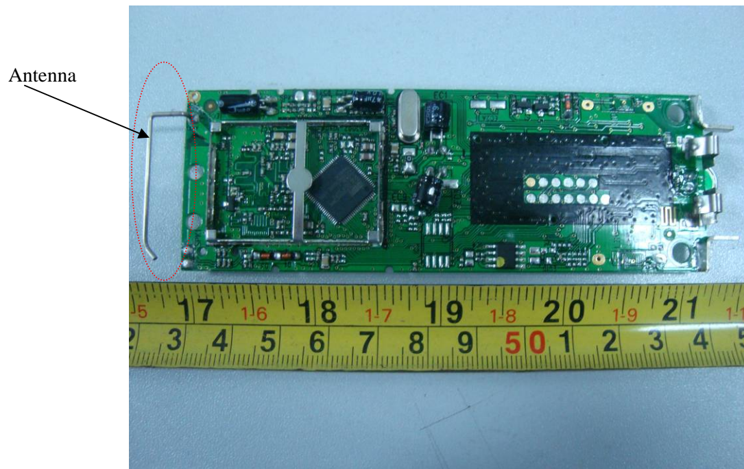
EUT – Main Board Top Shielding off View (model 31331)
