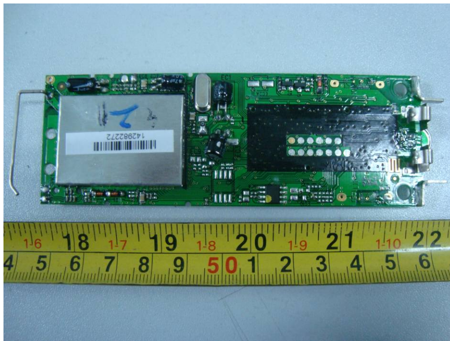
EUT – Main Board Top Shielding off View (model 31331)
