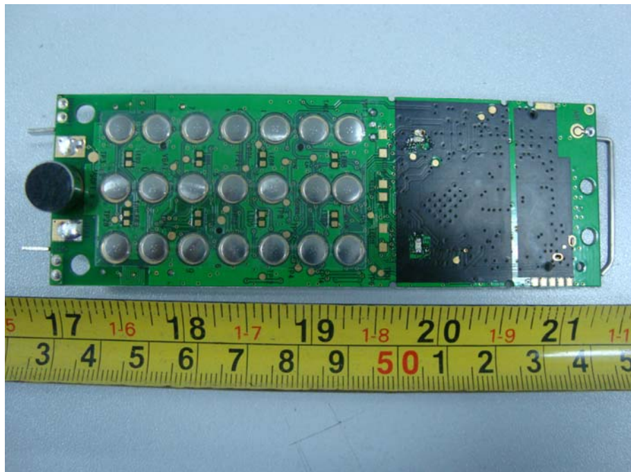
EUT – Main Board Top View (model 31130)
