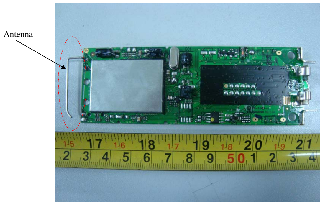
EUT – Main Board Bottom View (model 31130)
