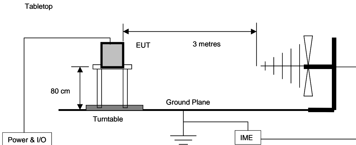
Figure 4 - Radiated Emissions for Tabletop Equipment
