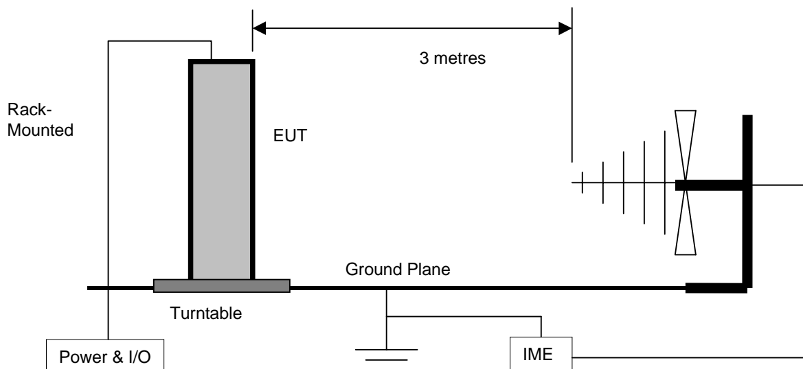
Figure 3 - Radiated Emissions for Rack-Mounted Equipment
