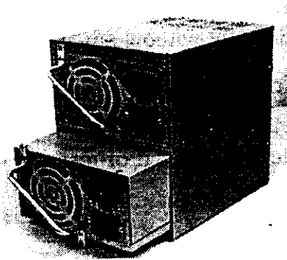
Figure 3.1 Rear Panel of the RPS-500 Including Two PVR-240G-DA Hot-Swap Boxes
