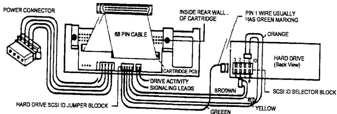
Figure 1.3 Mobile Rack Cabling Connections
