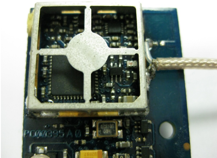
Close Up of RF Section, View #3
